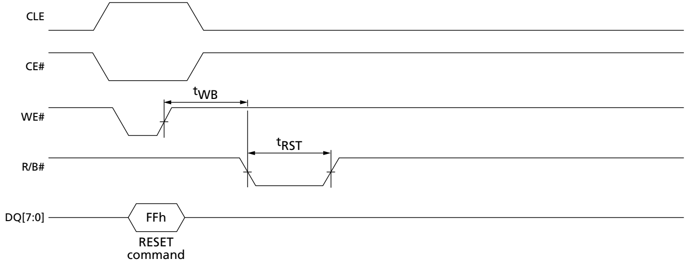
Figure 52: RESET Operation
