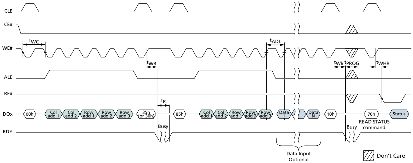
Figure 67: COPYBACK
