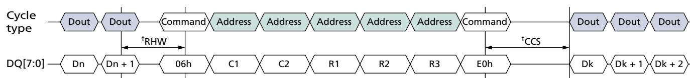
Figure 27: CHANGE READ COLUMN ENHANCED (06h-E0h) Operation
