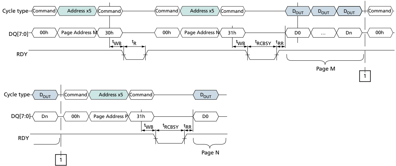
Figure 32: READ PAGE CACHE RANDOM (00h-31h) Operation
