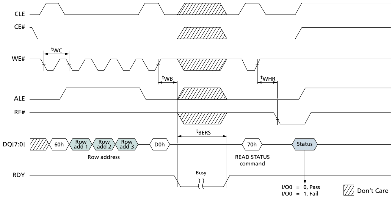
Figure 68: ERASE BLOCK Operation
