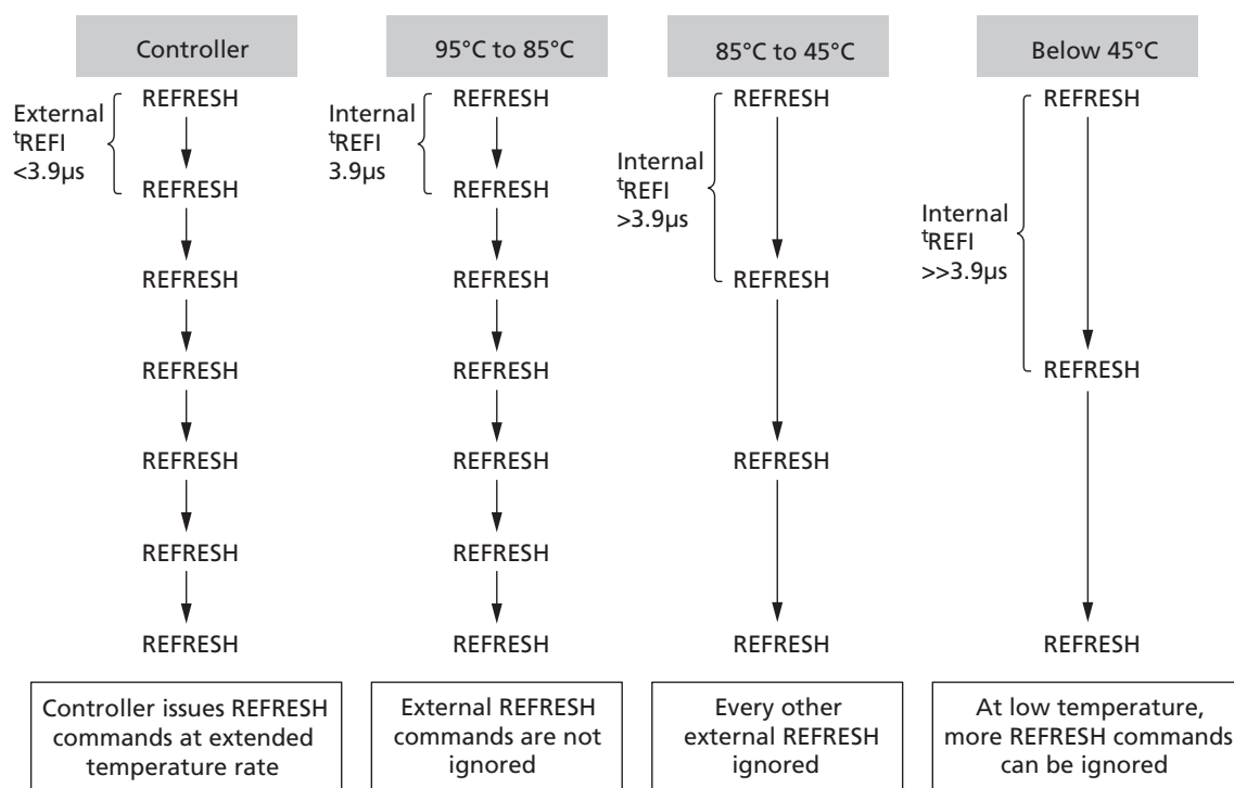
Figure 80: TCR Mode Example 1
