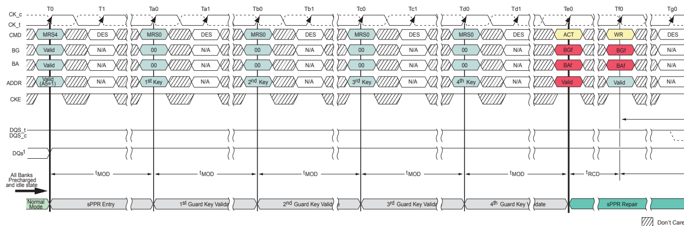
Figure 73: sPPR – Entry
