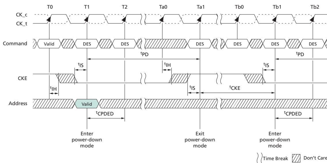
Figure 96: Power-Down Entry/Exit Clarifications – Case 1
