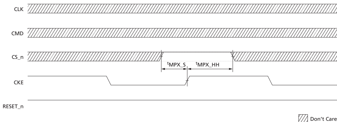
Figure 43: Maintaining Maximum Power-Saving Mode with CKE Transition
