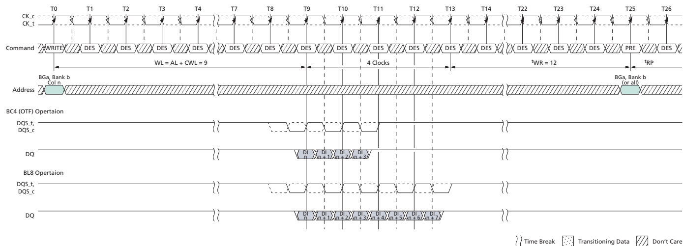
Figure 183: WRITE (BL8/BC4-OTF) to PRECHARGE with 1t_{CK} Preamble
