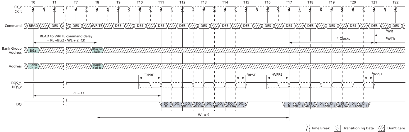
Figure 136: READ (BL8) to WRITE (BL8) with 1 t CK Preamble in Same or Different Bank Group
