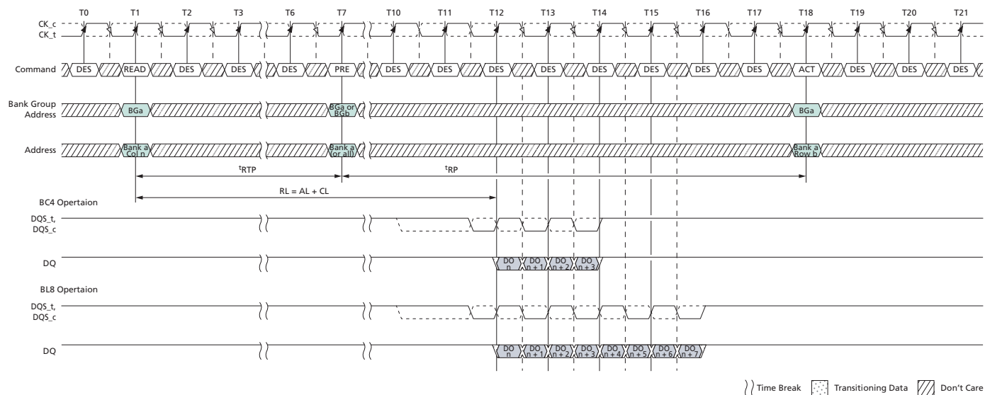
Figure 147: READ to PRECHARGE with 2 t CK Preamble
