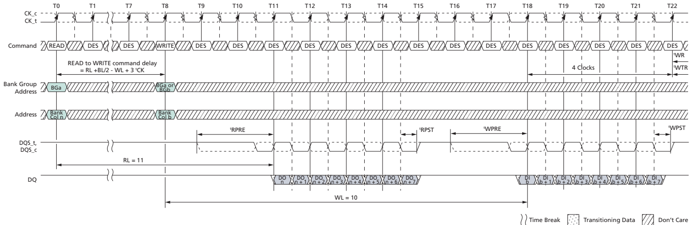
Figure 137: READ (BL8) to WRITE (BL8) with 2 t CK Preamble in Same or Different Bank Group
