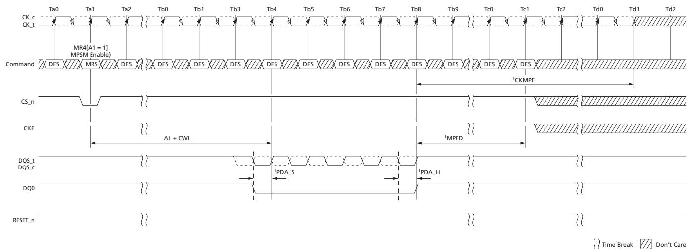
Figure 42: Maximum Power-Saving Mode Entry with PDA
