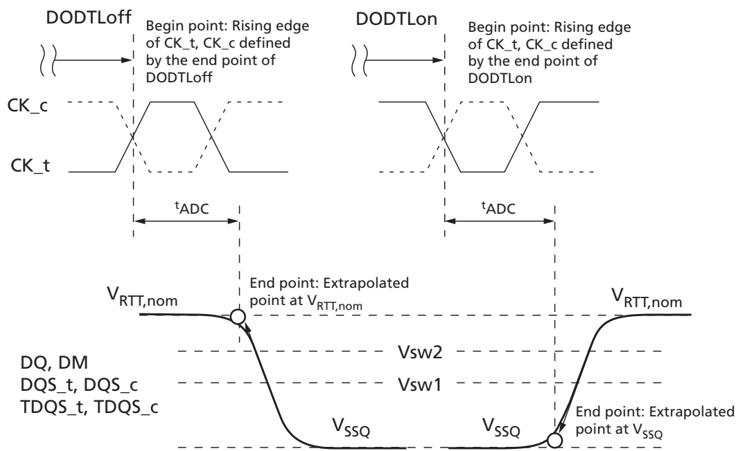
Figure 236: t_{ADC} Definition with Dynamic ODT Control
