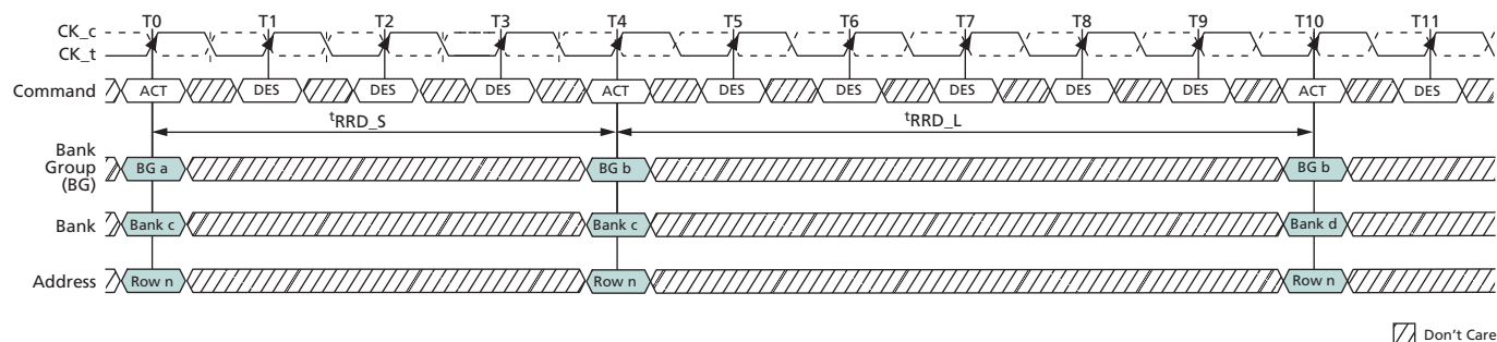
Figure 75: t_{RRD} Timing
