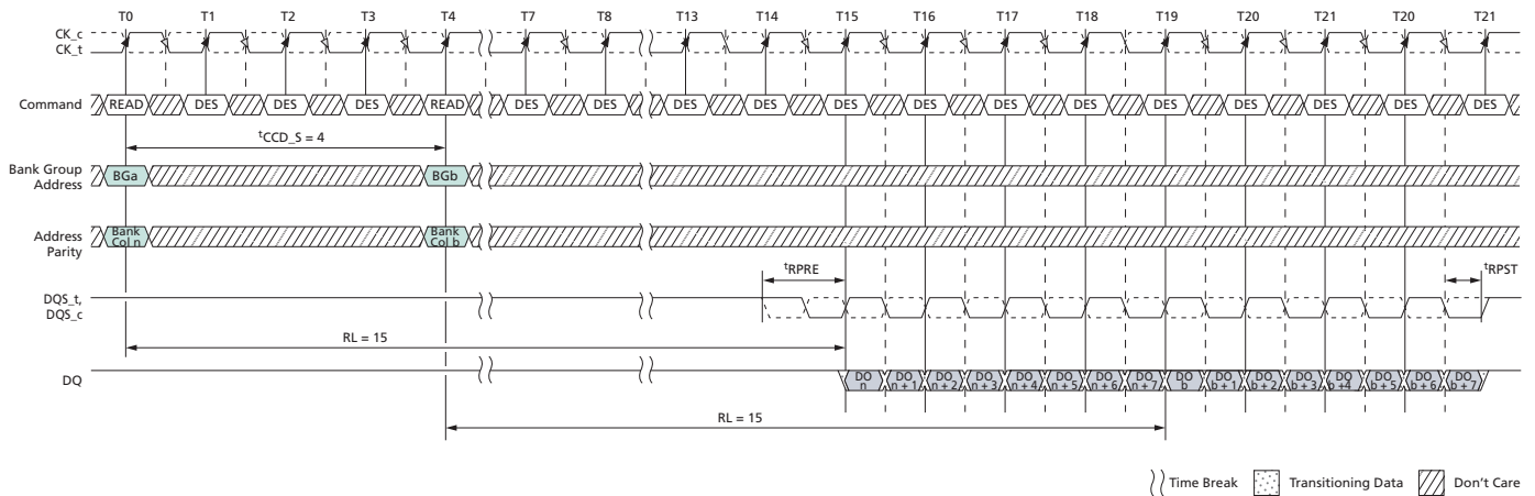
Figure 157: Consecutive READ (BL8) with 1 st CK Preamble and CA Parity in Different Bank Group
