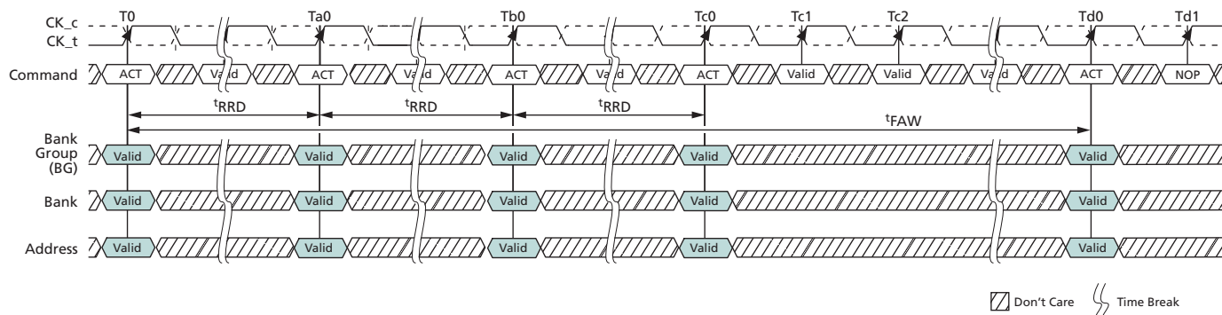
Figure 81: t_{FAW} Timing
