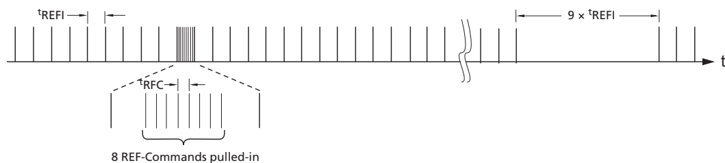
Figure 84: Pulling In REFRESH Commands (Example)
