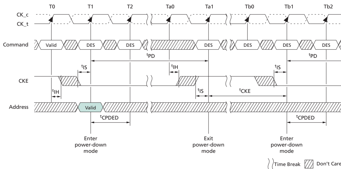
Figure 101: Power-Down Entry/Exit Clarifications – Case 1
