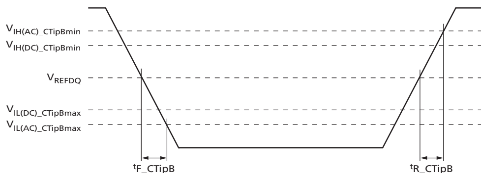
Figure 216: CT Type-B Input Slew Rate Definition
