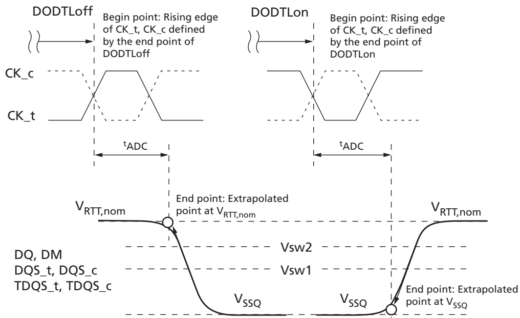
Figure 241: t_{ADC} Definition with Dynamic ODT Control
