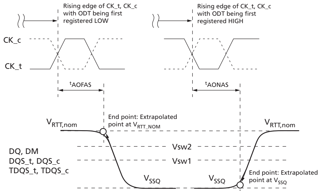
Figure 242: t_{\text{AOFAS}} and t_{\text{AONAS}} Definitions
