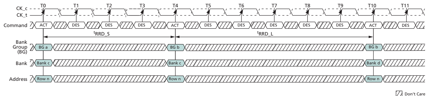
Figure 120: t_{RRD} Timing
