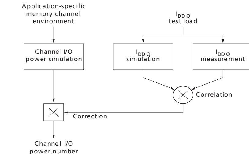
Figure 245: Correlation: Simulated Channel I/O Power to Actual Channel I/O Power
