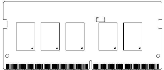
Figure 1: 288-Pin SODIMM (MO-310, R/C D1)
