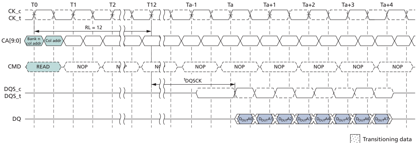
Figure 13: Burst READ – RL = 12, BL = 8, t_{DQSCK} > t_{CK}
