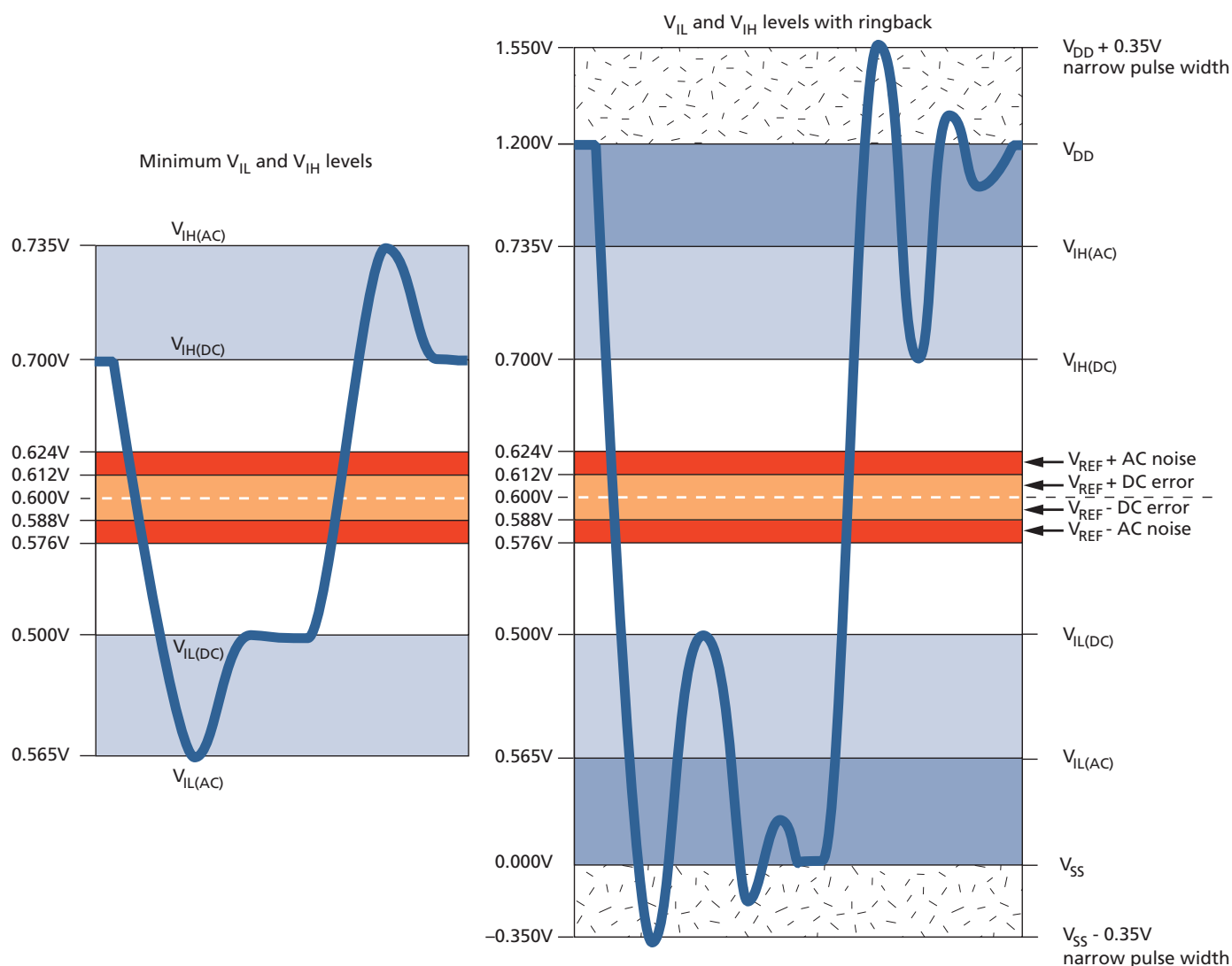
Figure 68: LPDDR3-2133 to LPDDR3-1866 Input Signal
