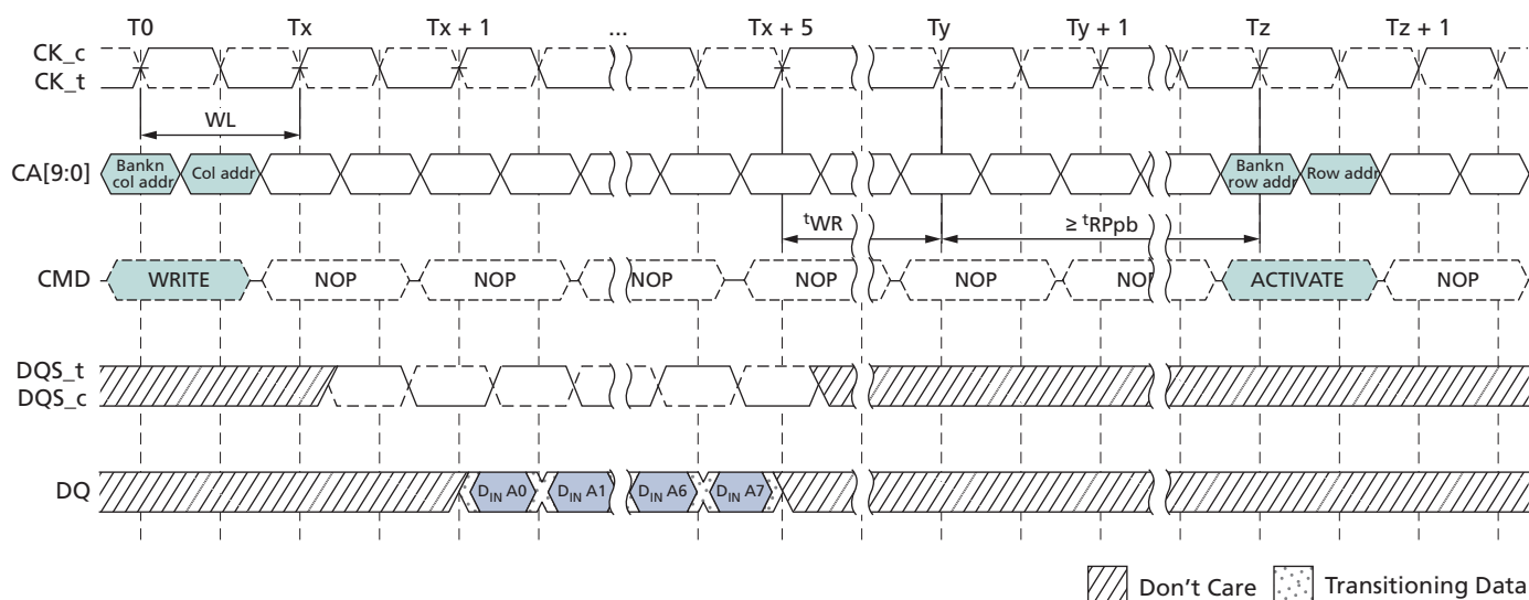
Figure 31: Burst WRITE with Auto Precharge – BL = 8
