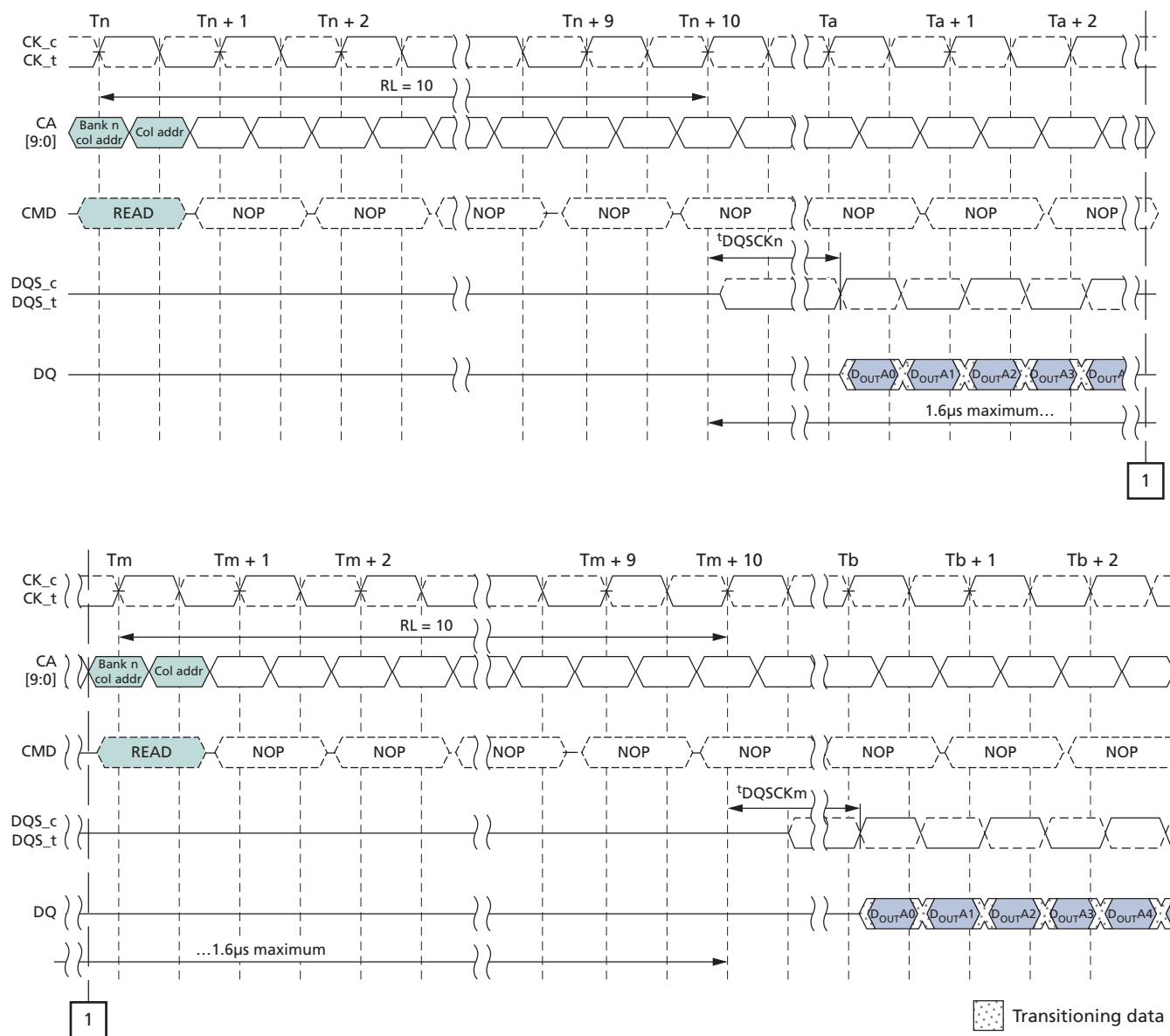
Figure 18: t_{DQSKDM} Timing
