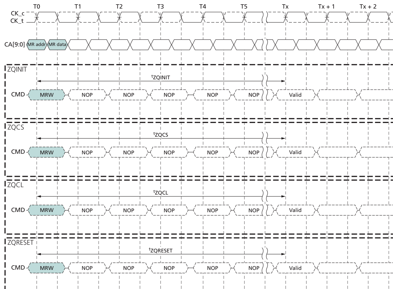
Figure 46: ZQ Timings
