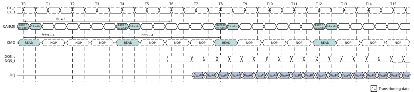
Figure 16: Seamless Burst READ – RL = 6, BL = 8, t_{CCD} = 4
