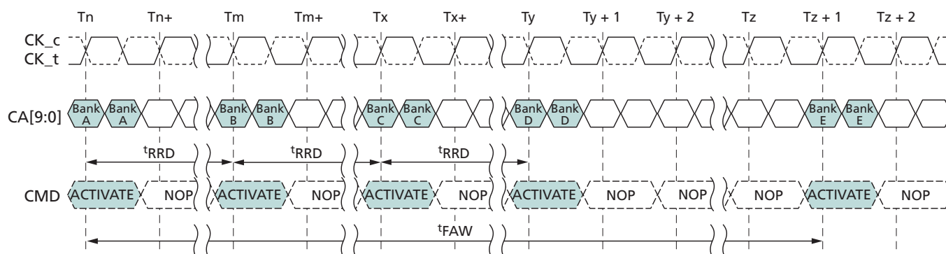
Figure 11: t_{FAW} Timing
