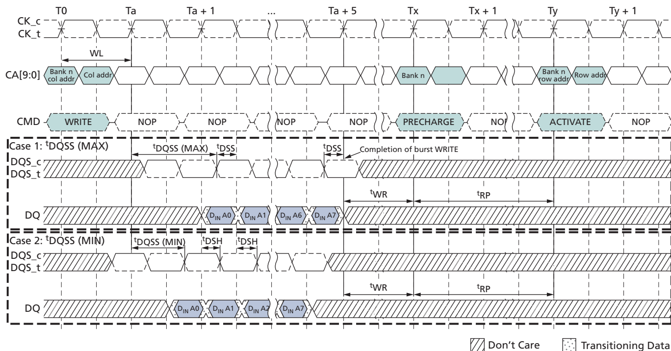
Figure 21: Burst WRITE
