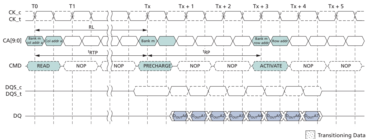
Figure 28: Burst READ Followed by PRECHARGE – BL = 8, RU(t_{RTP}(\text{MIN})/t_{CK}) = 2
