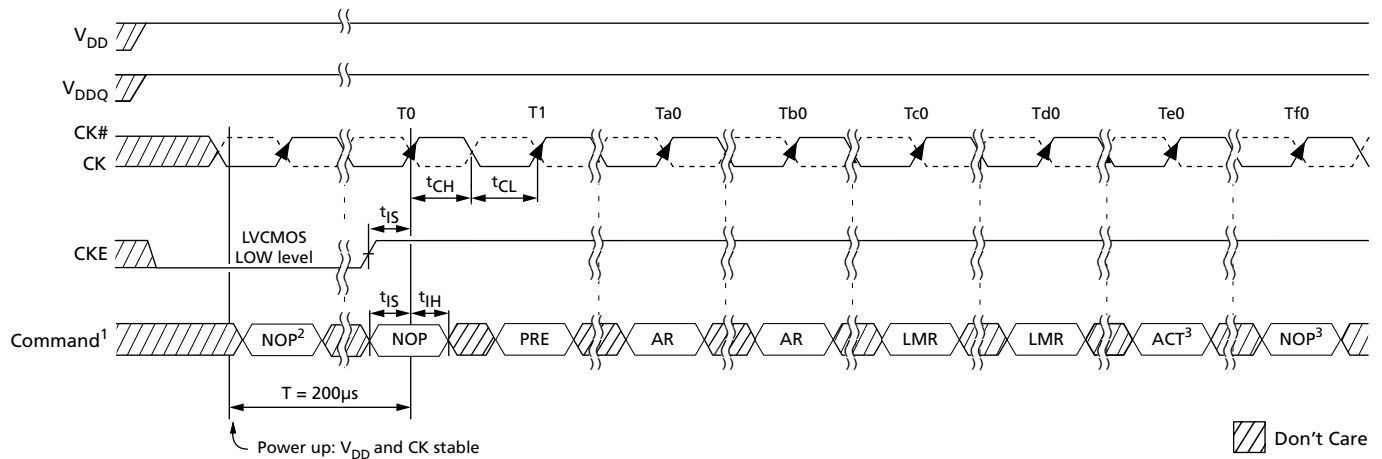
Figure 108: Alternate Initialization with CKE LOW
