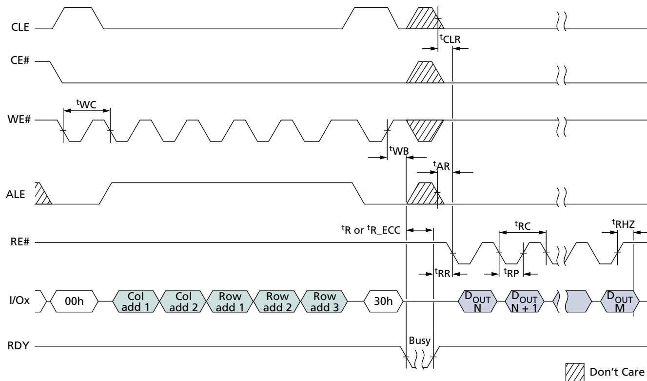
Figure 83: READ PAGE
