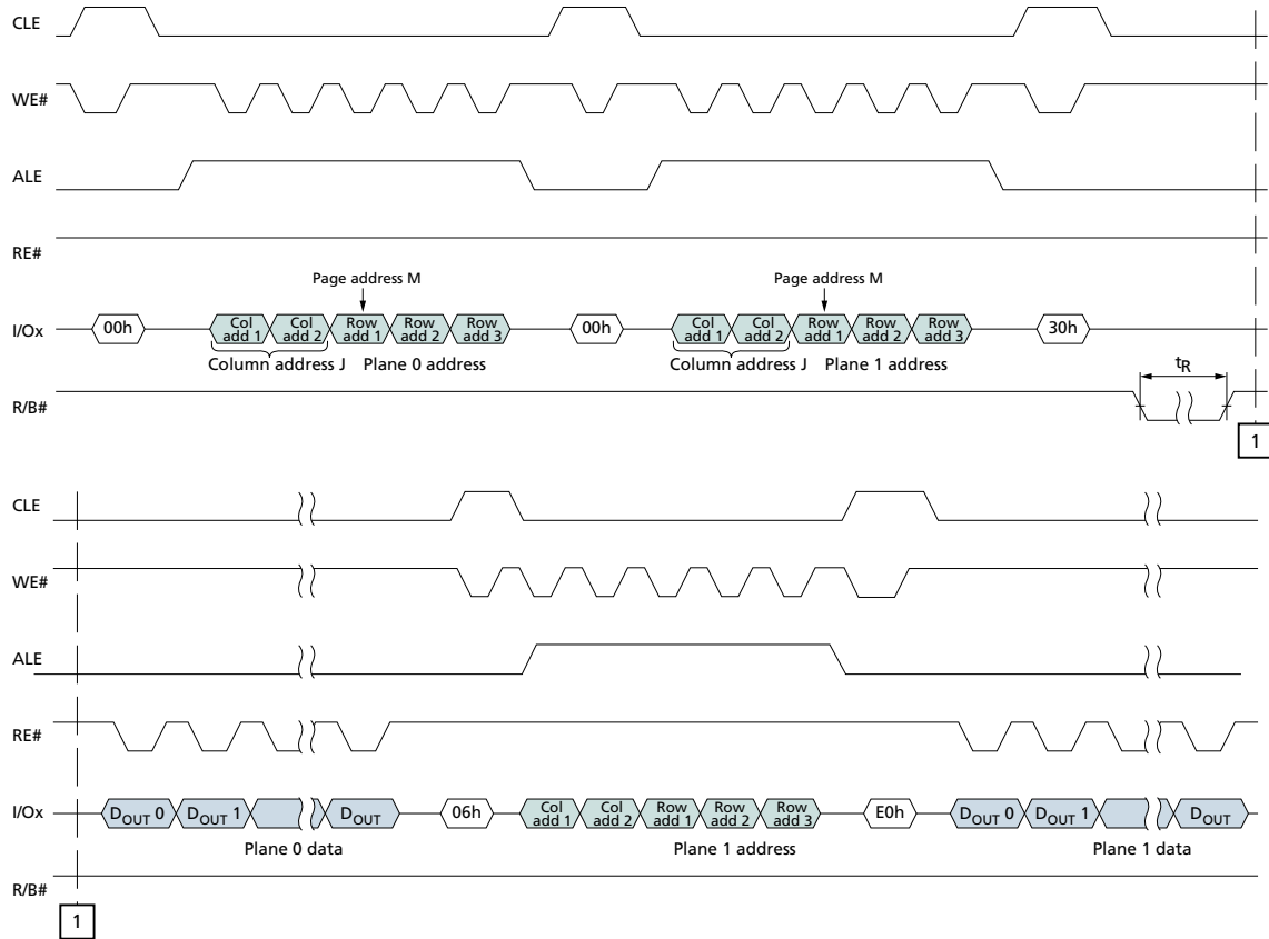
Figure 40: READ PAGE TWO-PLANE (00h-00h-30h) Operation
