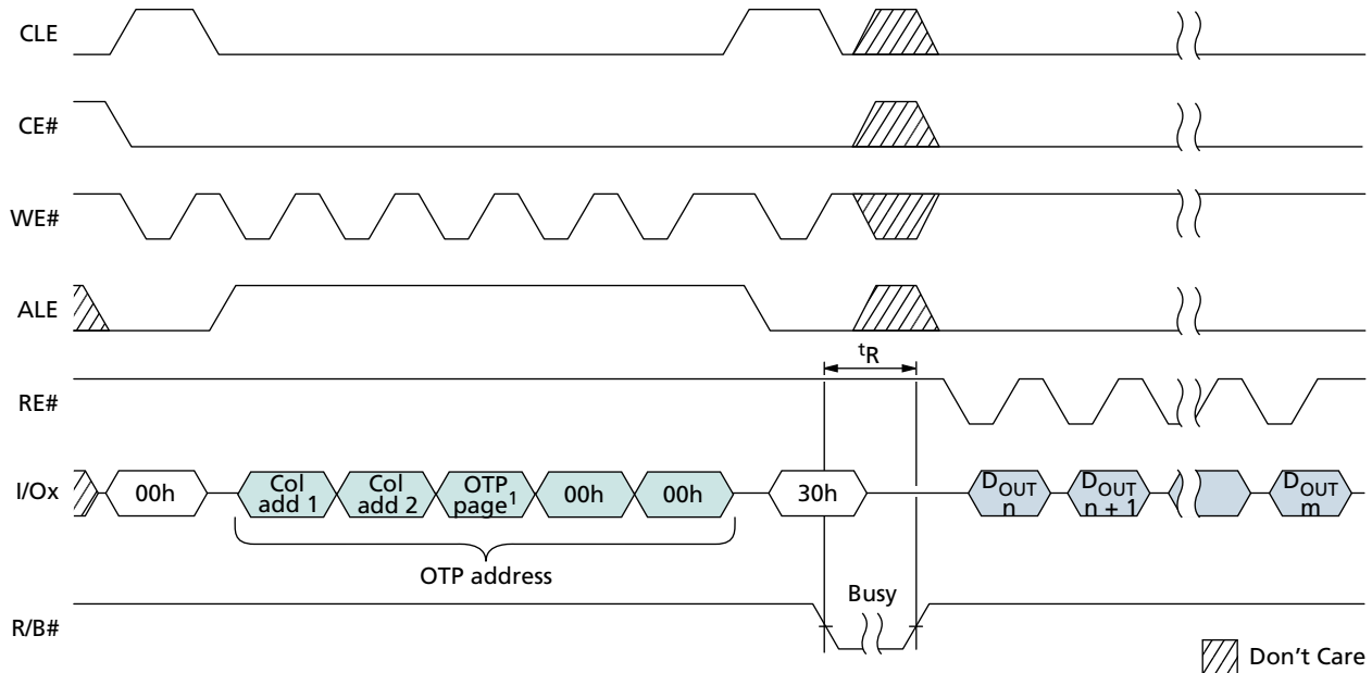
Figure 65: OTP DATA READ
