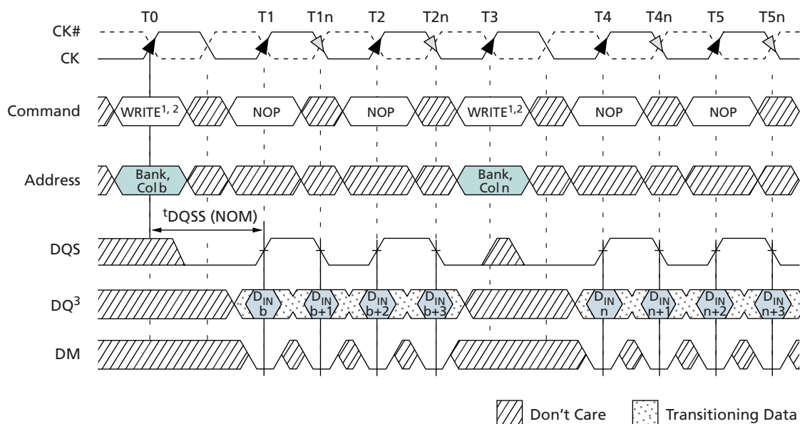
Figure 128: Nonconsecutive WRITE-to-WRITE
