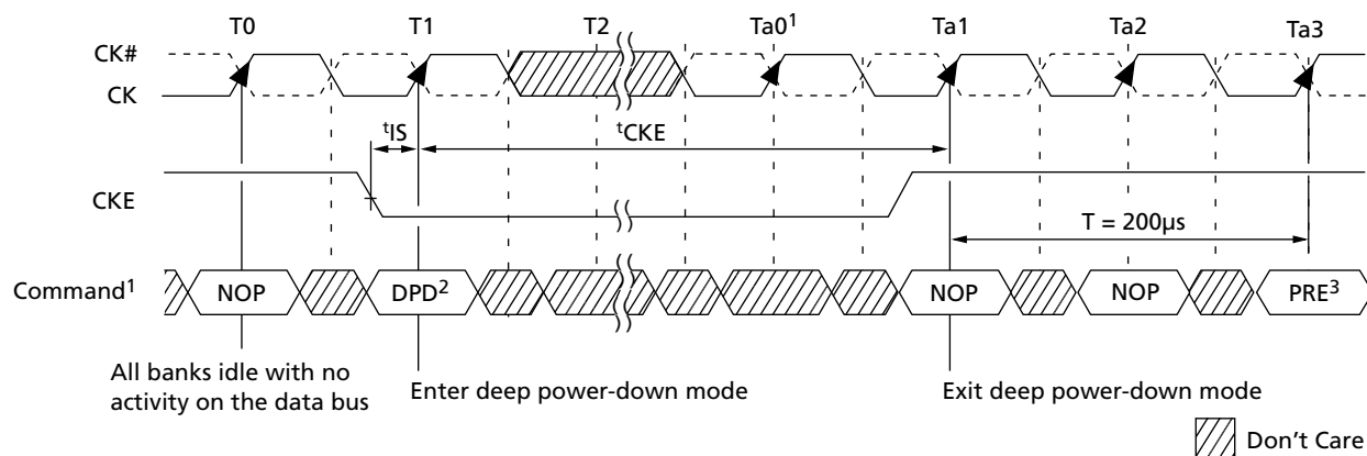
Figure 144: Deep Power-Down Mode
