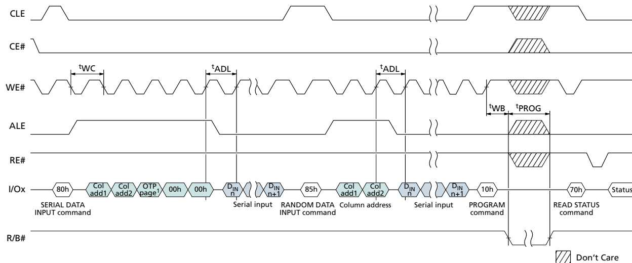
Figure 63: OTP DATA PROGRAM Operation with RANDOM DATA INPUT (After Entering OTP Operation Mode)
