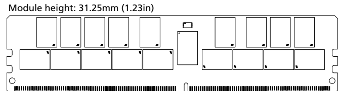
Figure 1: 288-Pin LRDIMM (MO-309, R/C-E2)
