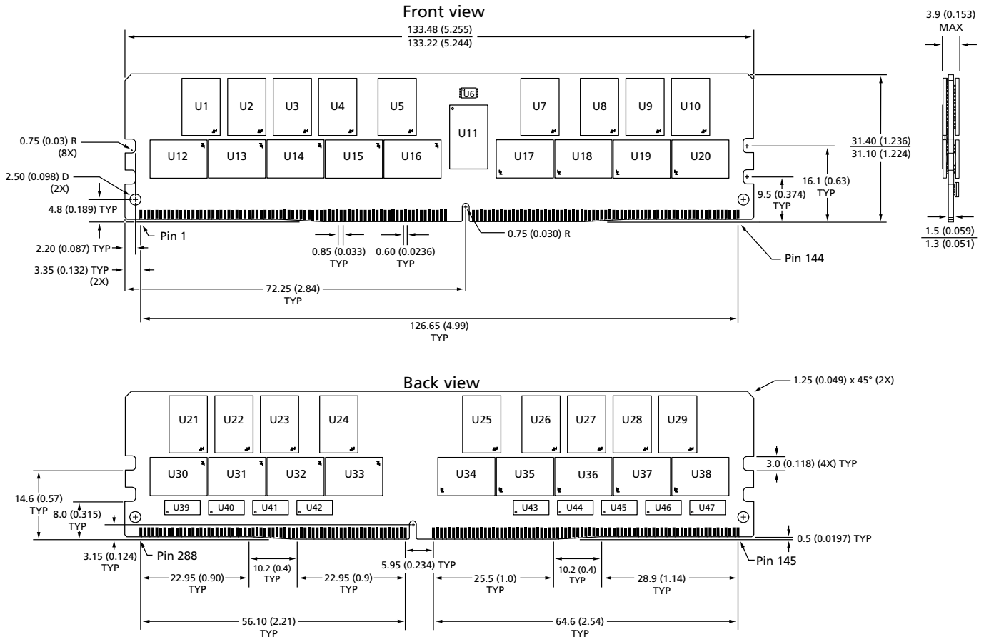
Figure 3: 288-Pin DDR4 LRDIMM
