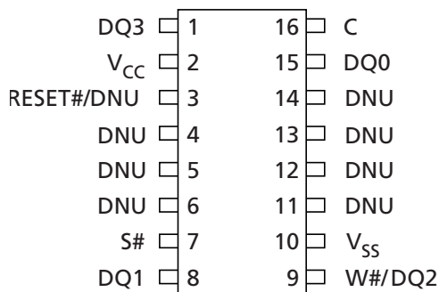
Figure 8: 16-Pin, Plastic Small Outline – SO16 (Top View)
