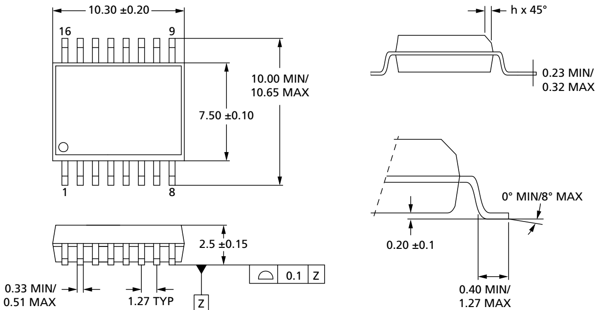
Figure 13: 16-Pin SOP2 – 300 mil Body Width
