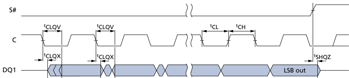
Figure 55: Output Timing
