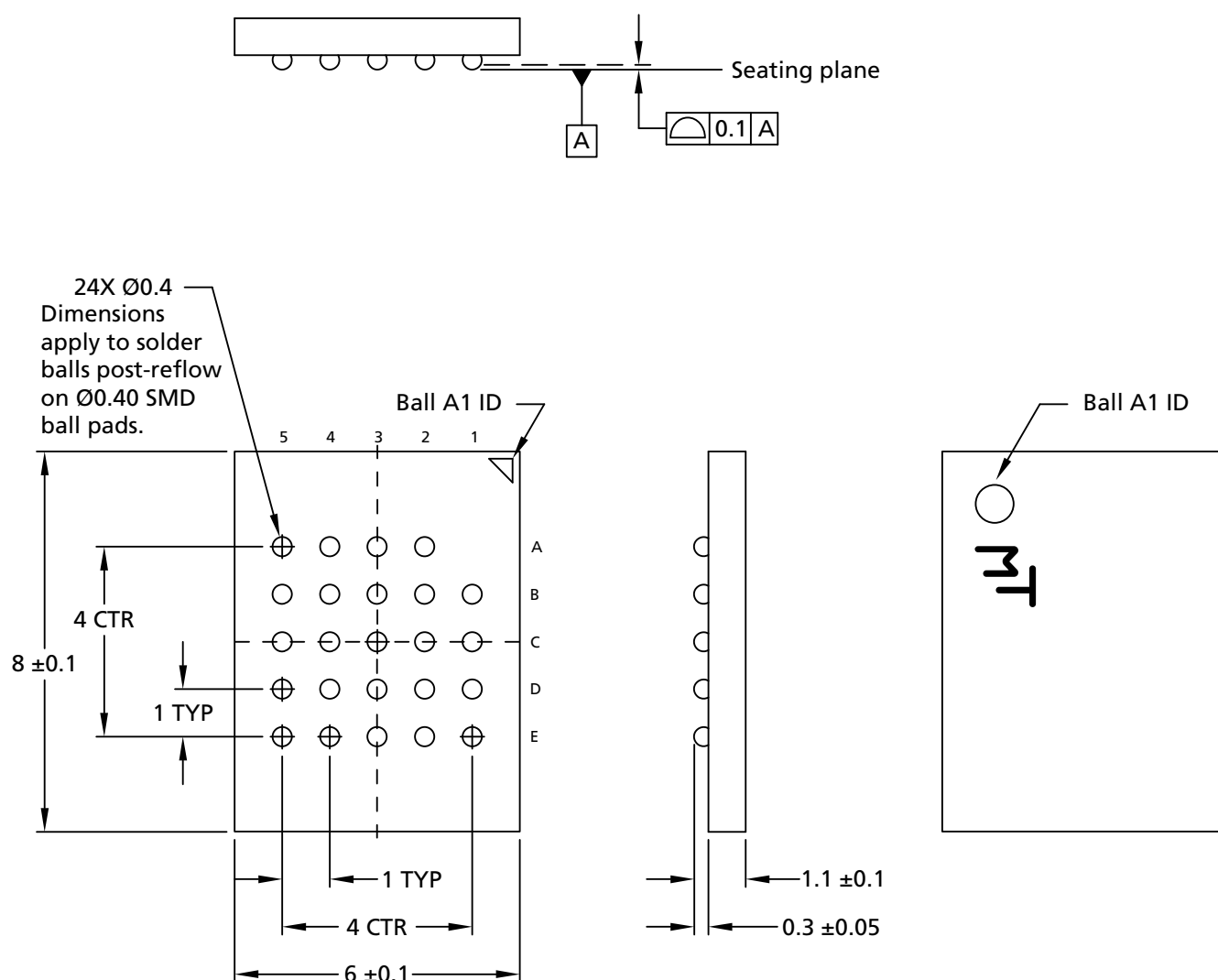
Figure 9: 24-Ball T-PBGA (5 × 5 ball grid array) – 6mm × 8mm
