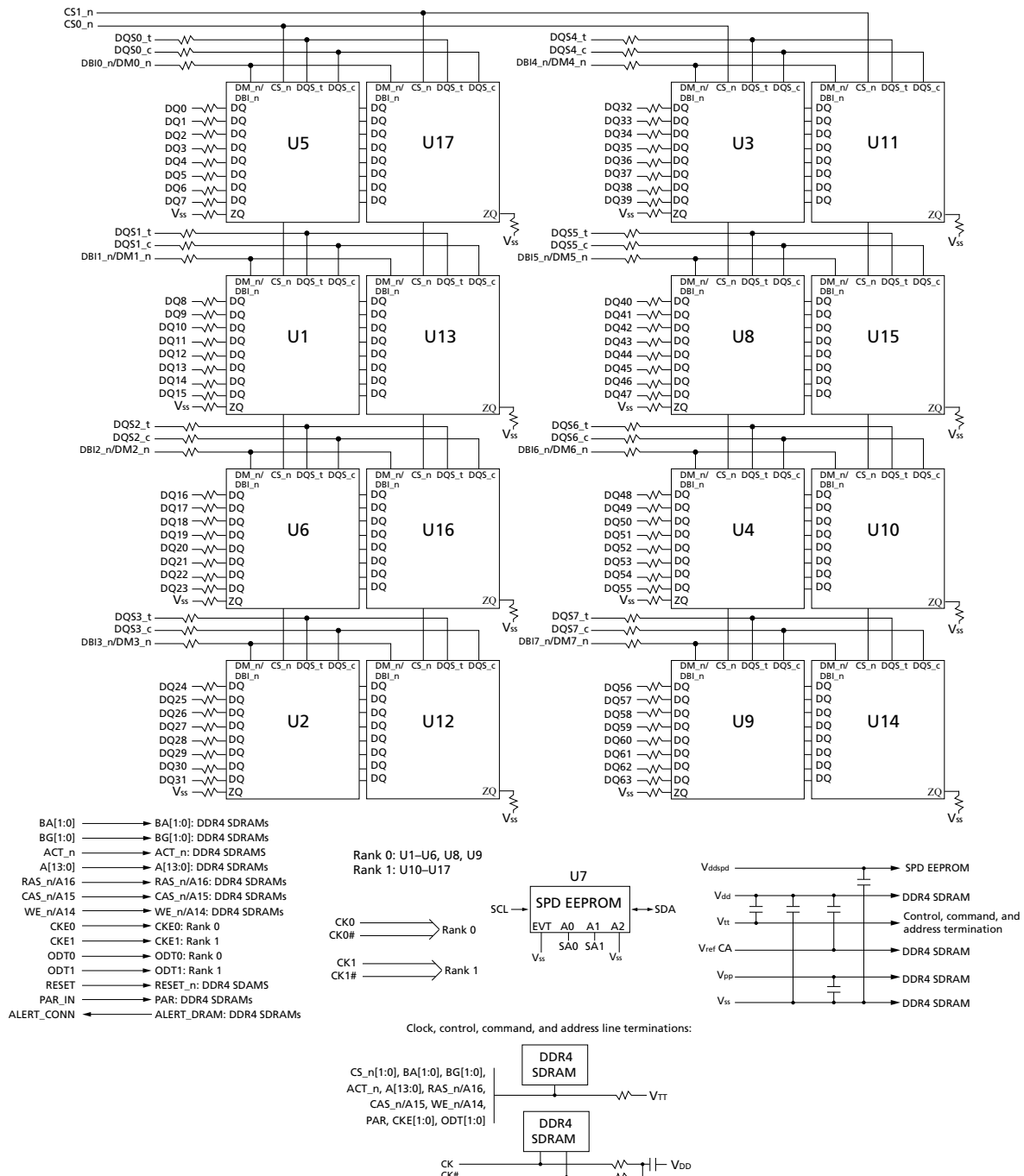
Figure 4: Functional Block Diagram, R/C-E1 (PCB 2261)
