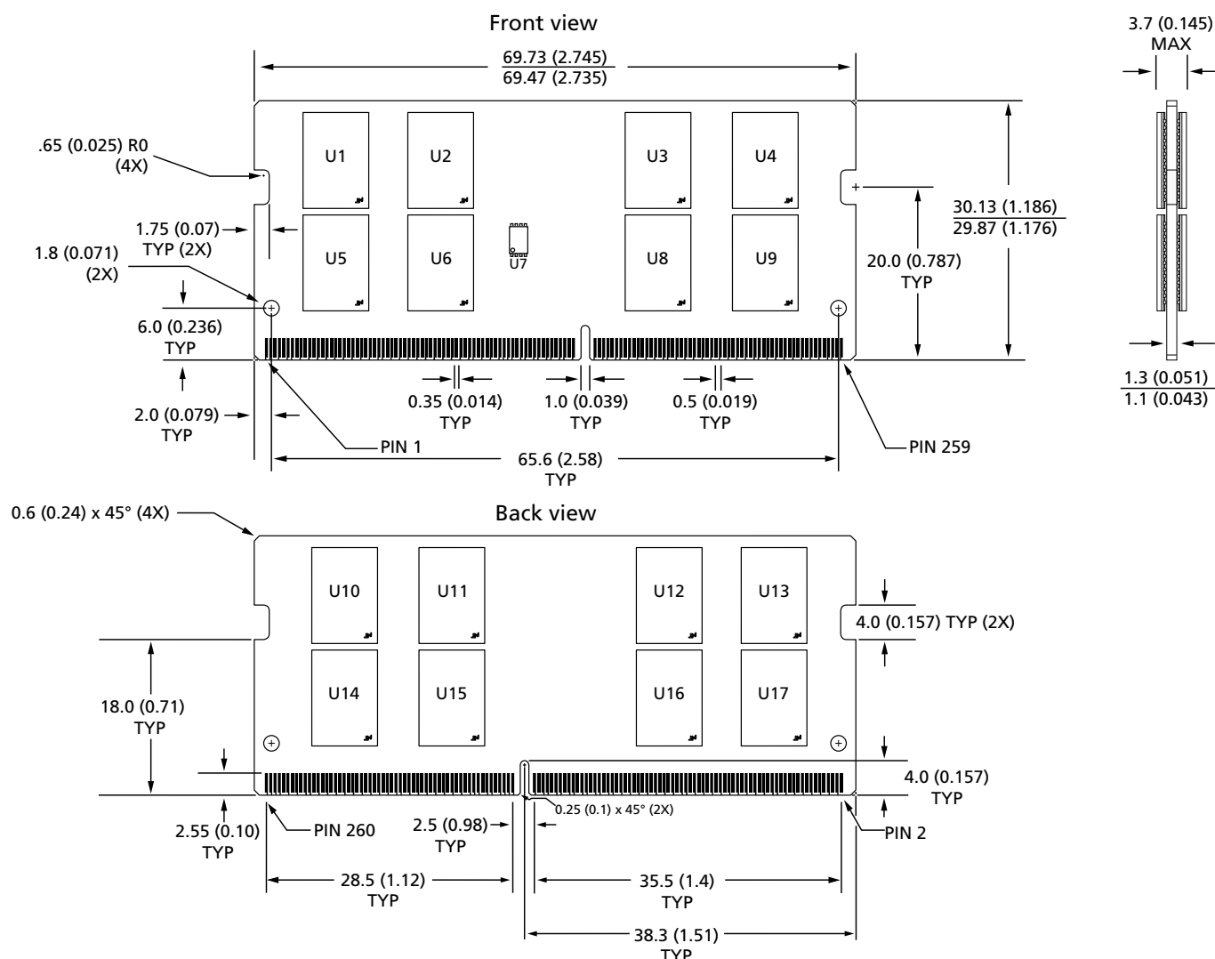
Figure 6: 260-Pin DDR4 SODIMM, R/C-E1 (PCB 2261)
