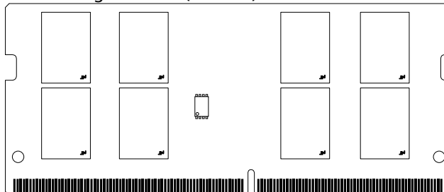
Figure 2: 260-Pin SODIMM (MO-310, R/C E1)
