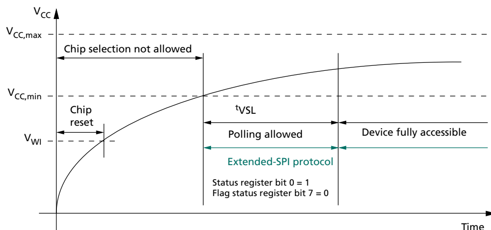
Figure 44: Power-Up Timing
