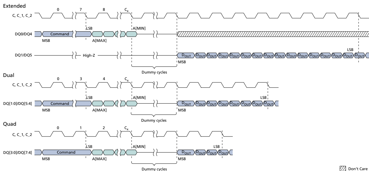
Figure 24: DTR FAST READ – 0Dh/0Eh 3
