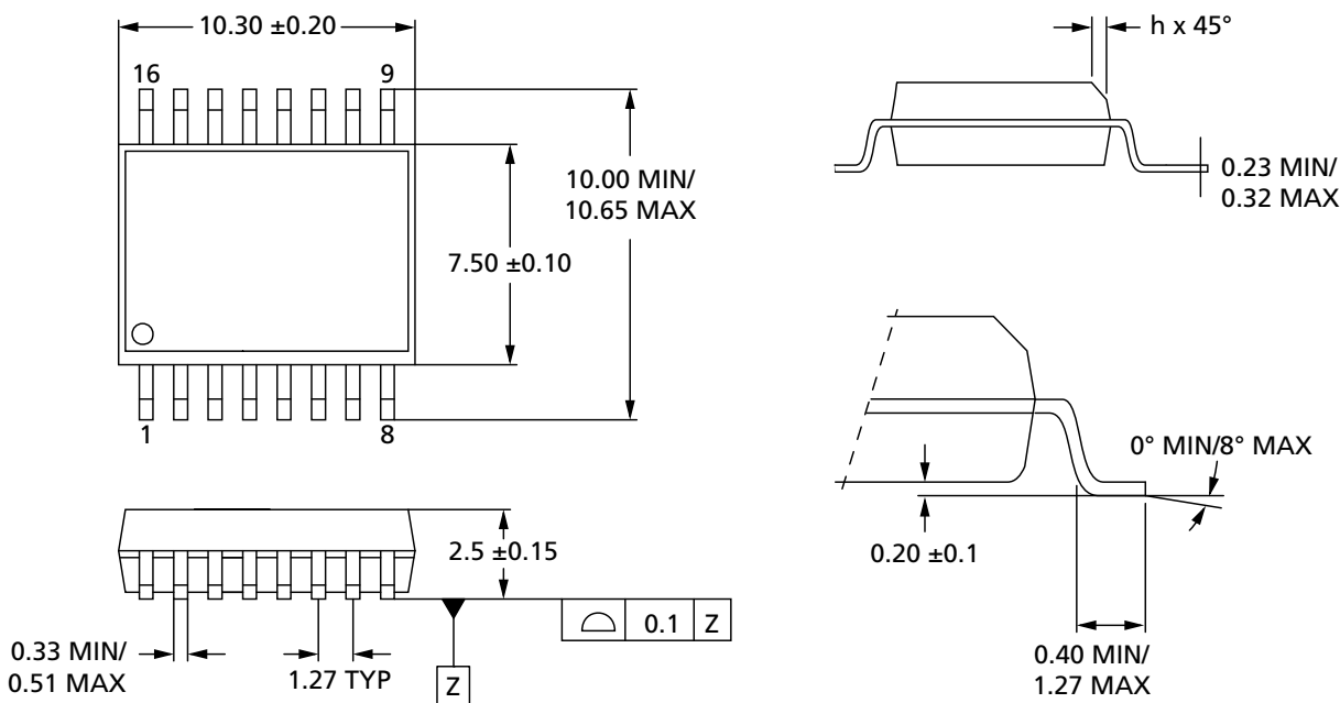
Figure 9: 16-Pin SOP2 – 300 mil Body Width
