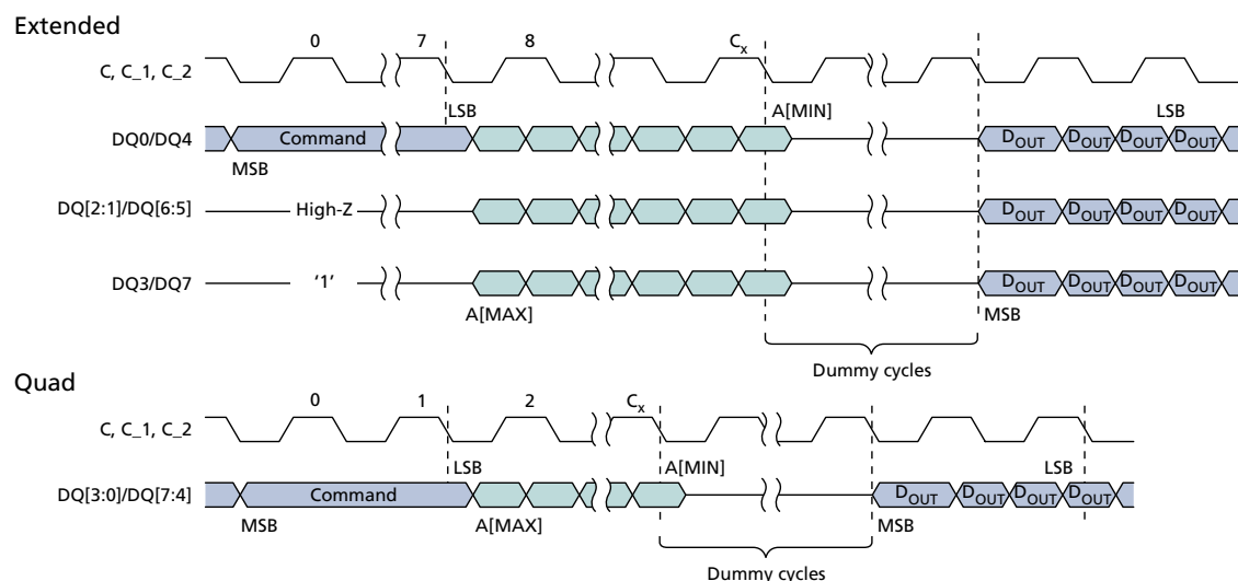
Figure 28: DTR QUAD INPUT/OUTPUT FAST READ – EDh 3
