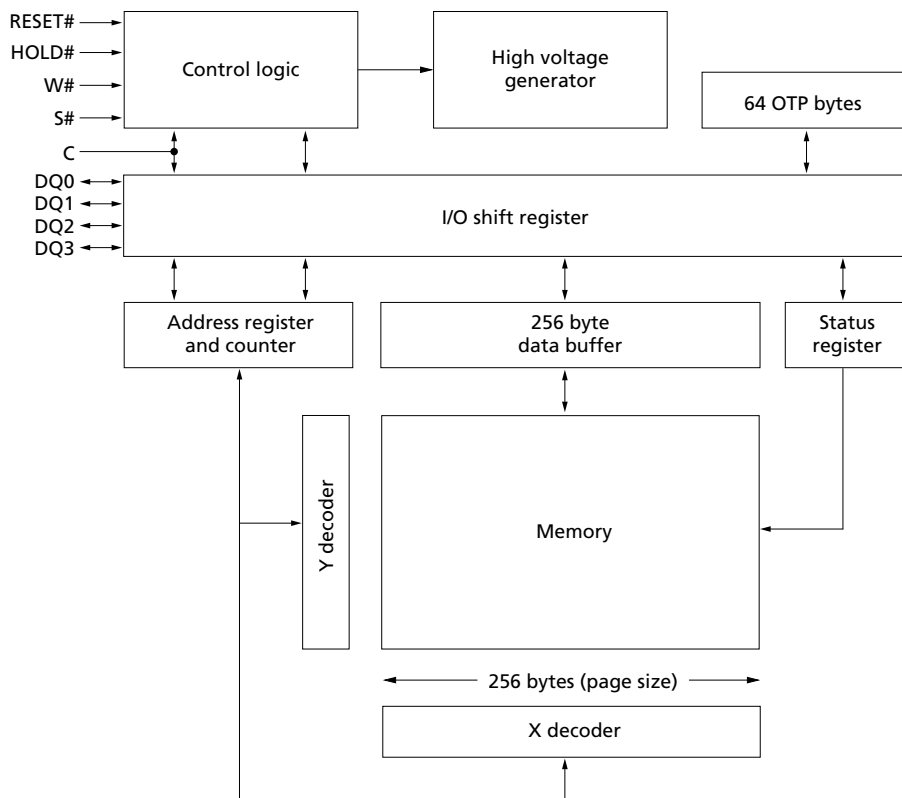
Figure 4: Block Diagram – Components and Signals
