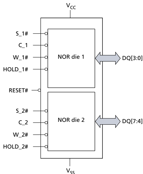
Figure 2: Logic Diagram – Separate Chip-Select and Clock Signals
