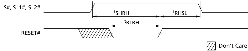
Figure 46: Reset AC Timing During PROGRAM or ERASE Cycle
