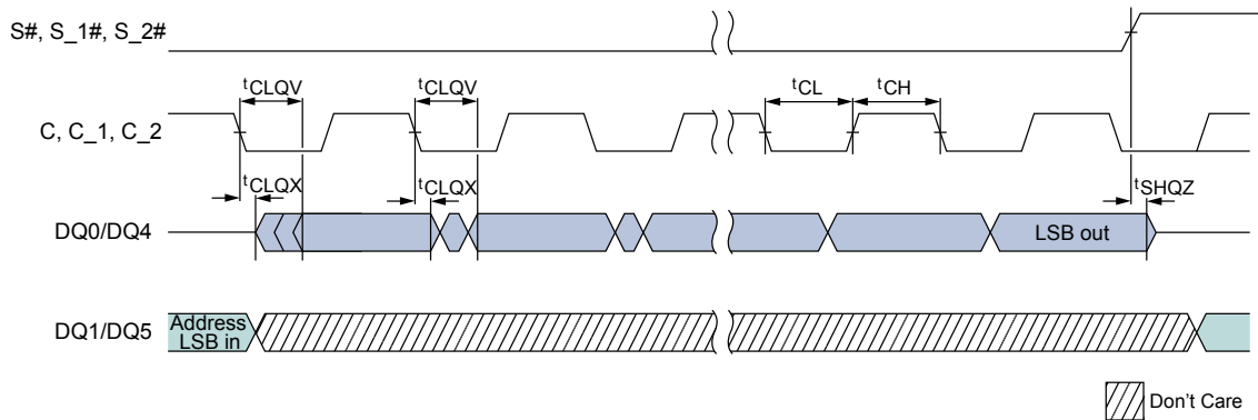
Figure 51: Output Timing
