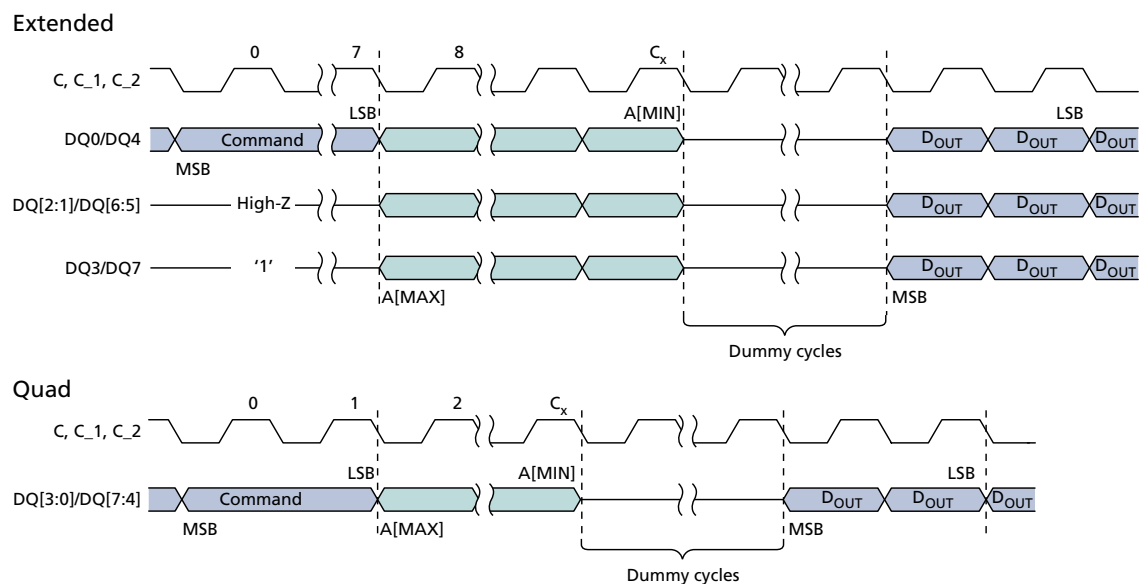
Figure 22: QUAD INPUT/OUTPUT FAST READ – EBh/ECh 3
