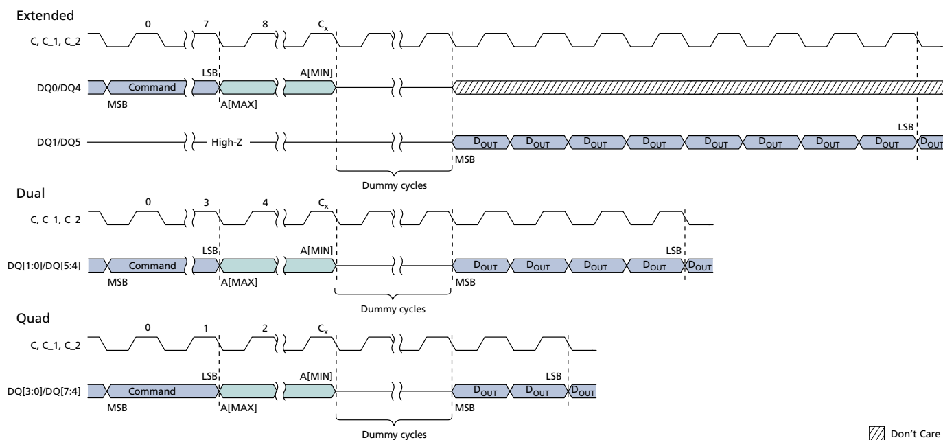
Figure 18: FAST READ – 0Bh/0Ch 3
