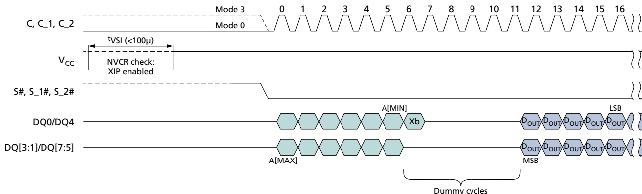
Figure 43: XIP Mode Directly After Power-On
