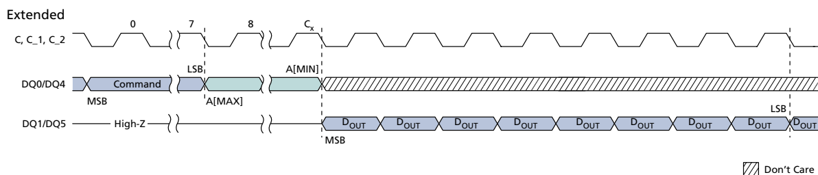
Figure 17: READ – 03h/13h 3
