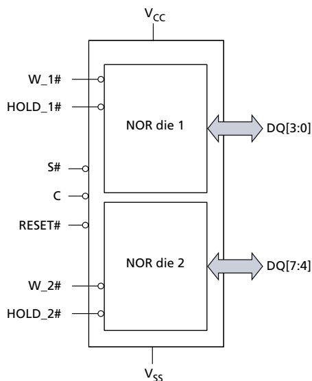
Figure 3: Logic Diagram – Shared Chip-Select and Clock Signals
