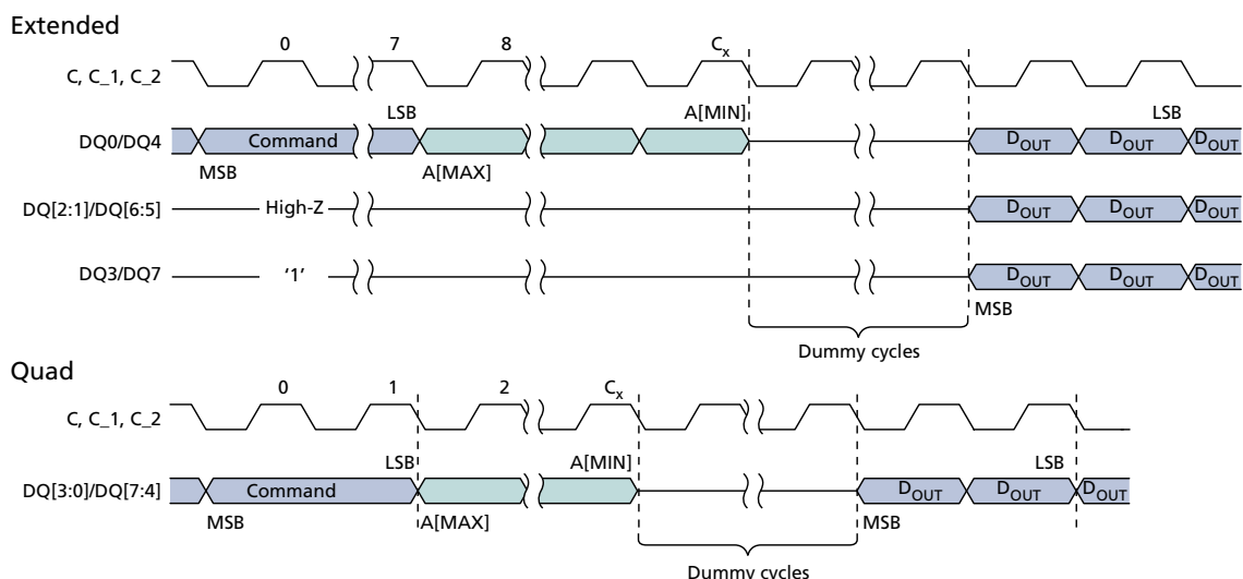
Figure 21: QUAD OUTPUT FAST READ – 6Bh/6Ch 3
