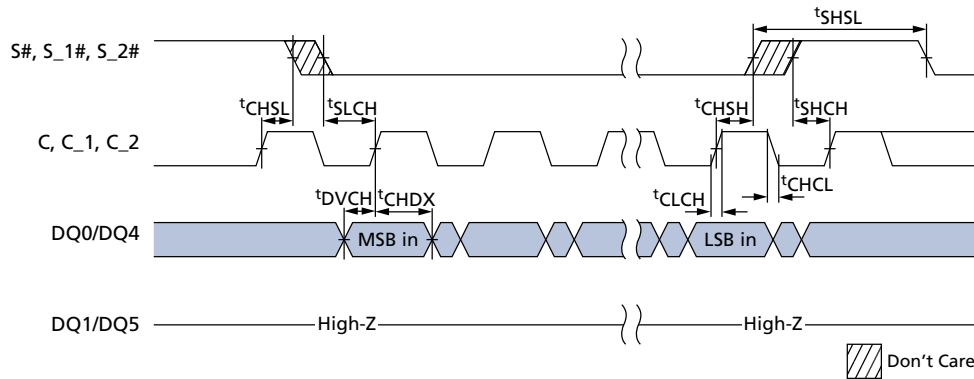
Figure 48: Serial Input Timing
