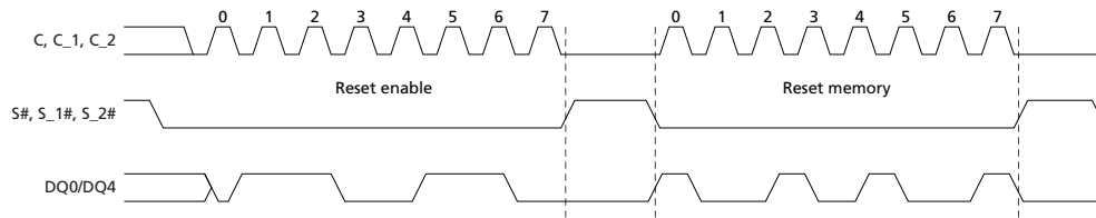
Figure 47: Reset Enable and Reset Memory Timing
