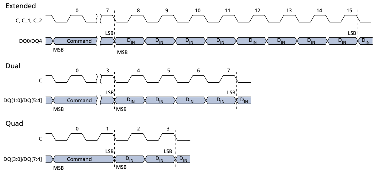
Figure 31: WRITE REGISTER Timing
