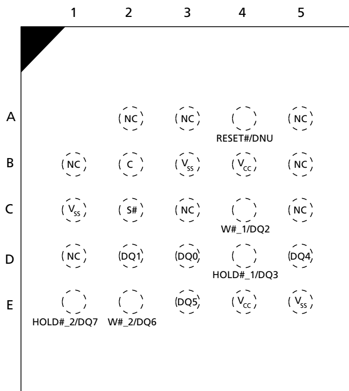
Figure 7: 24-Ball TBGA – 5 x 5 (Balls Down) (Single Chip-Select and Clock)
