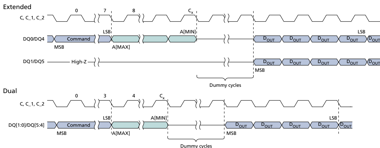
Figure 19: DUAL OUTPUT FAST READ – 3Bh/3Ch 3
