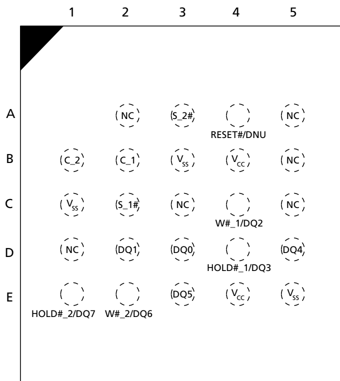
Figure 8: 24-Ball TBGA – 5 x 5 (Balls Down) (Double Chip-Select and Clock)
