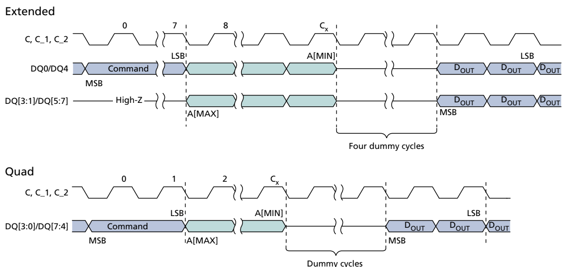
Figure 23: QUAD INPUT/OUTPUT WORD READ – E7h 3
