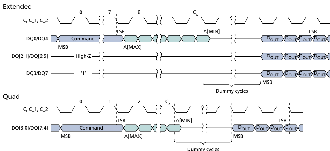
Figure 27: DTR QUAD OUTPUT FAST READ – 6Dh 3
