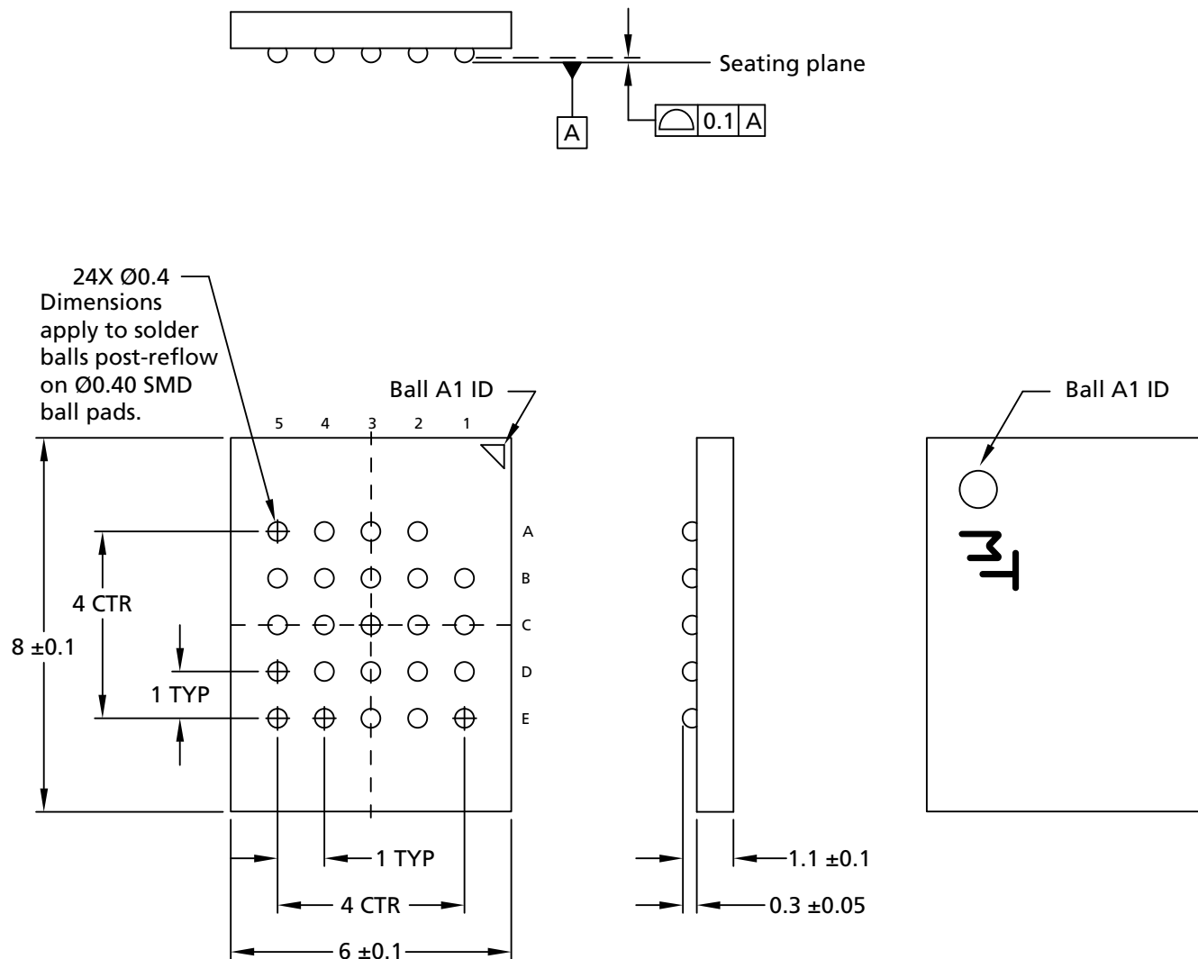
Figure 10: 24-Ball T-PBGA (5 x 5 ball grid array) – 6mm x 8mm
