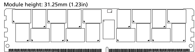
Figure 1: 288-Pin LRDIMM (MO-309, R/C-E1)
