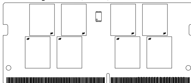
Figure 1: 260 Pin SODIMM (MO-310, R/C E)
