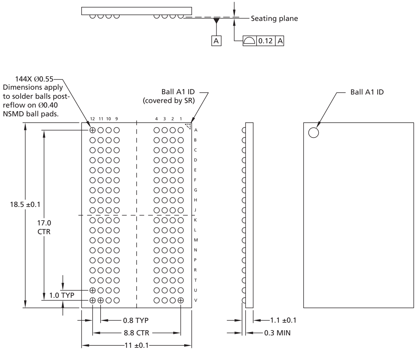
Figure 5: 144-Ball FBGA
