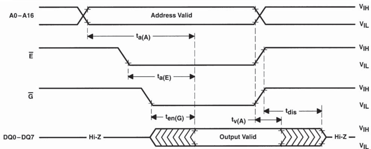
FIGURE 3. READ-CYCLE TIMING
