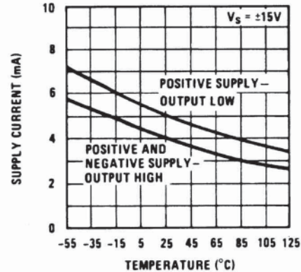
Supply Current
