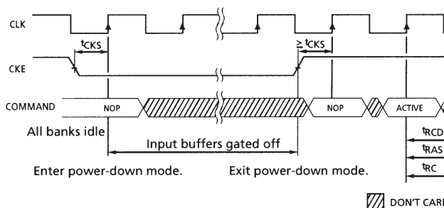
FIGURE 21: Power-Down
