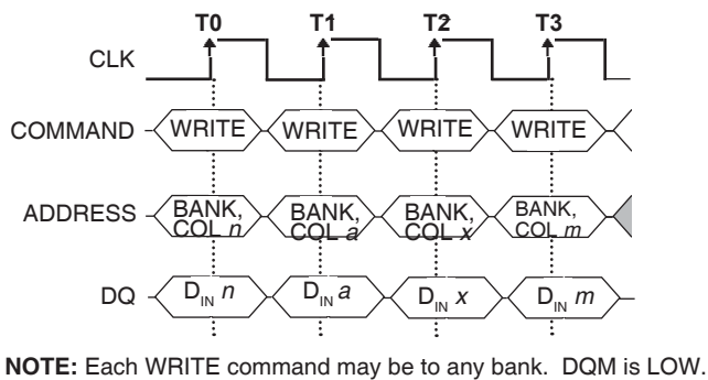
Figure 16 RANDOM WRITE CYCLES
