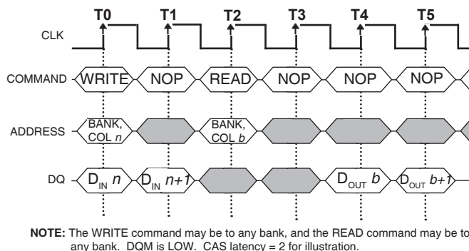
Figure 17 WRITE TO READ
