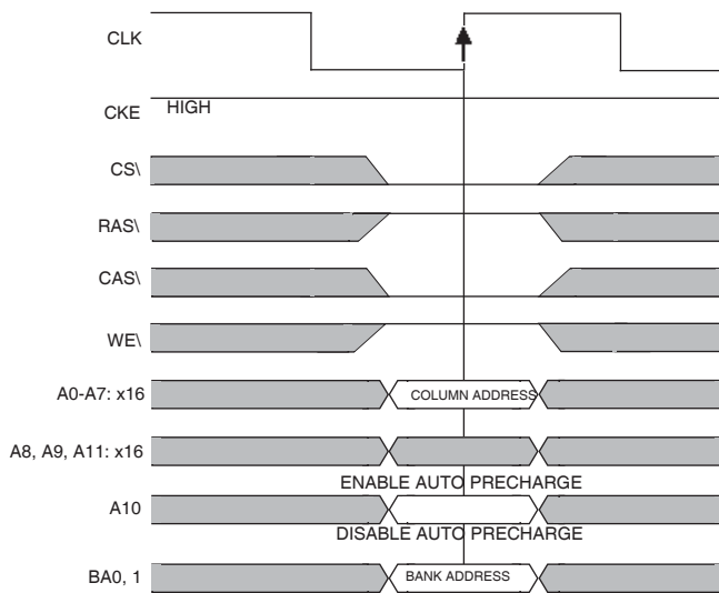
Figure 5 READ COMMAND
