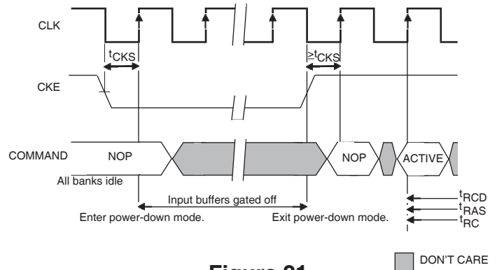
Figure 21 POWER-DOWN
