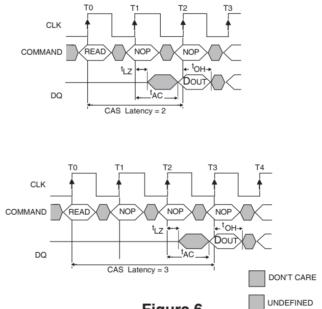
Figure 6 CAS LATENCY
