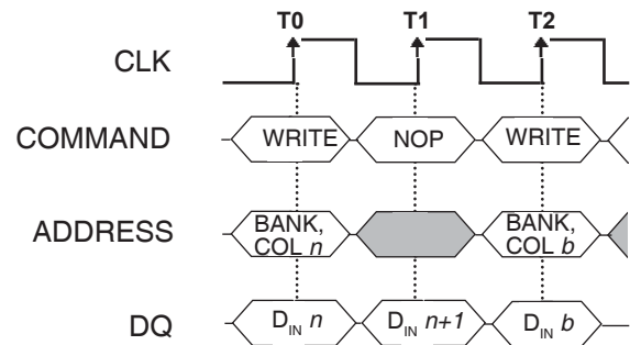
Figure 14 WRITE BURST
