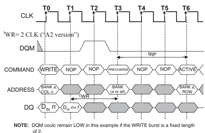
Figure 18 WRITE TO PRECHARGE
