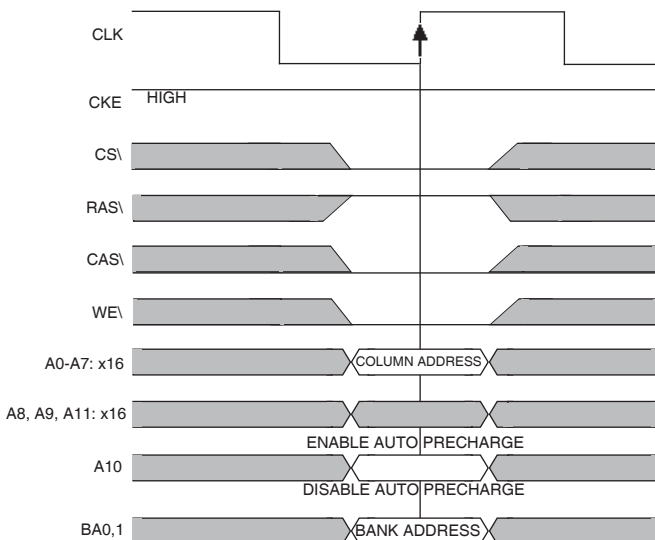
Figure 13 WRITE COMMAND
