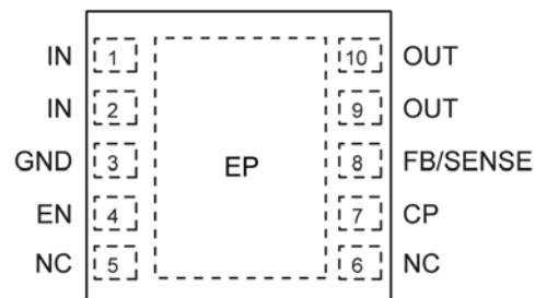
10-Pin 3mm x 3mm MLF ® (ML)
