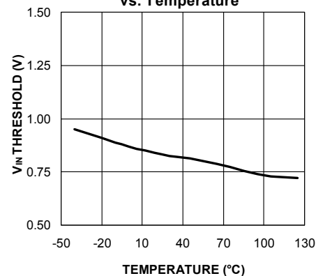
V_{IN} Turn-On Threshold vs. Temperature
