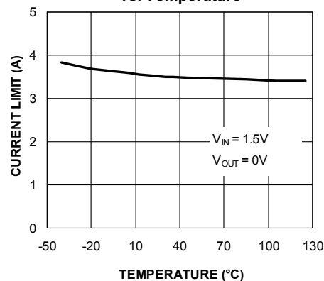
Short-Circuit Current vs. Temperature
