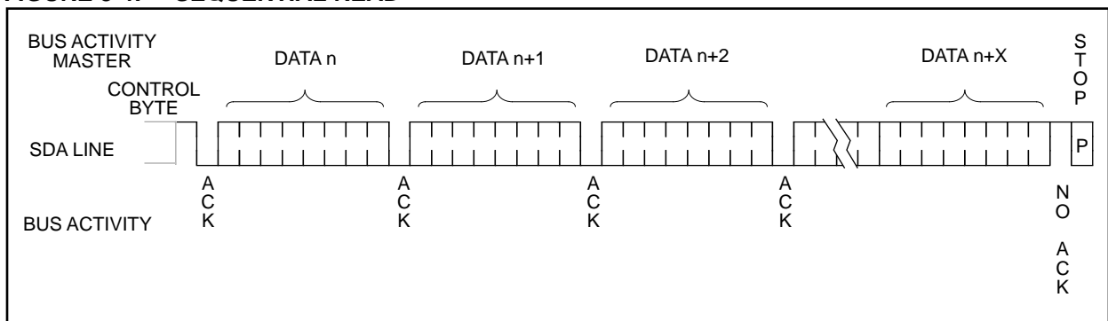
FIGURE 8-4: SEQUENTIAL READ
