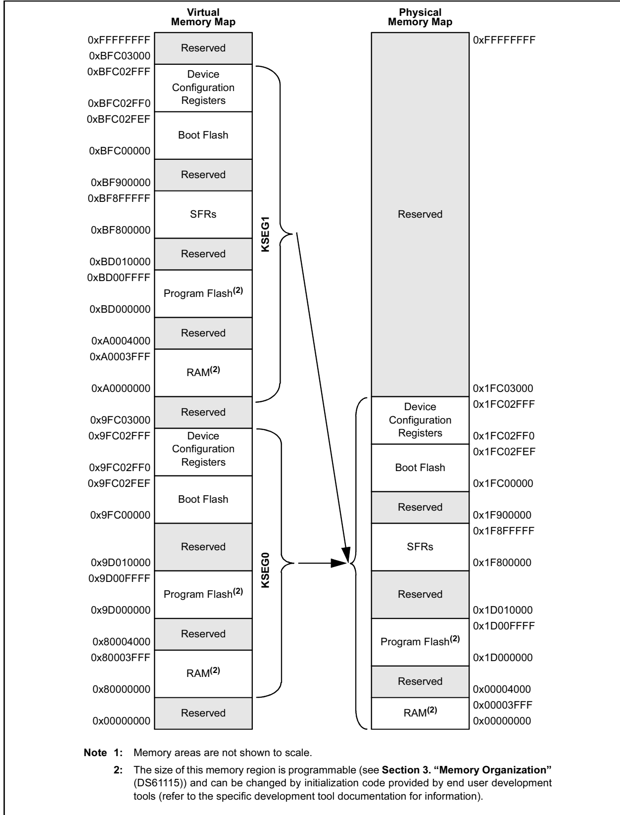
FIGURE 4-2: MEMORY MAP ON RESET FOR PIC32MX534F064H AND PIC32MX534F064L DEVICES (1)
