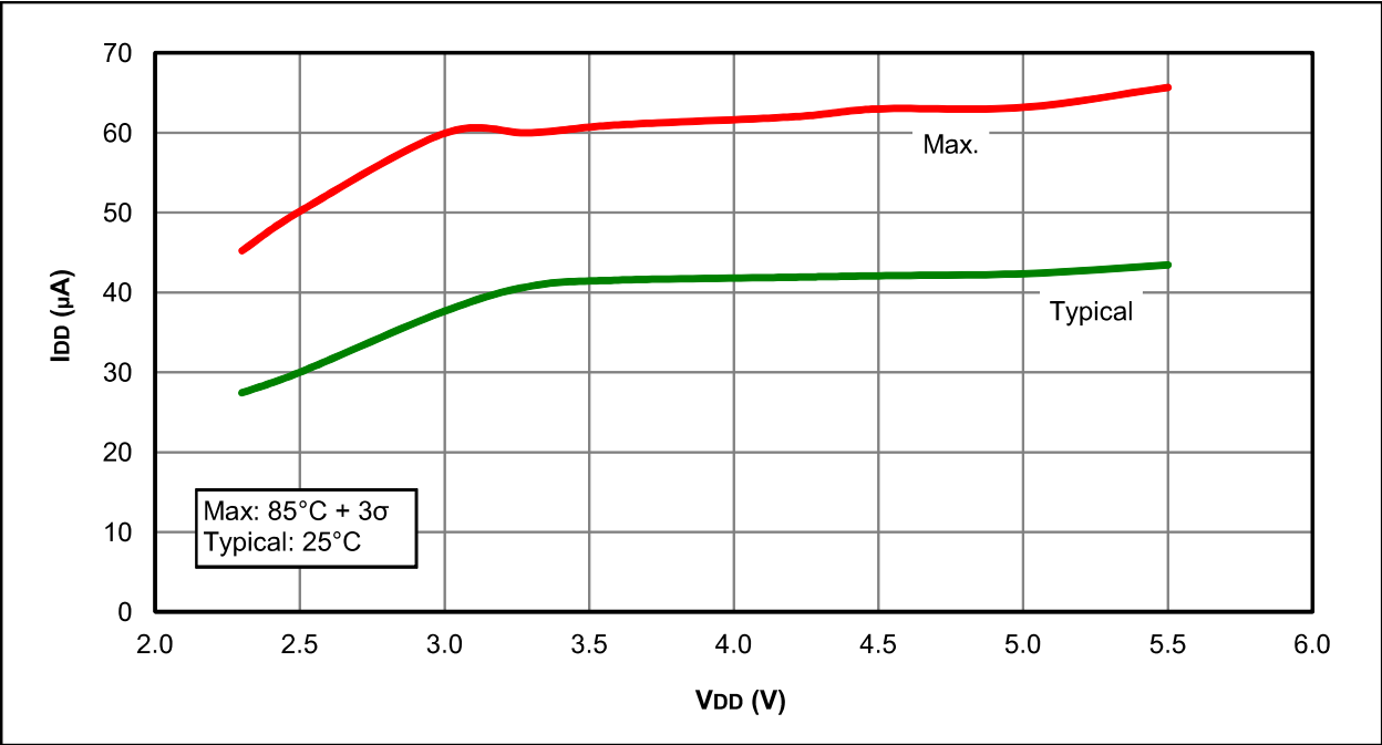
FIGURE 31-10: I_{DD} , EXTERNAL CLOCK (ECL), LOW-POWER MODE, F_{osc} = 500\text{ kHz} , PIC12F1840 ONLY
