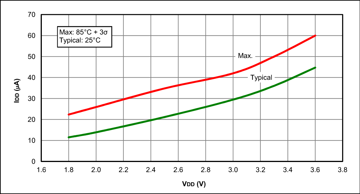
FIGURE 31-9: I_{DD} , EXTERNAL CLOCK (ECL), LOW-POWER MODE, F_{osc} = 500\text{ kHz} , PIC12LF1840 ONLY
