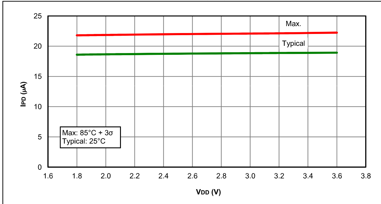
FIGURE 31-35: I_{PD} , FIXED VOLTAGE REFERENCE (FVR), PIC12LF1840 ONLY
