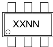
6-Lead SOT-23
