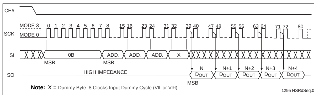
Figure 6: High-Speed-Read Sequence
