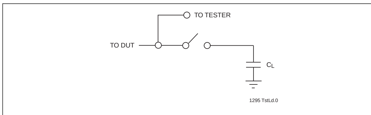
Figure 27: A Test Load Example
