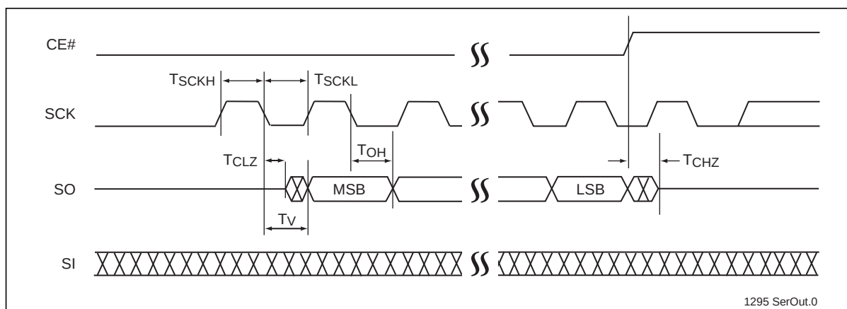
Figure 23: Serial Output Timing Diagram
