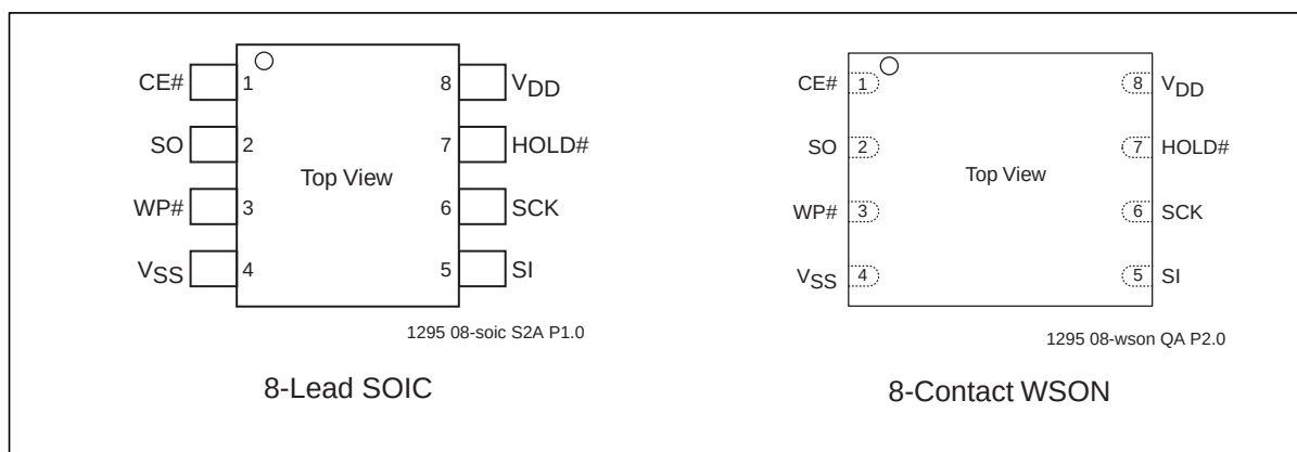
Figure 2: Pin Assignments
