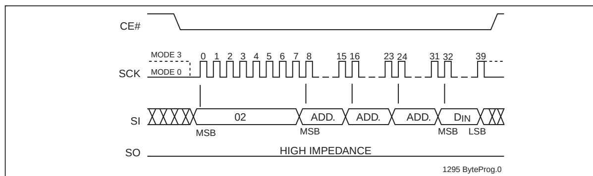
Figure 7: Byte-Program Sequence
