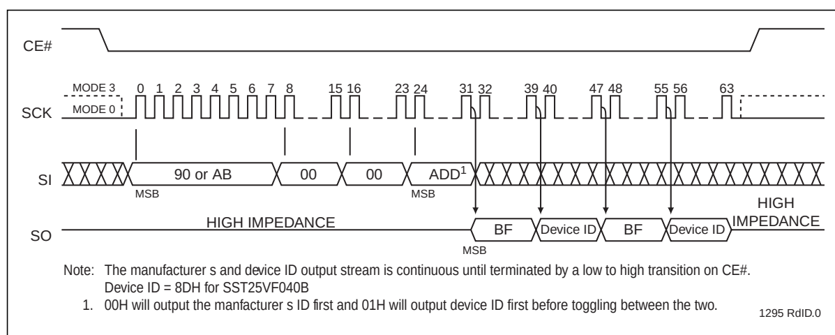
Figure 21: Read-ID Sequence
