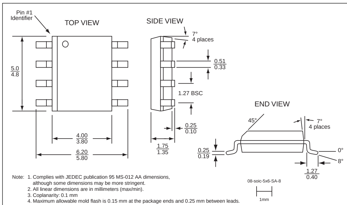
Figure 29: 8-Lead Small Outline Integrated Circuit (SOIC) 150mil Body Width (5mm x 6mm) SST Package Code: SA
