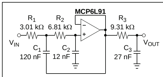
FIGURE 4-5: Chebyshev Filter.
