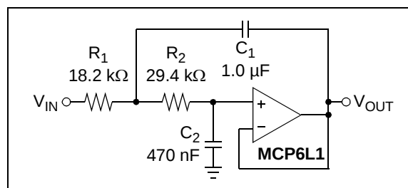
FIGURE 4-6: Sallen Key Topology.
