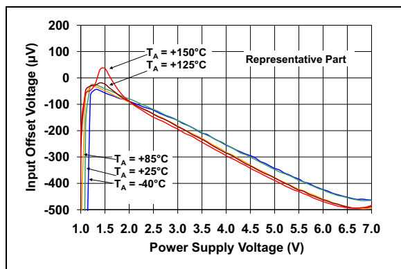
FIGURE 2-9: Input Offset Voltage vs. Power Supply Voltage.
