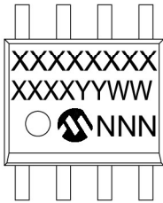
8-Lead SOIC (150 mil)(MCP6401, MCP6402, MCP6407)
