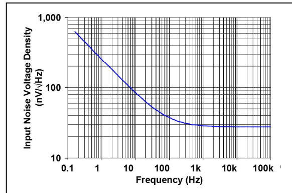
FIGURE 2-10: Input Noise Voltage Density vs. Frequency.
