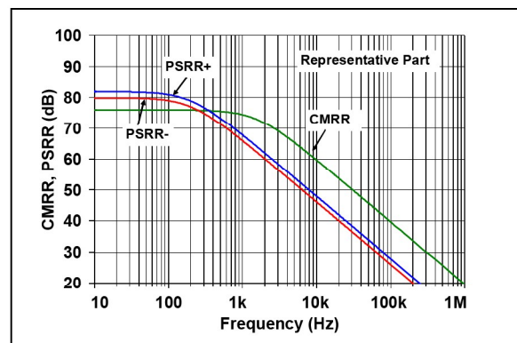
FIGURE 2-12: CMRR, PSRR vs. Frequency.
