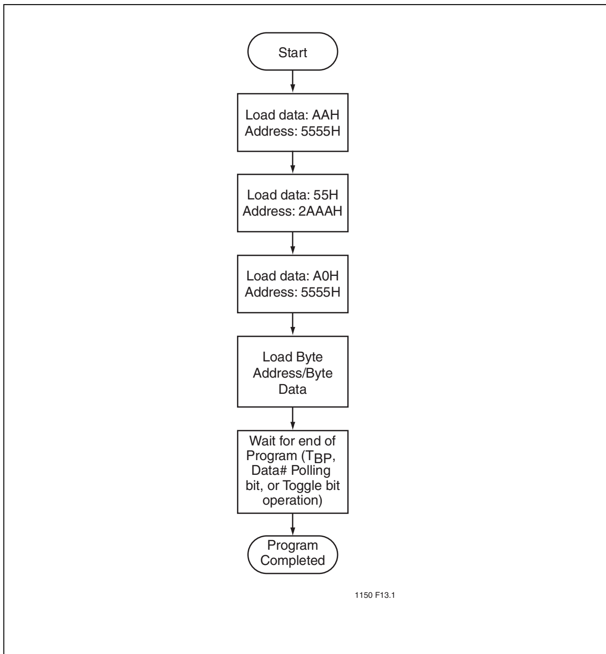
Figure 17: Byte-Program Algorithm
