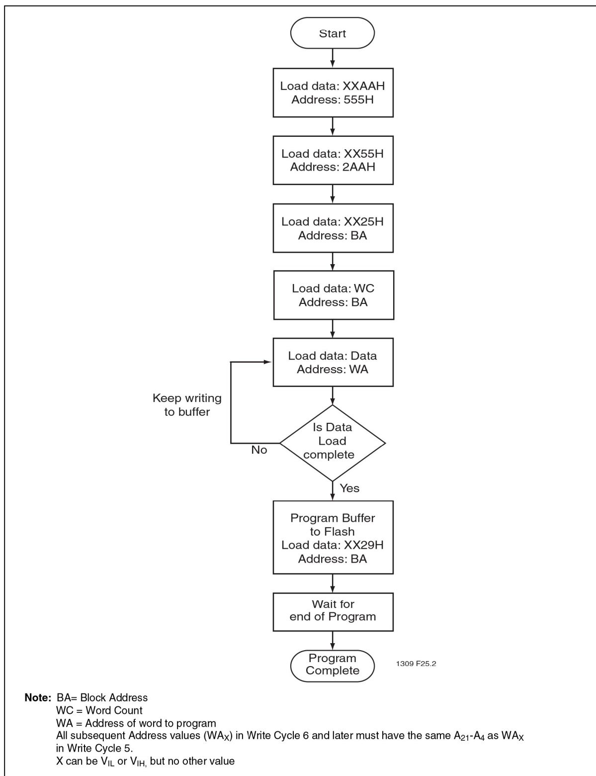
Figure 25: Write-Buffer Programming
