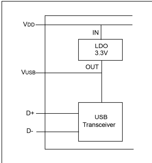
FIGURE 1-2: MCP2200 INTERNAL POWER SUPPLY DETAILS
