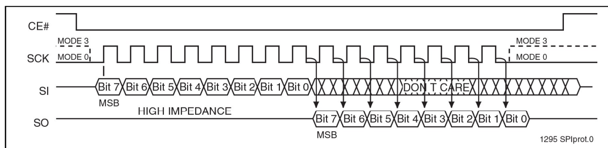
Figure 3: SPI Protocol
