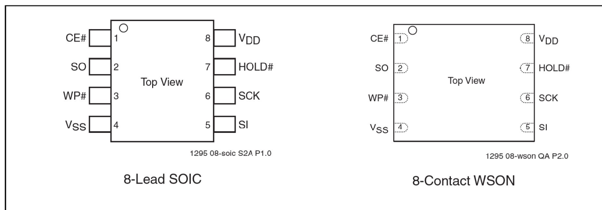
Figure 2: Pin Assignments
