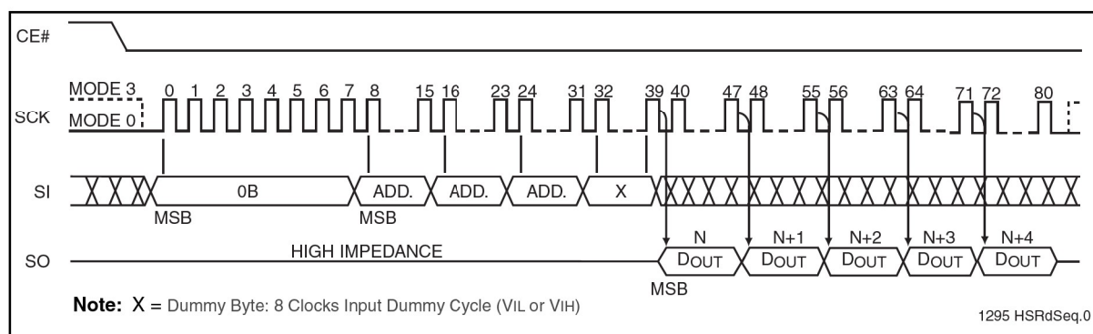
Figure 6: High-Speed-Read Sequence
