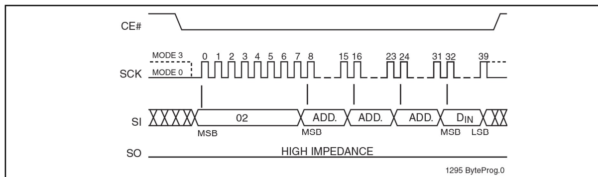
Figure 7: Byte-Program Sequence
