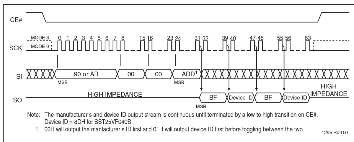
Figure 21: Read-ID Sequence
