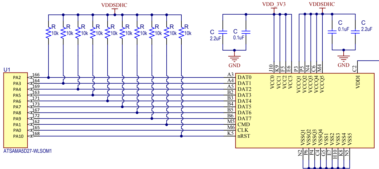
Figure 7-23. e-MMC Interface Example Schematic
