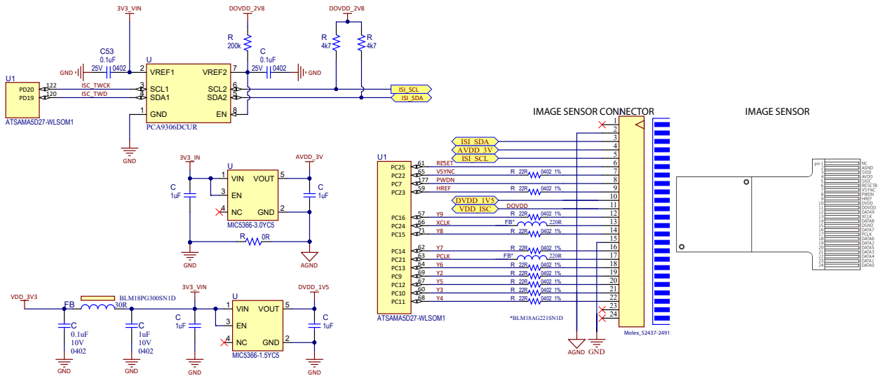
Figure 7-30. EMI Improvement Example
