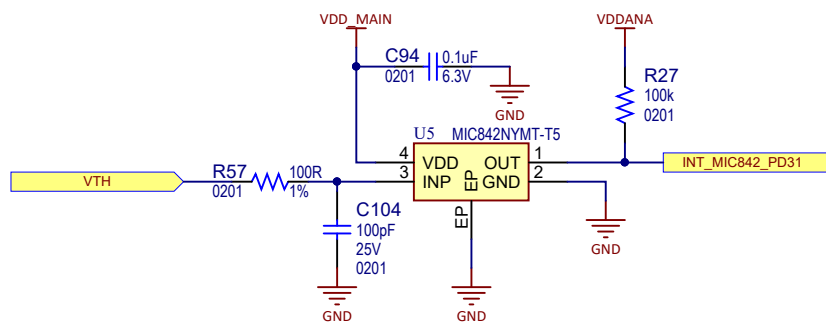
Figure 7-14. Voltage Threshold Detector Schematic
