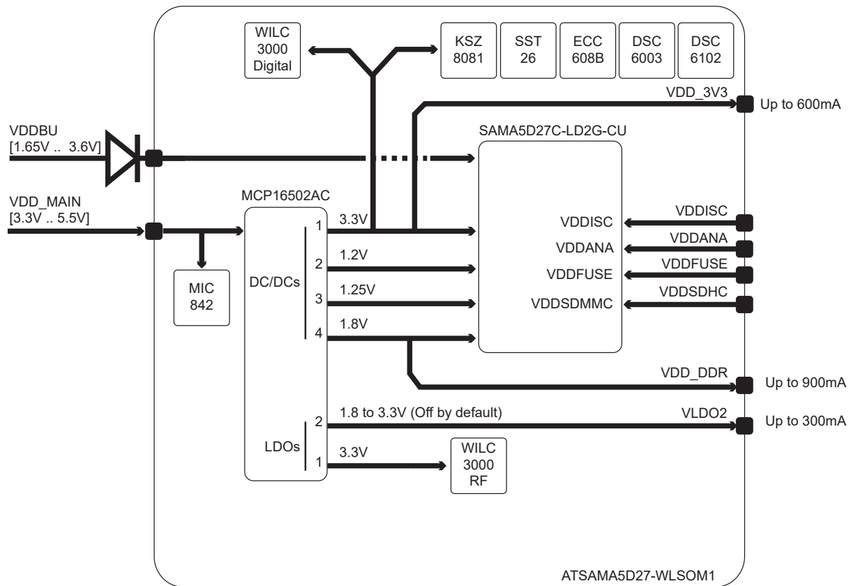
Figure 7-4. ATSAMA5D27-WLSOM1 Power Architecture
