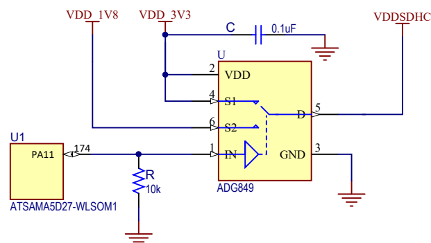
Figure 7-22. e-MMC Power Switch Example Schematic
