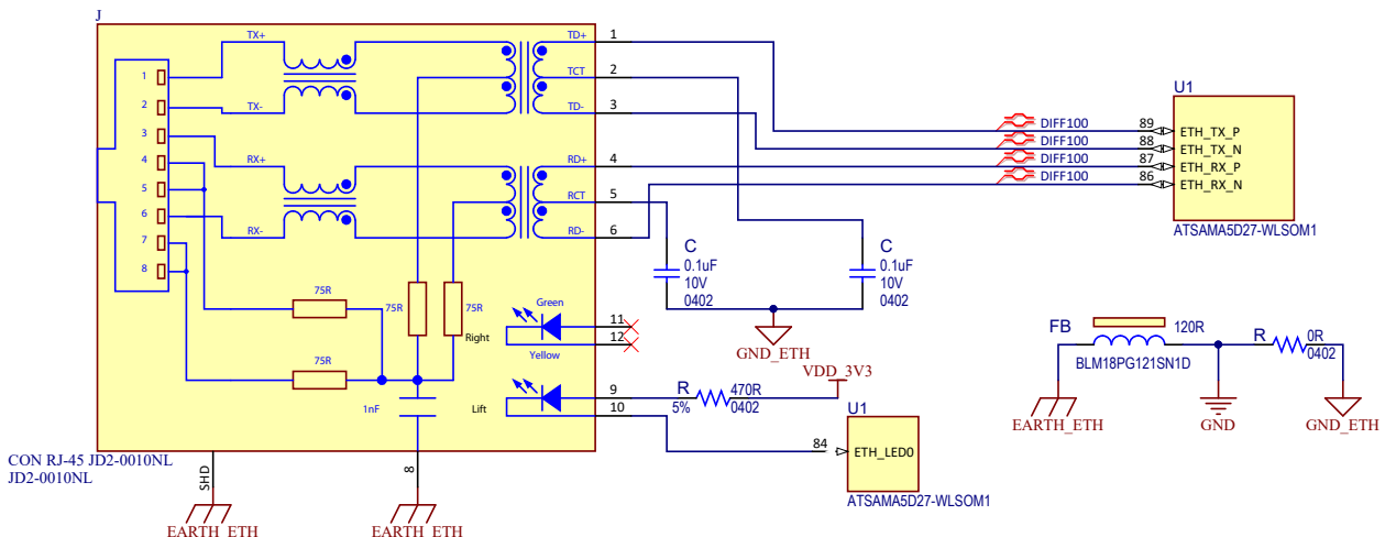
Figure 7-13. Ethernet Phy Schematic Example
