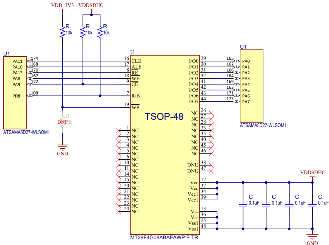
Figure 7-25. NAND Flash Interface Example Schematic
