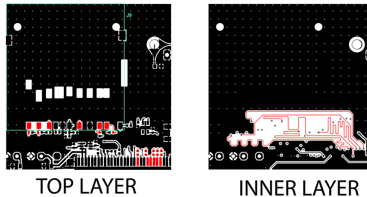
Figure 7-21. EMI Improvement Layout Example
