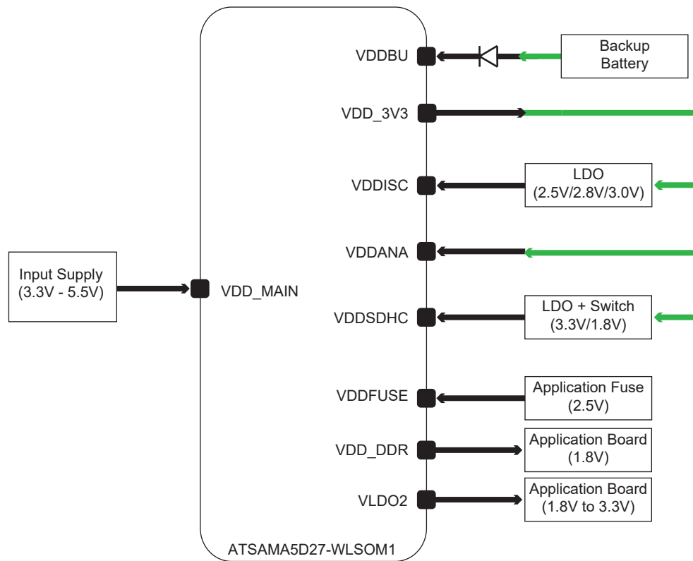
Figure 7-6. ATSAMA5D27-WLSOM1 Multiple Supplies Connection Example
