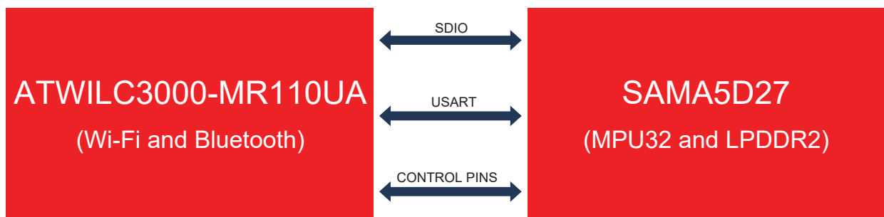
Figure 7-16. Wi-Fi/BT Radio Subsystem Block Diagram
