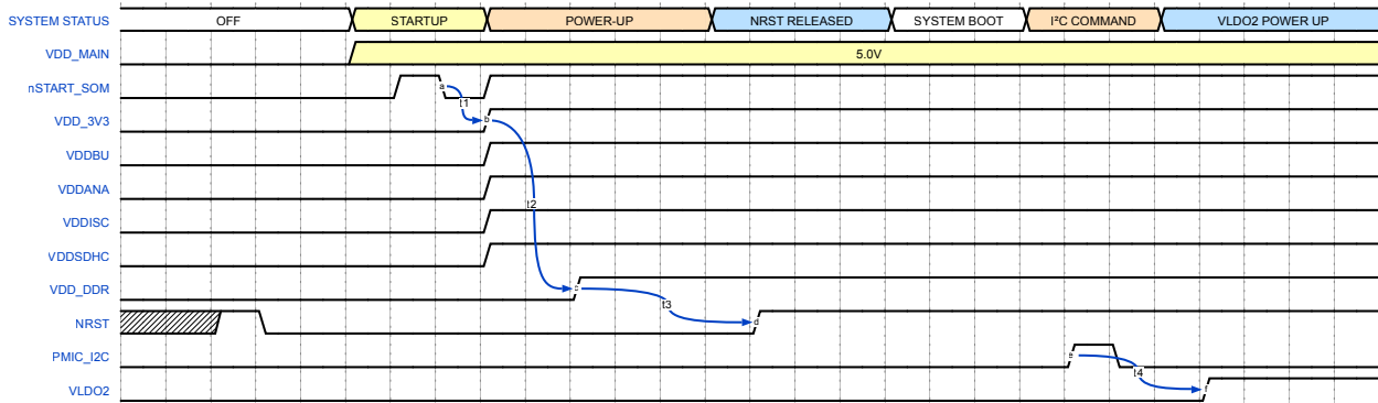
Figure 7-7. ATSAMA5D27-WLSOM1 Single Supply Connection: Power-On Sequence
