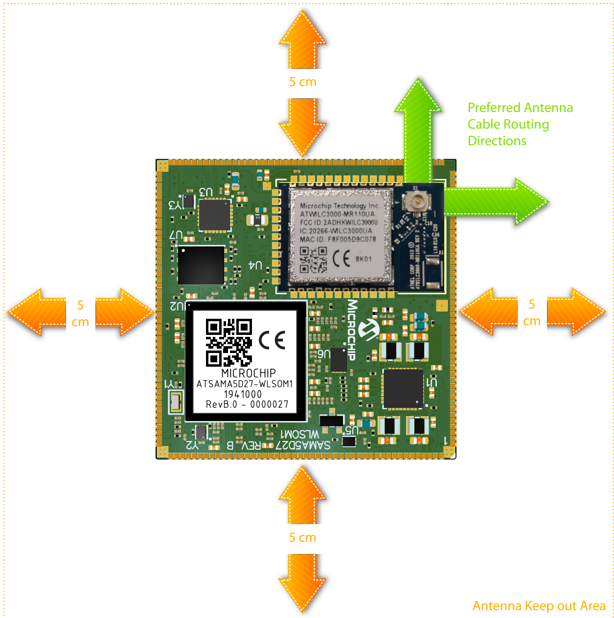
Figure 10-1. ATSAMA5D27-WLSOM1 Antenna Placement
