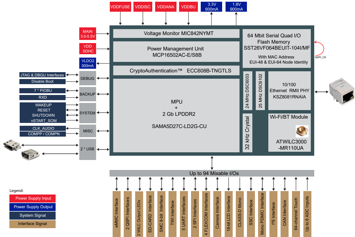
Figure 5-1. ATSAMA5D27-WLSOM1 Module Block Diagram
