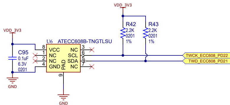
Figure 7-3. ECC608B Secure Element Schematic
