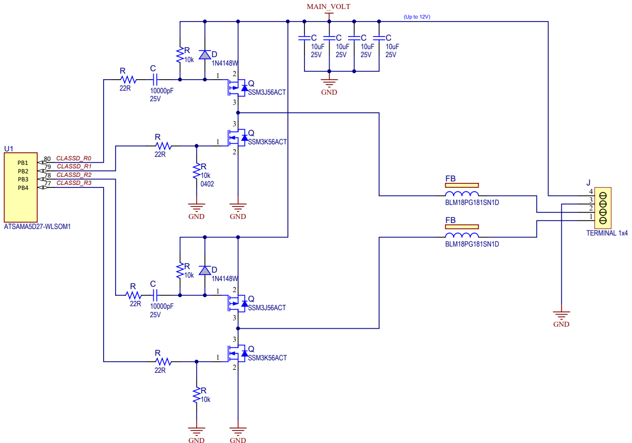
Figure 7-31. CLASS-D Interface Example Schematic
