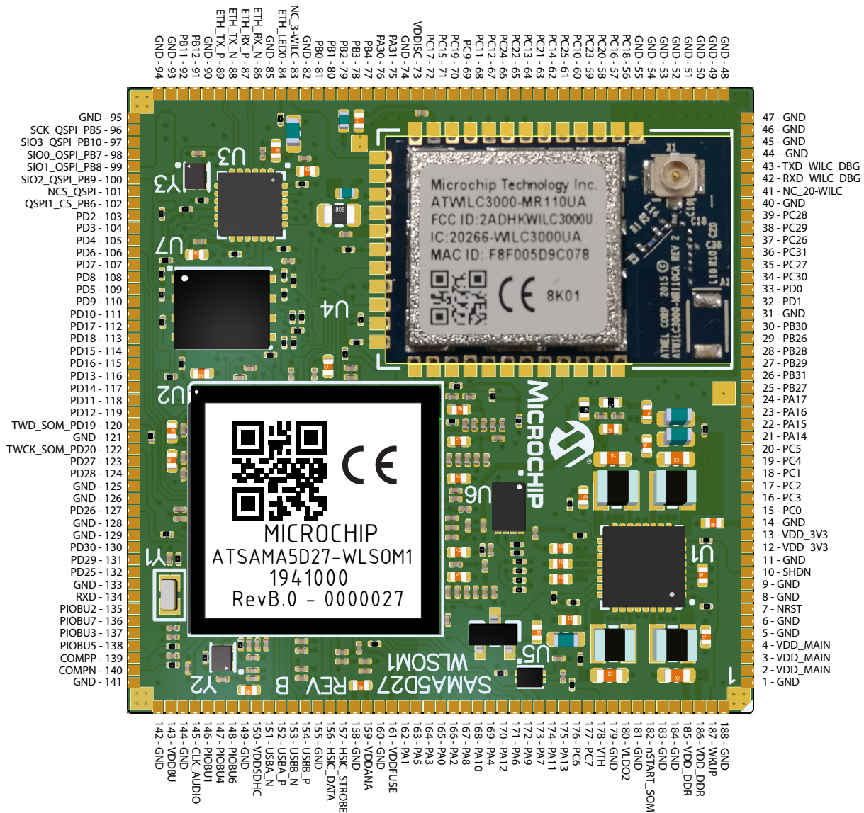
Figure 6-1. ATSAMA5D27-WLSOM1 Pin Assignment
