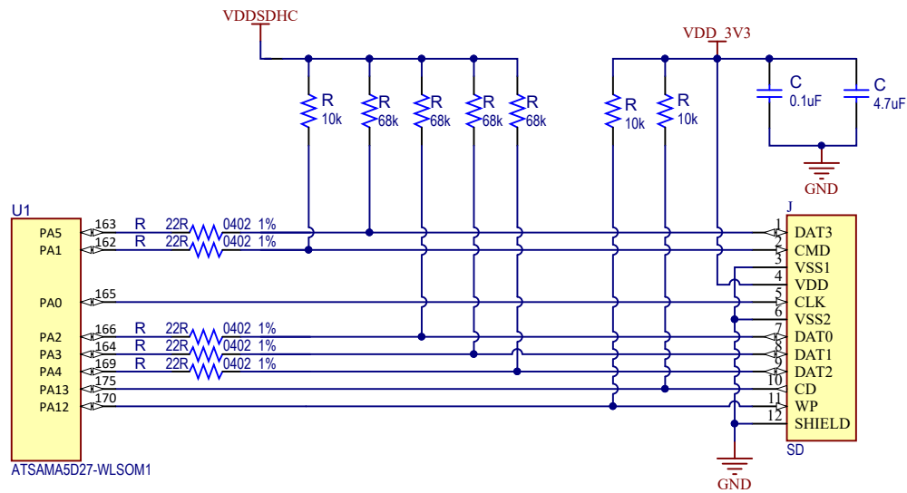
Figure 7-18. 4-bit SD Card Interface Example Schematic
