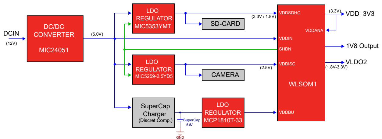
Figure 7-11. Baseboard Power Delivery Application Diagram Example
