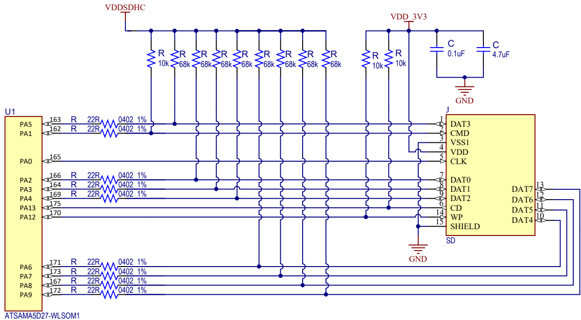
Figure 7-19. 8-bit SD Card Interface Example Schematic
