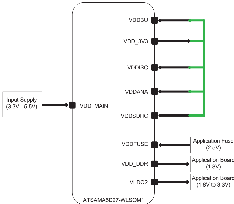
Figure 7-5. ATSAMA5D27-WLSOM1 Single Supply Connection Example
