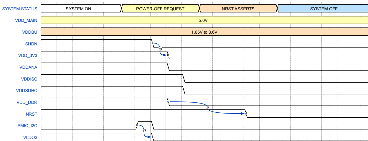
Figure 7-10. ATSAMA5D27-WLSOM1 Multiple Supplies Connections: Power-Off Sequence
