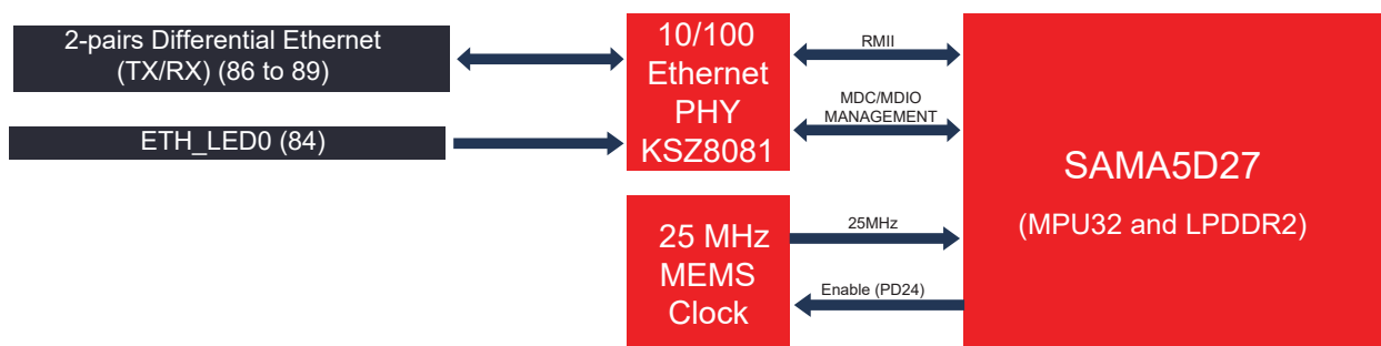
Figure 7-12. Ethernet Phy Block Diagram
