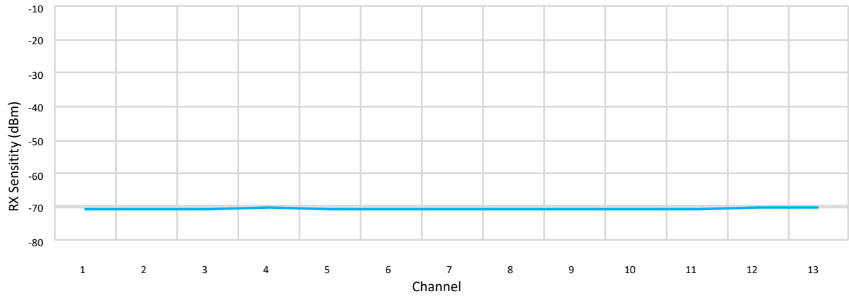
Figure 3-10. RX Sensitivity vs Channel, MCS7, 3.3V, 25°C
