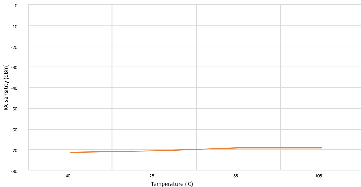
Figure 3-11. RX Sensitivity vs Temperature, MCS7, Channel 7, 3.3V
