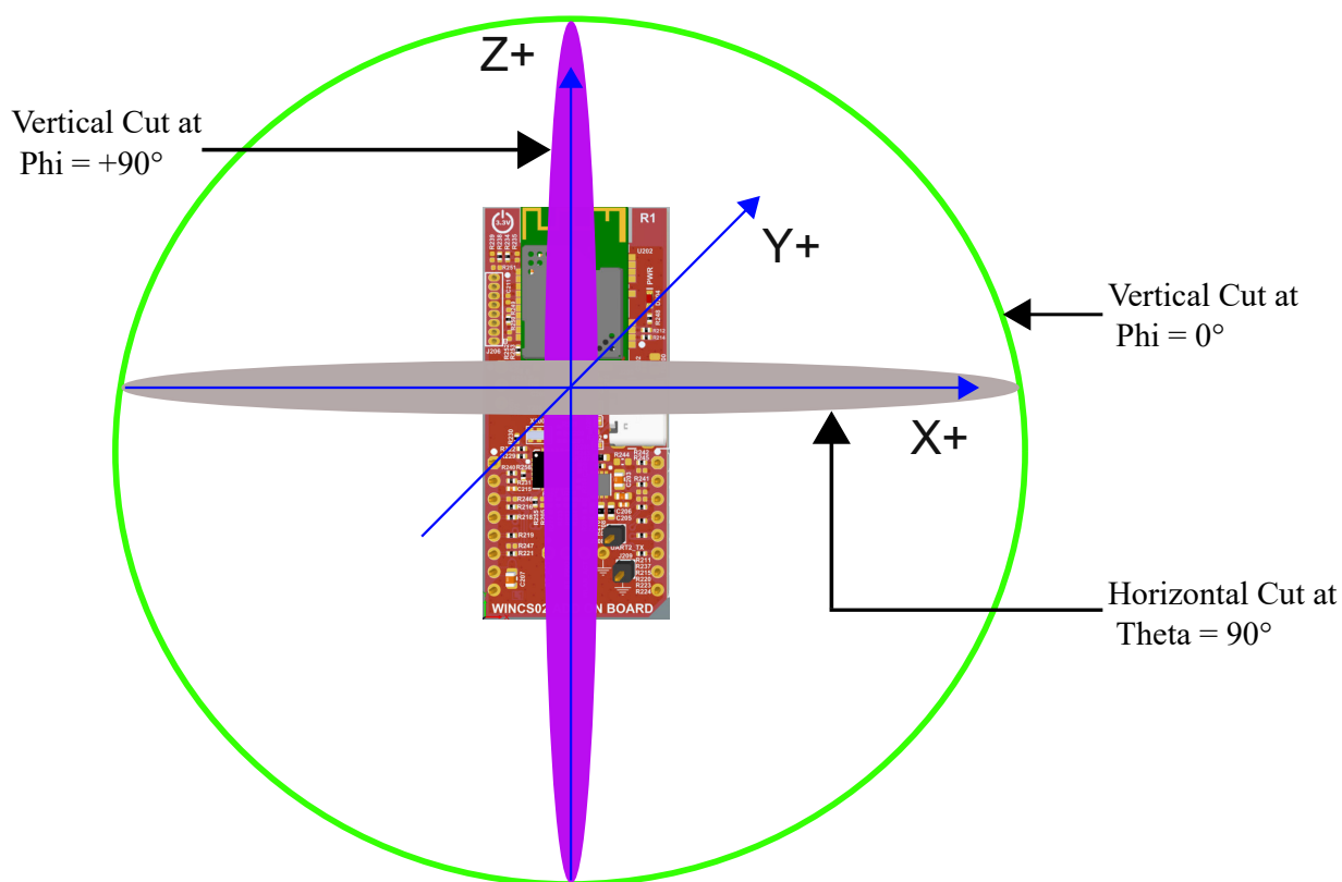
Figure 2-12. Module Orientation for Radiation Pattern Measurement
