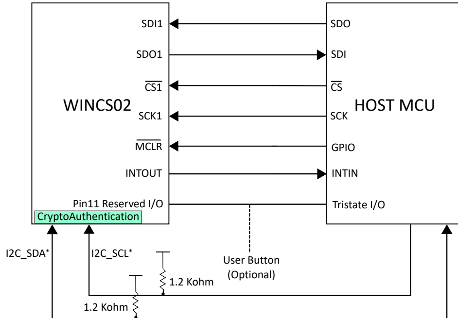
Figure 2-8. WINCS02 Module Host Interface Diagram
