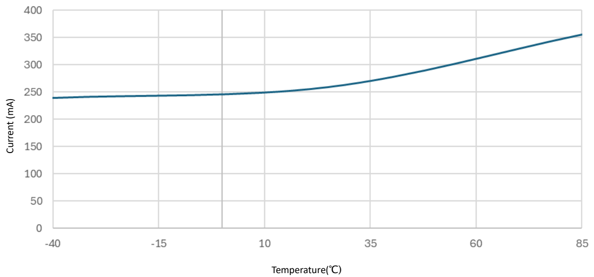
Figure 3-4. Transmit Current vs Temperature, MCS7, Channel 7, 3.3V
