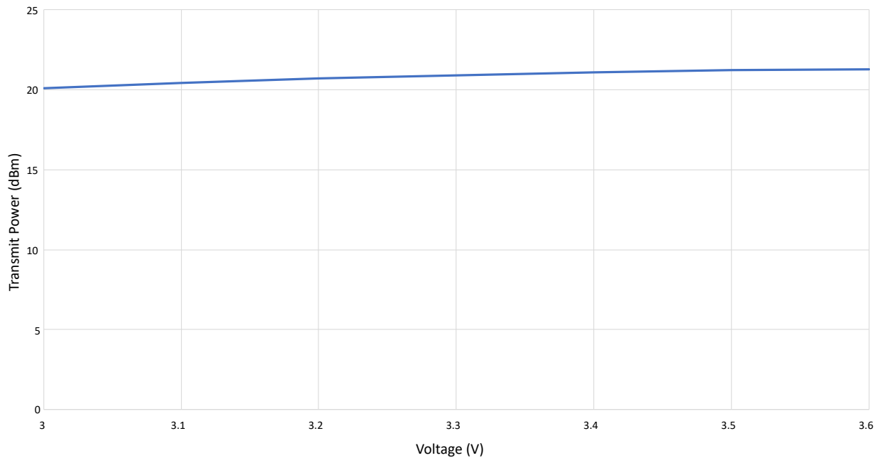
Figure 3-6. Transmit Power vs Voltage, 11b, 1Mbps, Channel 7, 25°C
