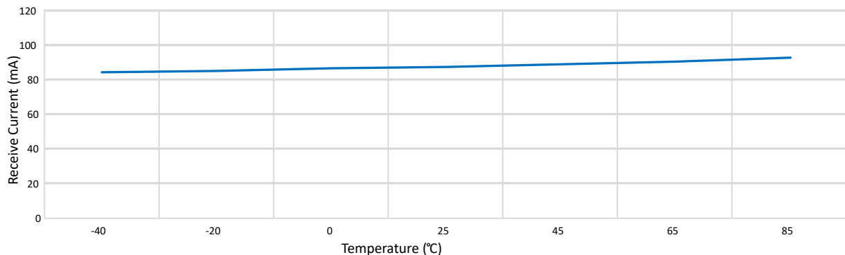
Figure 3-2. Receive Current vs Temperature, MCS7, Channel 7, 3.3V
