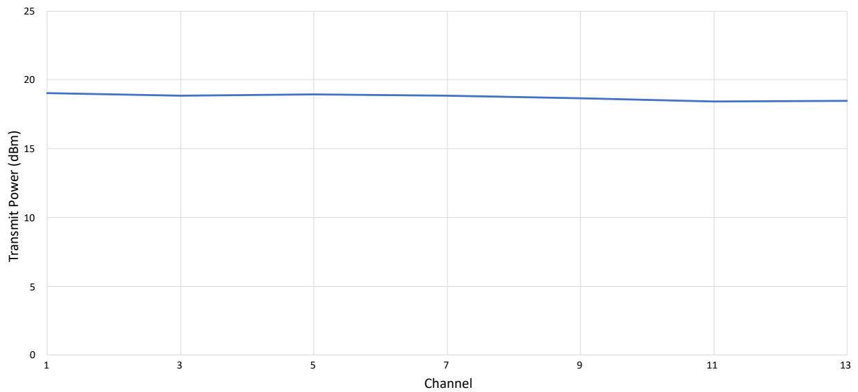
Figure 3-8. Transmit Power vs Channel, 1Mbps, 3.3V, 25°C
