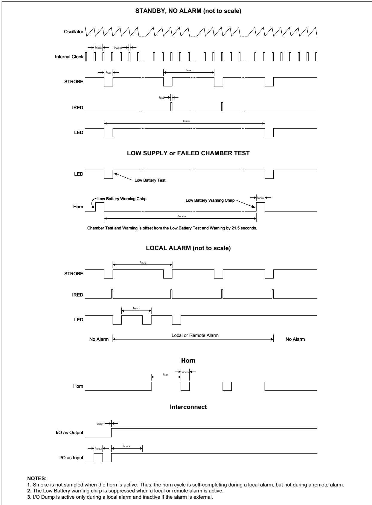
FIGURE 3-1: RE46C143 Timing Diagrams.
