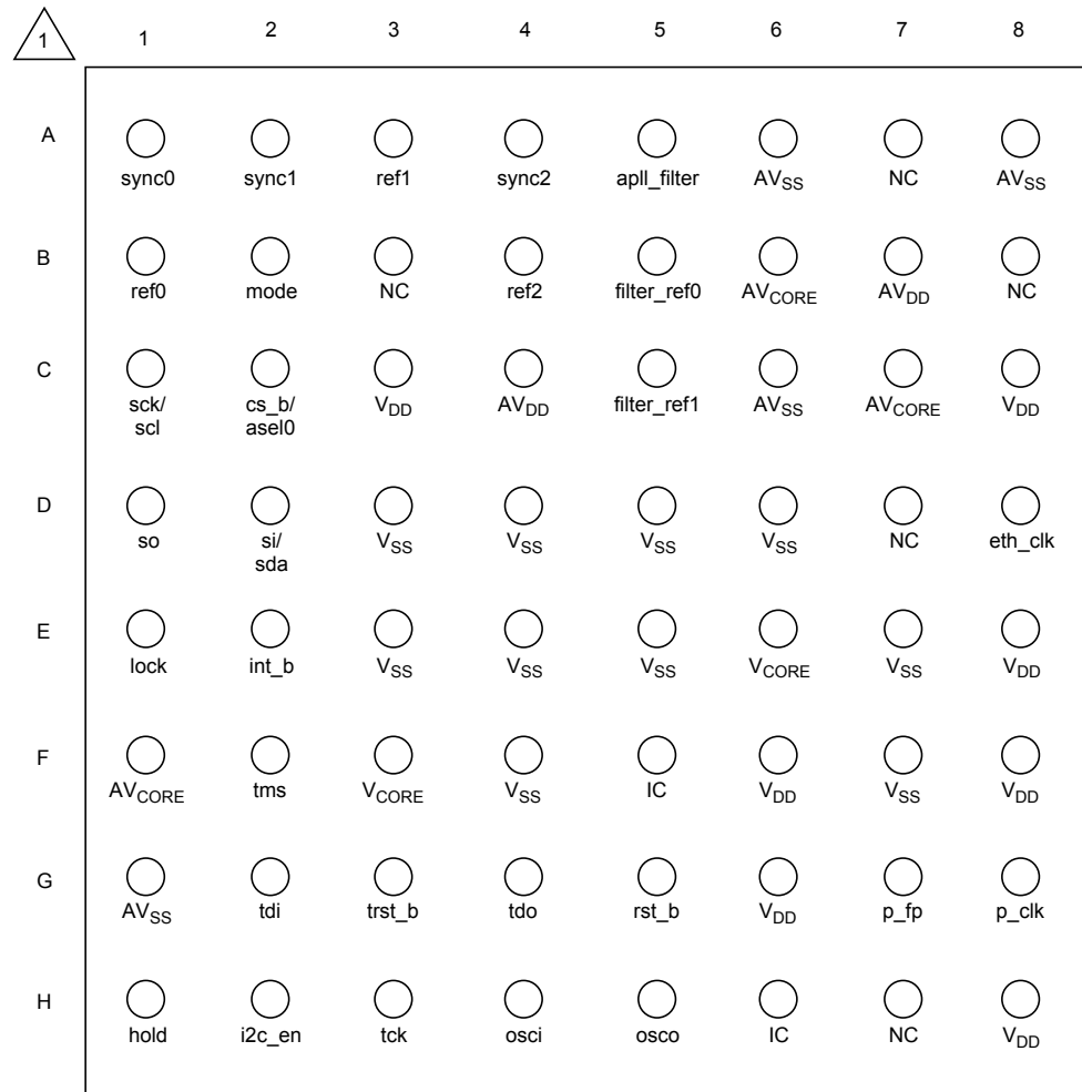
TOP VIEW
