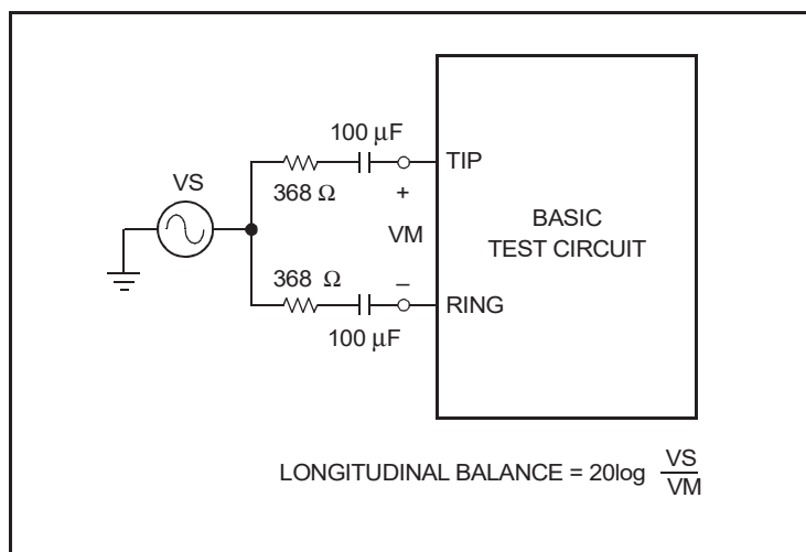
Figure 7-4. Longitudinal Balance
