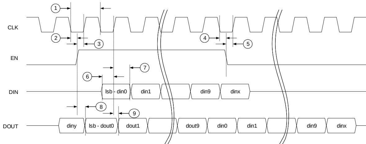
Figure 5-1. Serial Interface Timing Diagram
