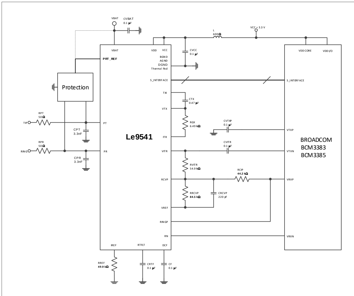
Figure 8-2. Reference Schematic Interfacing Broadcom Codec
