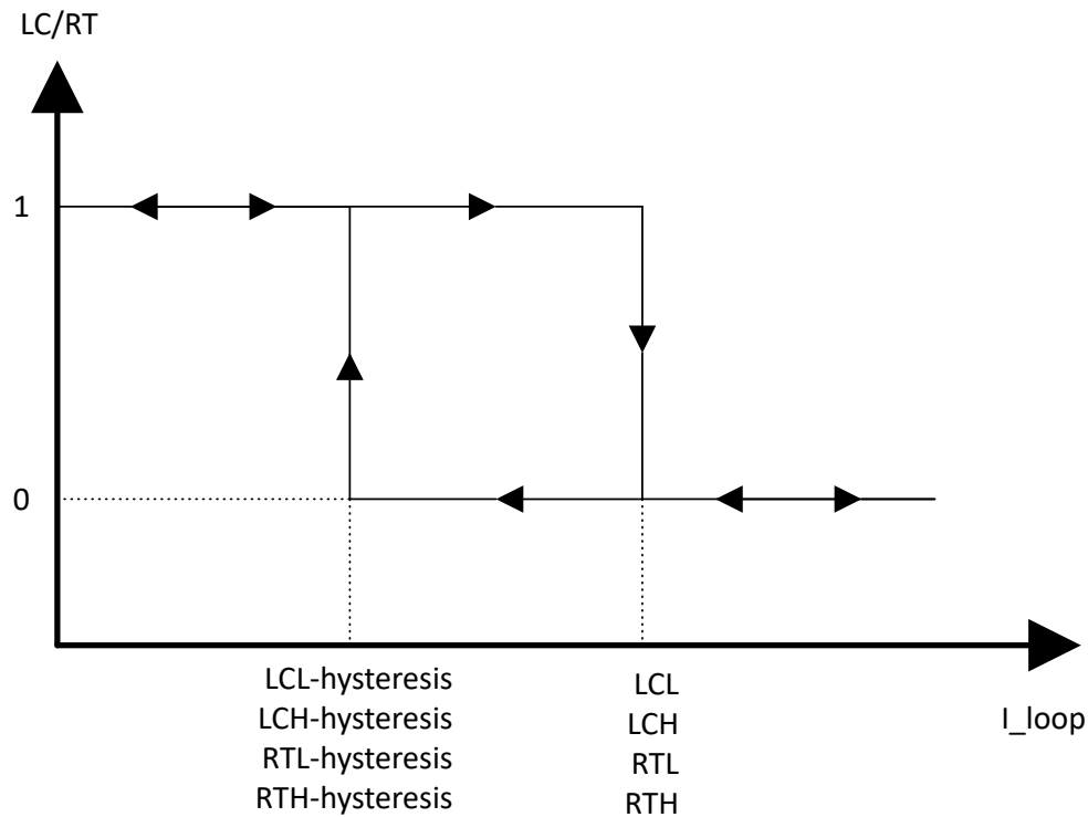
Figure 8-1. Detection Threshold with Hysteresis
