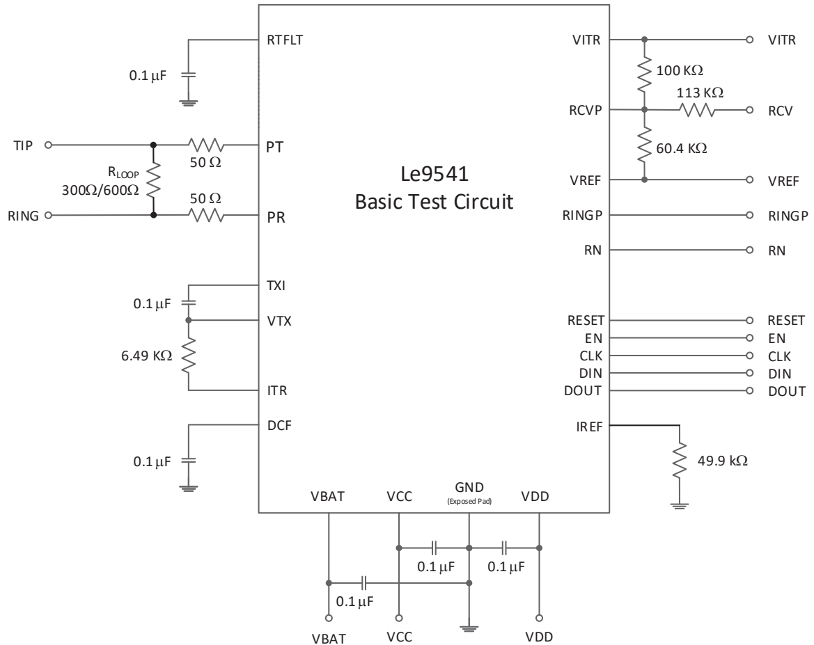
Figure 7-1. Le9541 Basic Test Circuit Diagram
