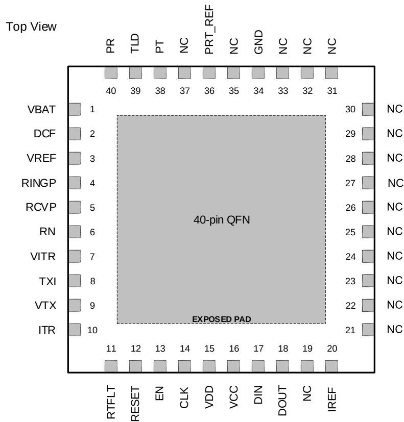
Figure 2-1. Le9541 Pin Diagram
