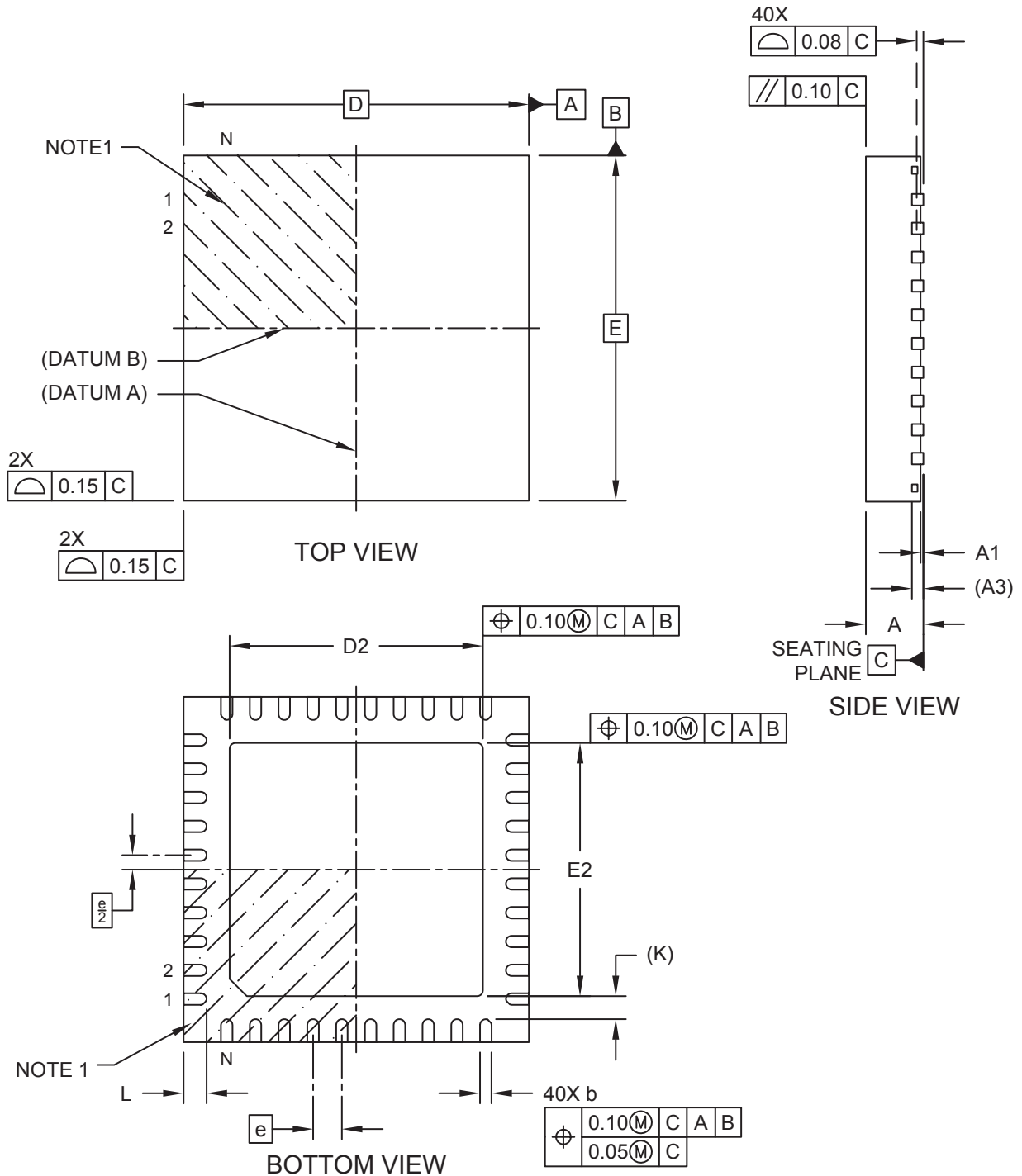
Figure 9-1. 40-Pin QFN Package Diagram
