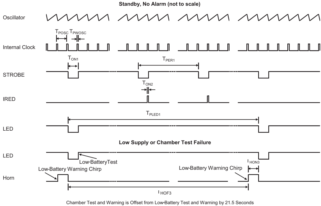
FIGURE 3-1: RE46C144 Timing Diagram – Standby, Low Supply and Chamber Test Failure.
