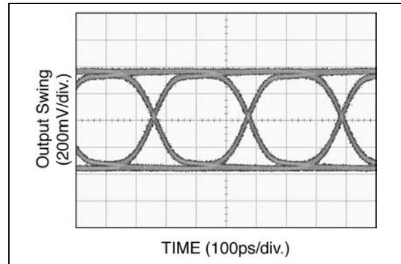
FIGURE 2-3: 20 mV PP Input @ 3.2 Gbps 2^{23}-1 PRBS.
