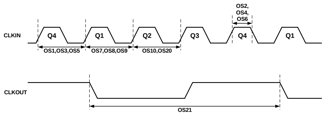
Figure 32-4. Clock Timing
