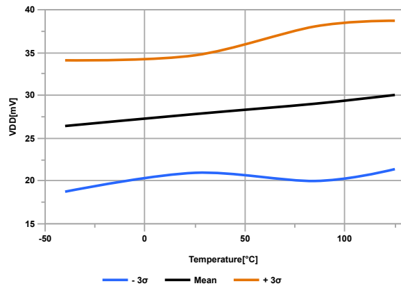
Figure 33-9. BROWN-OUT RESET HYSTERESIS, TRIP POINT (BORV = 0)
