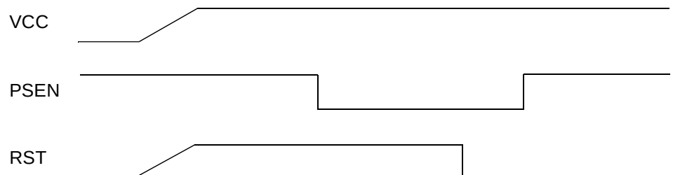
Figure 38. Hardware conditions typical sequence during power-on.
