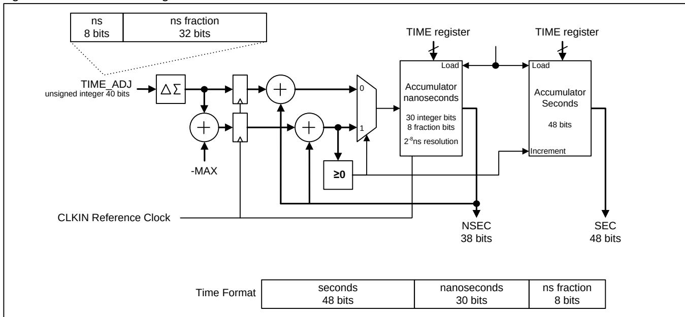
Figure 7-14. 1588 Time Engine
