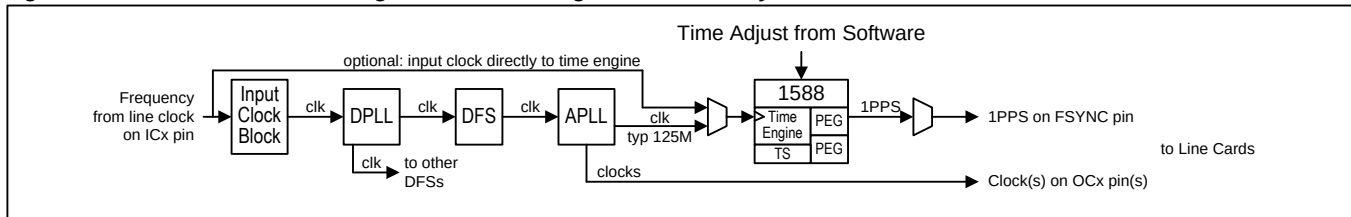
Figure 2-5. 1588 Resource Usage, Slave Timing Card, 1588-Only or 1588+SyncE
