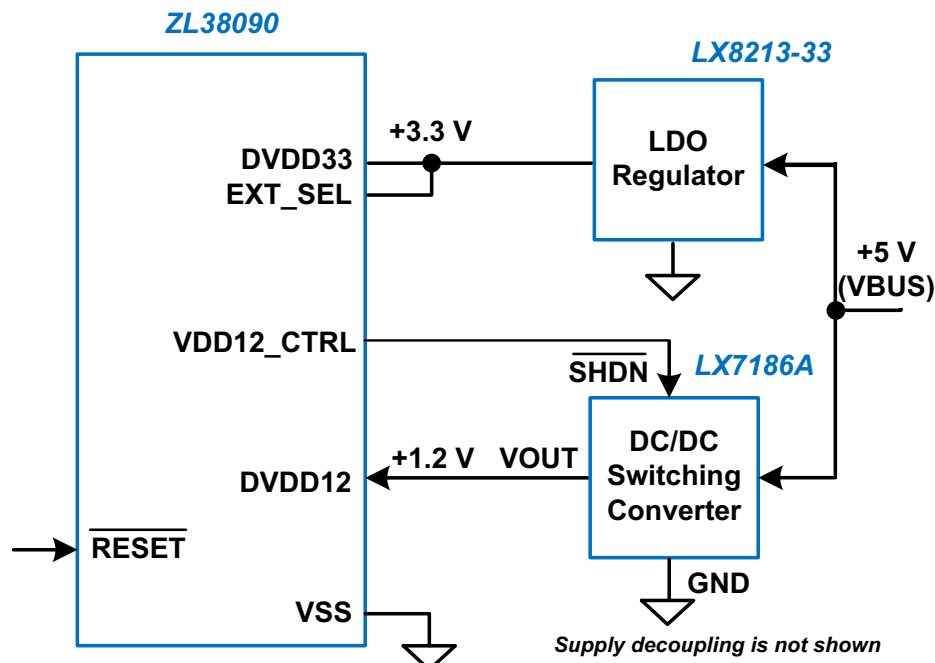
Figure 26 • Typical Power Supply Configuration
