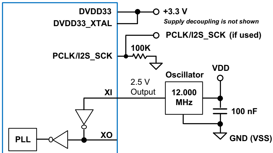
Figure 33 • Clock Oscillator Application Circuit
