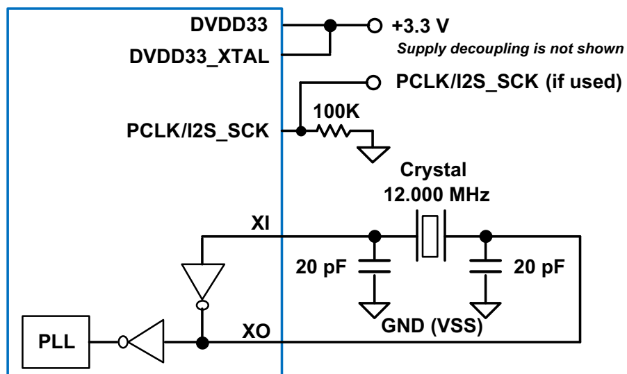
Figure 32 • Crystal Application Circuit
