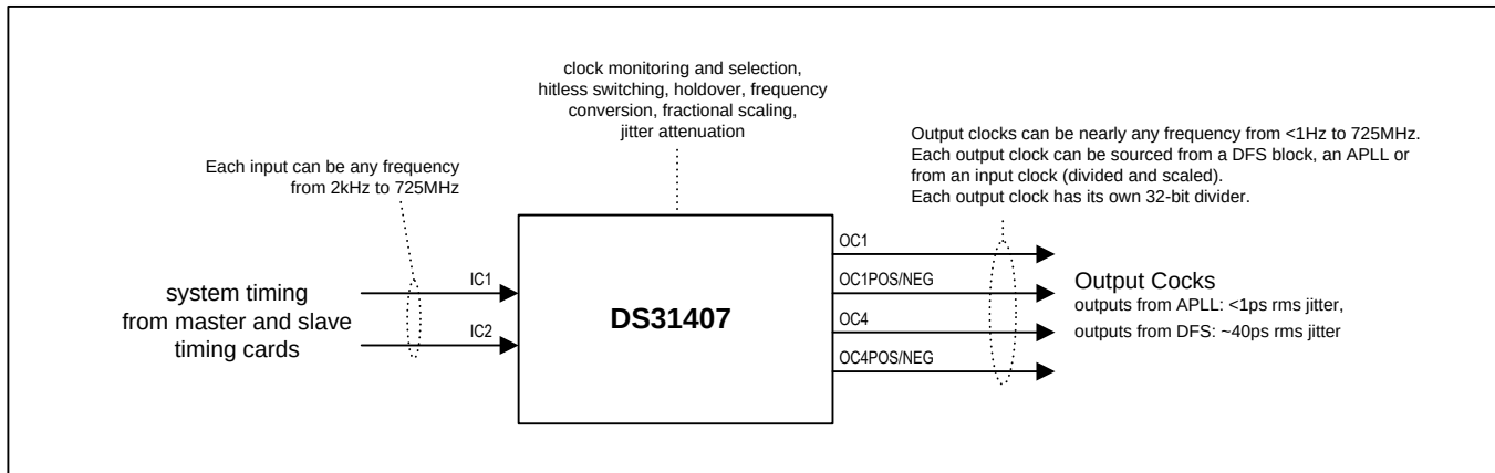
Figure 2-1. Typical Application Example
