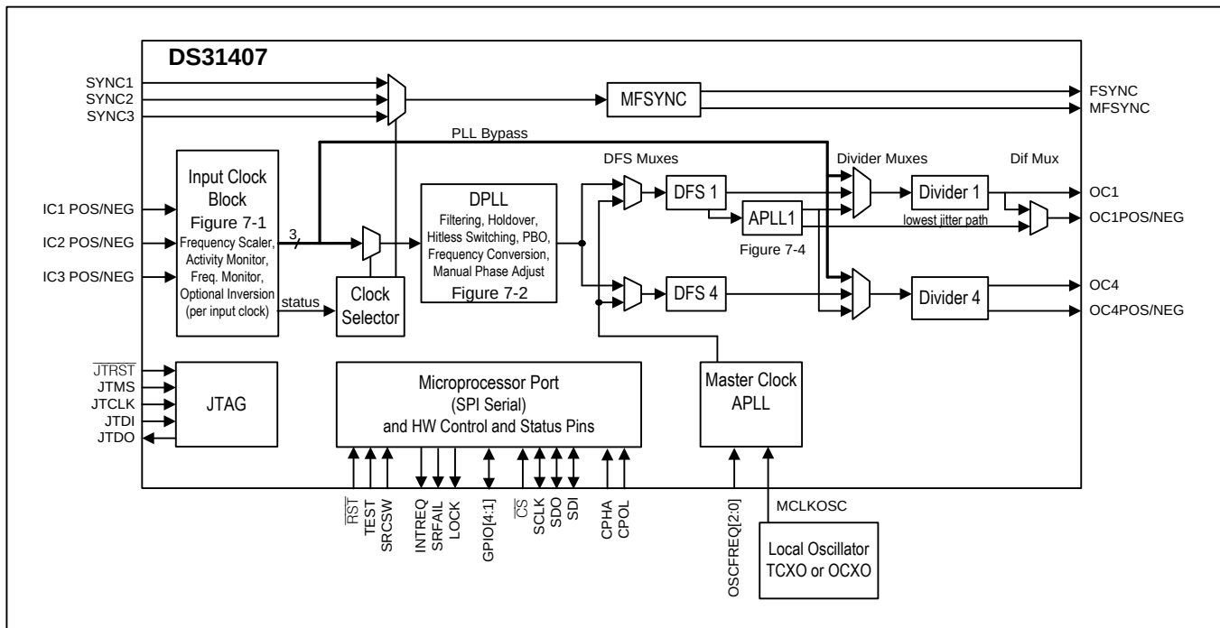
Figure 3-1. DS31407 Block Diagram
