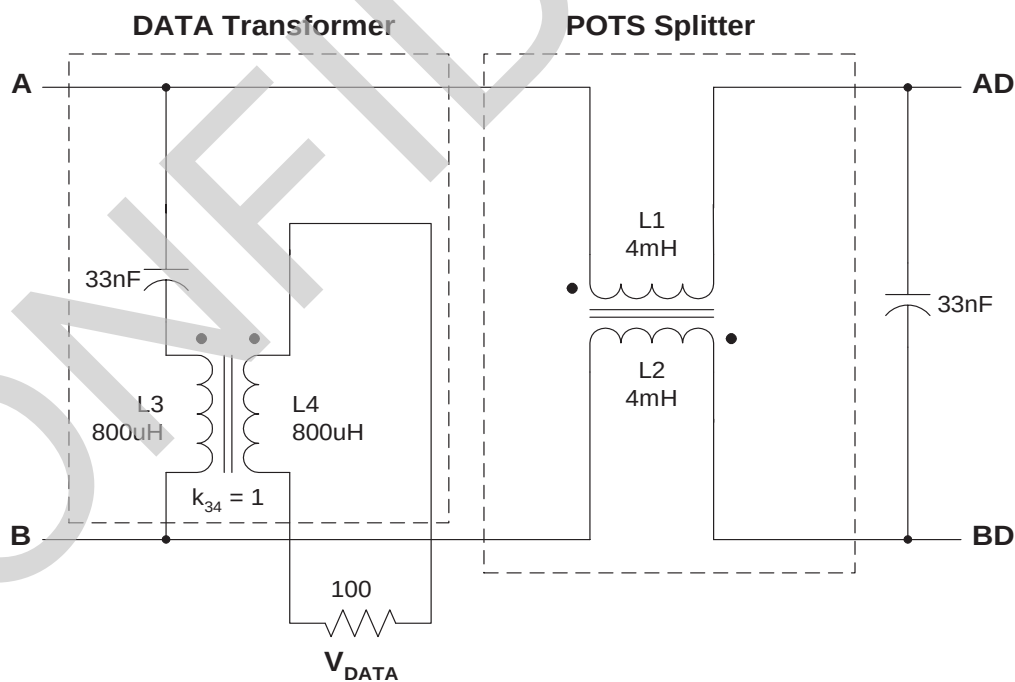
Figure 2. IVD POTS Splitter and Data Transformer
