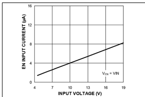
FIGURE 2-8: Enable Input Current vs. Input Voltage.
