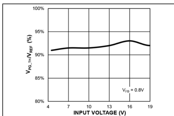
FIGURE 2-9: PG Threshold/ V_{REF} Ratio vs. Input Voltage.
