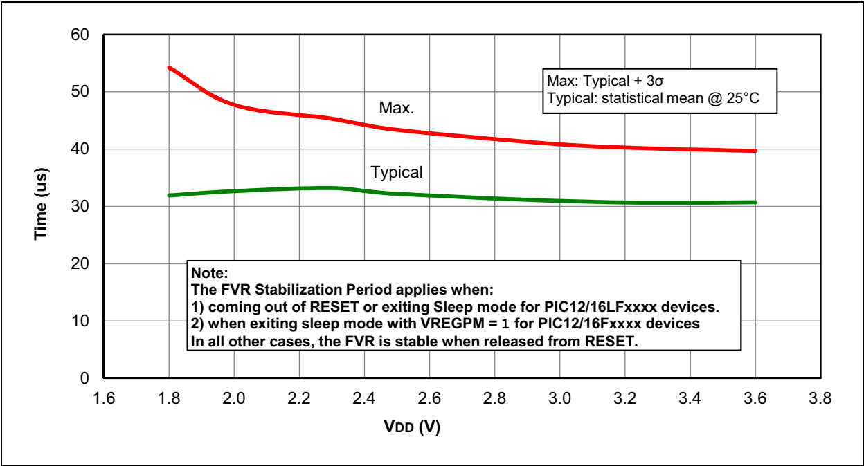
FIGURE 36-19: FVR STABILIZATION PERIOD
