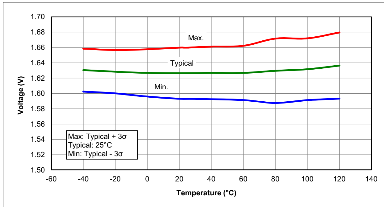
FIGURE 36-7: POR RELEASE VOLTAGE
