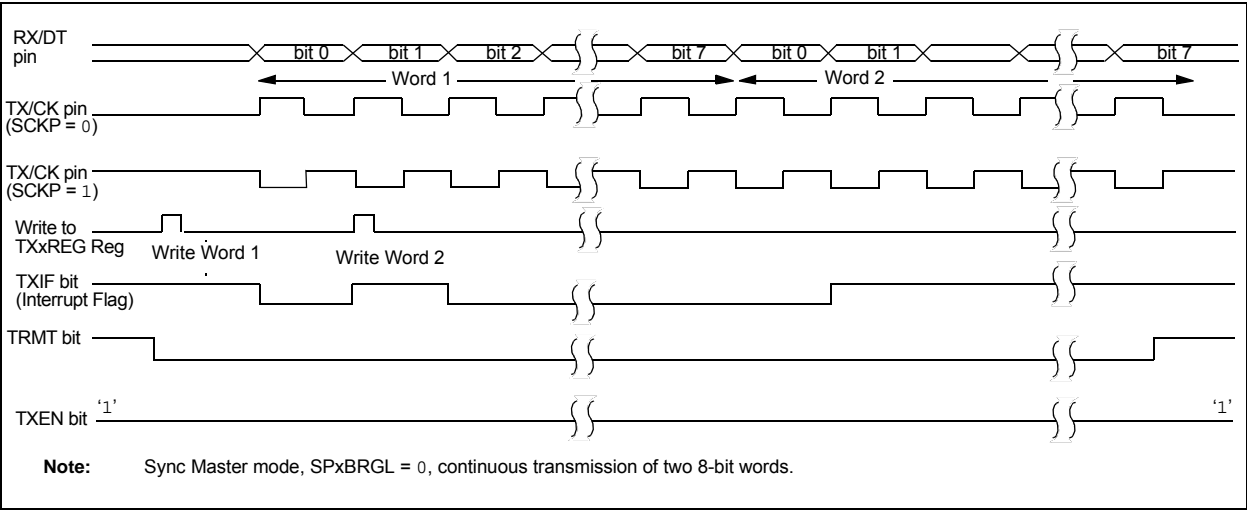
FIGURE 25-10: SYNCHRONOUS TRANSMISSION
