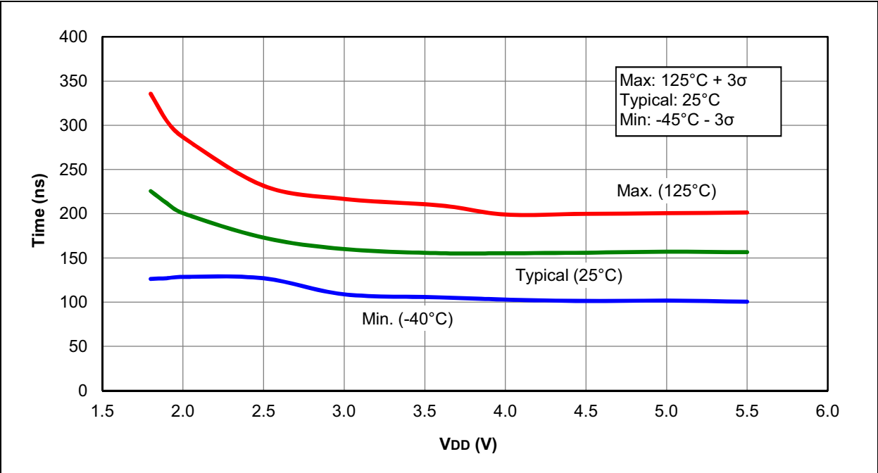
FIGURE 36-23: COMPARATOR RESPONSE TIME OVER TEMPERATURE, NORMAL-POWER MODE (CxSP = 1)
