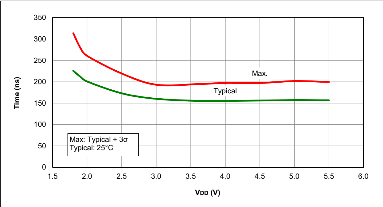
FIGURE 36-22: COMPARATOR RESPONSE TIME, NORMAL-POWER MODE (CxSP = 1)
