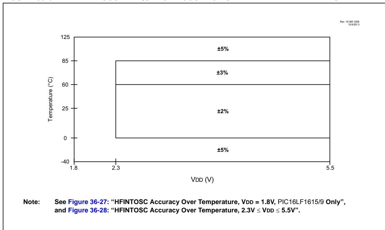
FIGURE 35-6: HFINTOSC FREQUENCY ACCURACY OVER V DD AND TEMPERATURE
