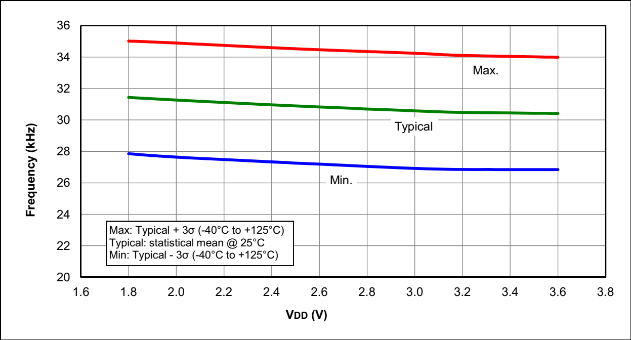
FIGURE 36-25: LFINTOSC FREQUENCY OVER VDD AND TEMPERATURE, PIC16LF1615/9 ONLY
