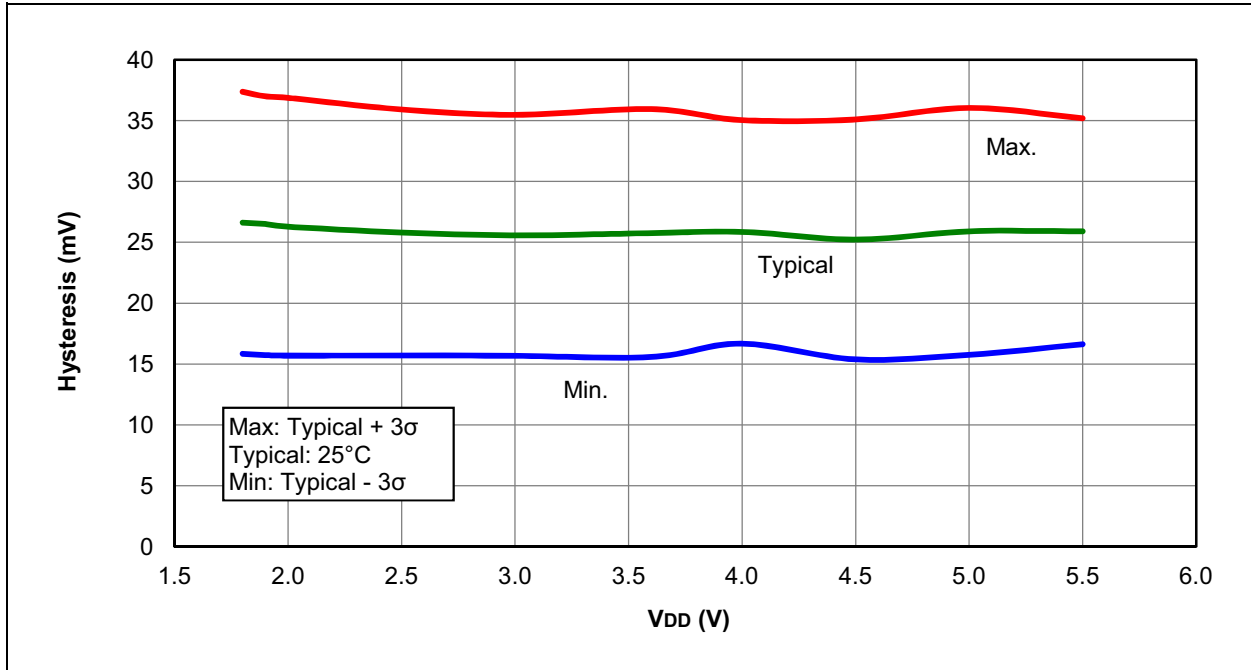
FIGURE 36-20: COMPARATOR HYSTERESIS, NORMAL-POWER MODE (CxSP = 1, CxHYS = 1)
