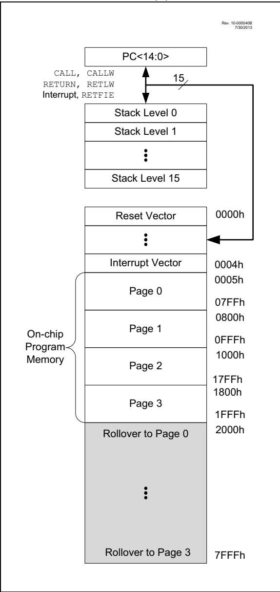
FIGURE 3-1: PROGRAM MEMORY MAP AND STACK FOR PIC16(L)F1615/9
