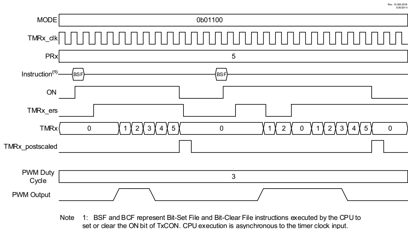
FIGURE 23-10: EDGE-TRIGGERED HARDWARE LIMIT ONE-SHOT TIMING DIAGRAM
