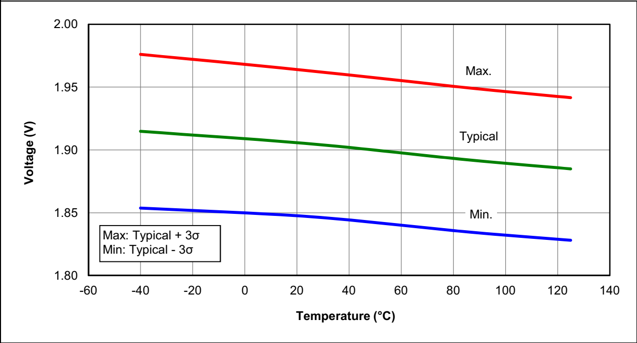
FIGURE 36-9: BROWN-OUT RESET VOLTAGE, BORV = 1, PIC16LF1615/9 ONLY
