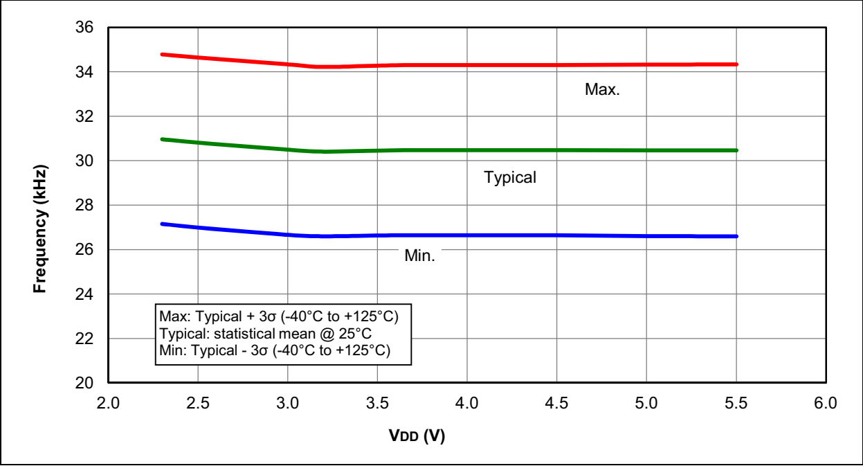
FIGURE 36-26: LFINTOSC FREQUENCY OVER VDD AND TEMPERATURE, PIC16F1615/9 ONLY
