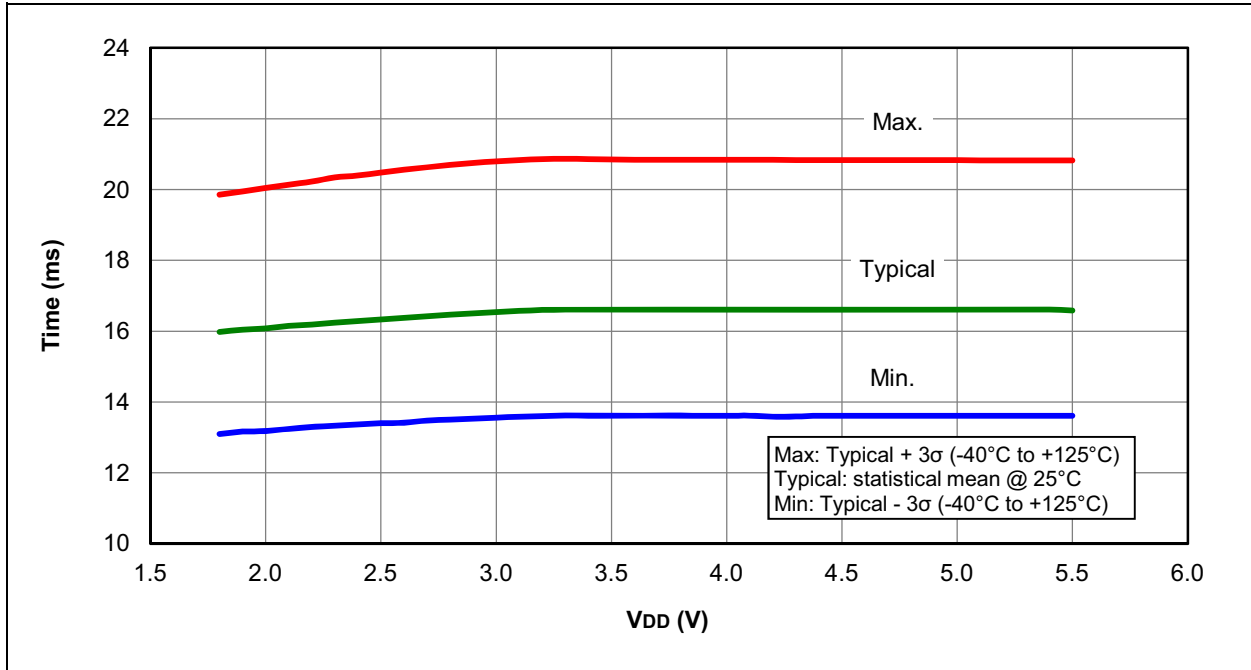
FIGURE 36-17: WDT TIME-OUT PERIOD
