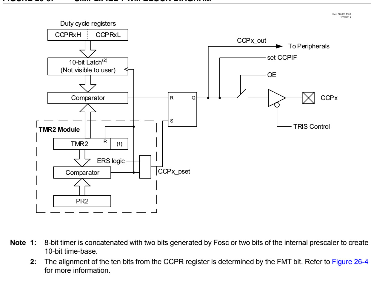
FIGURE 26-3: SIMPLIFIED PWM BLOCK DIAGRAM
