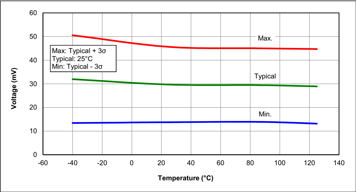
FIGURE 36-10: BROWN-OUT RESET HYSTERESIS, BORV = 1, PIC16LF1615/9 ONLY
