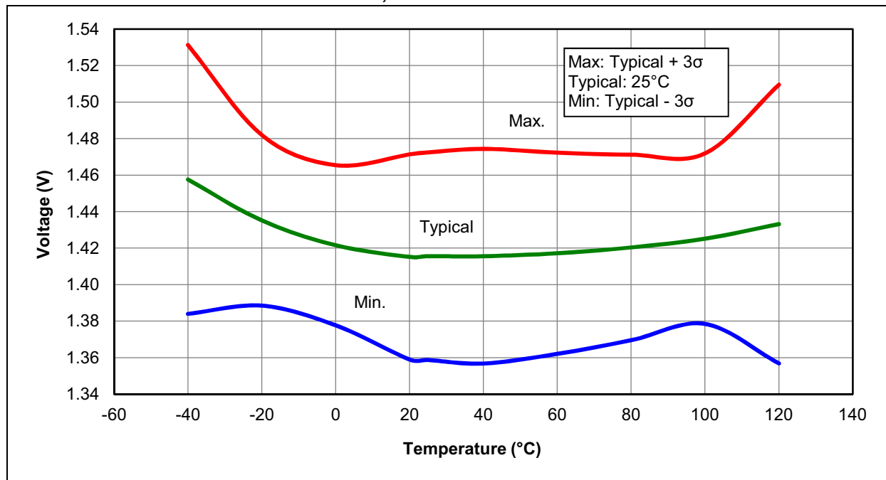
FIGURE 36-8: POR REARM VOLTAGE, PIC16F1615/9 ONLY
