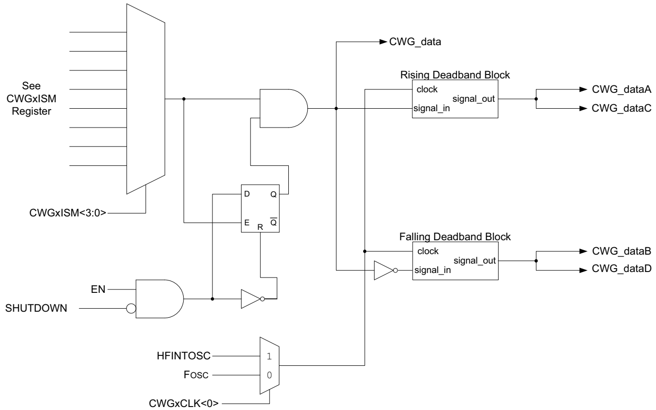
FIGURE 28-1: SIMPLIFIED CWG BLOCK DIAGRAM (HALF-BRIDGE MODE)
