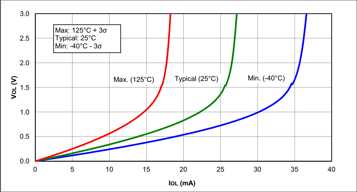
FIGURE 36-4: V_{OL} vs. I_{OL} OVER TEMPERATURE, V_{DD} = 3.0V
