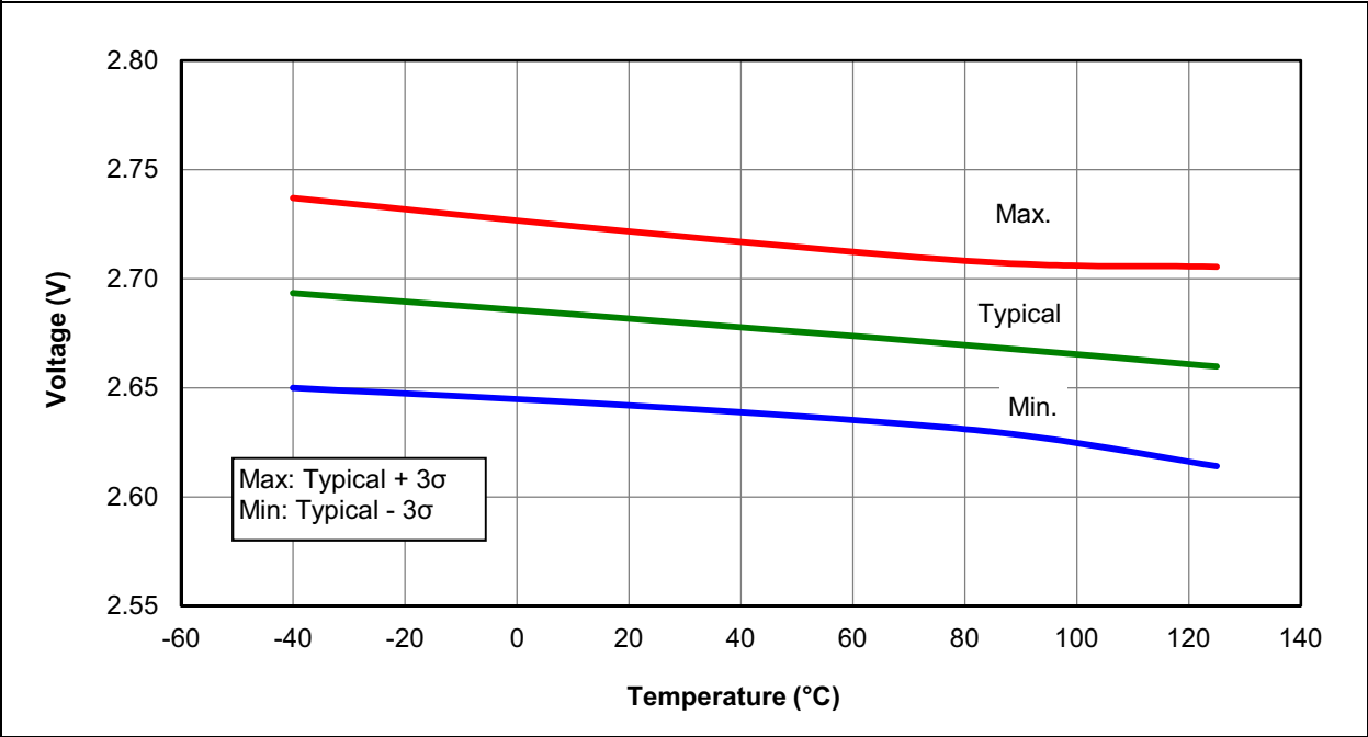
FIGURE 36-13: BROWN-OUT RESET VOLTAGE, BORV = 0
