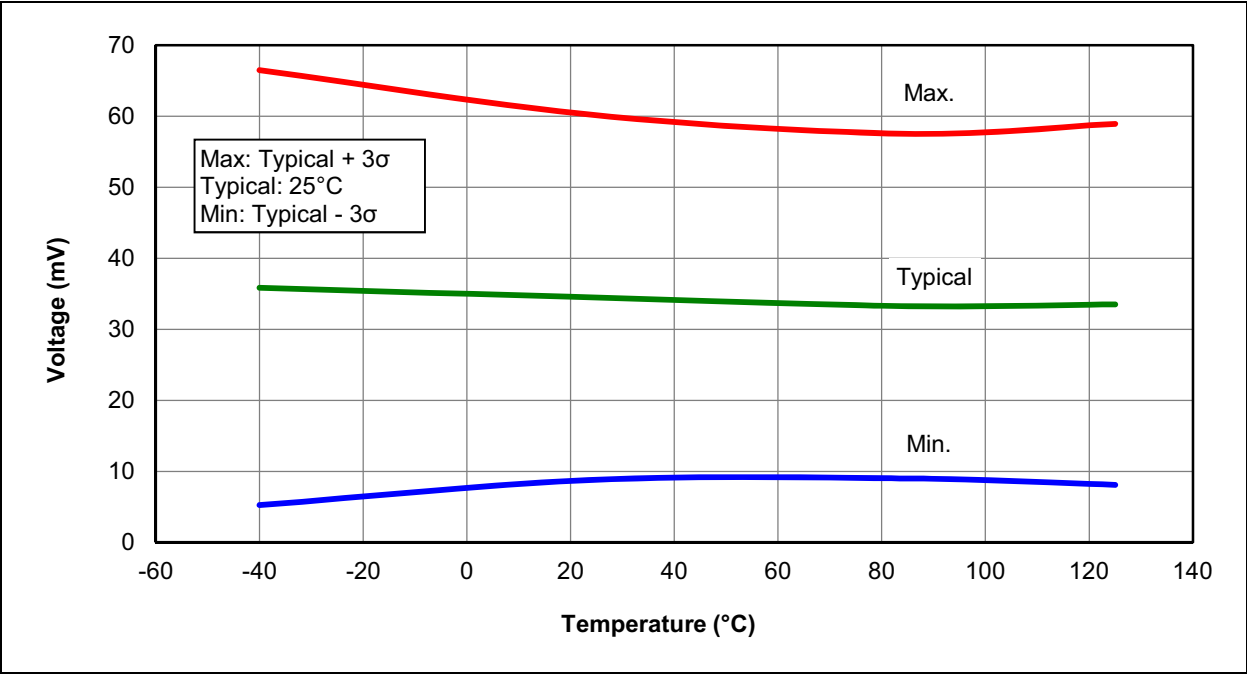
FIGURE 36-12: BROWN-OUT RESET HYSTERESIS, BORV = 1, PIC16F1615/9 ONLY
