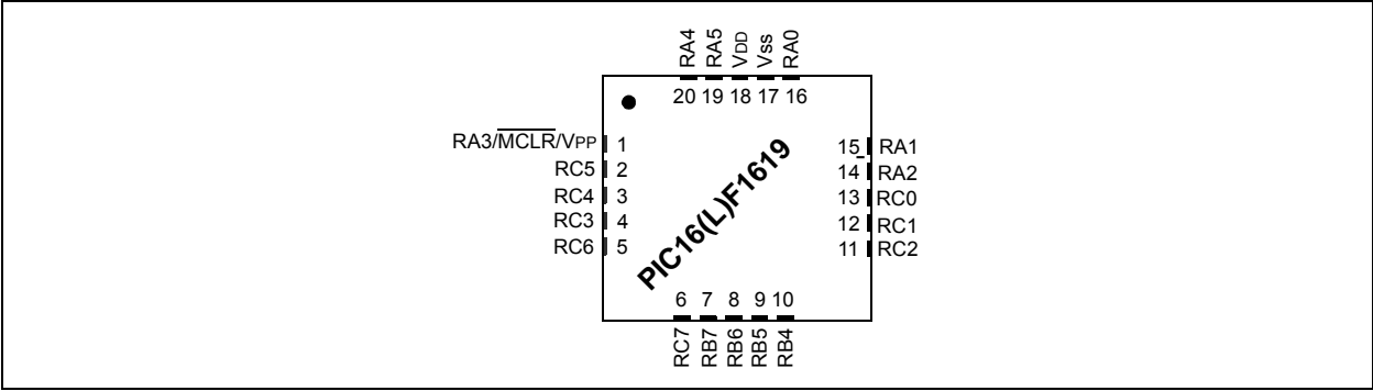
FIGURE 4: 20-PIN UQFN, QFN
