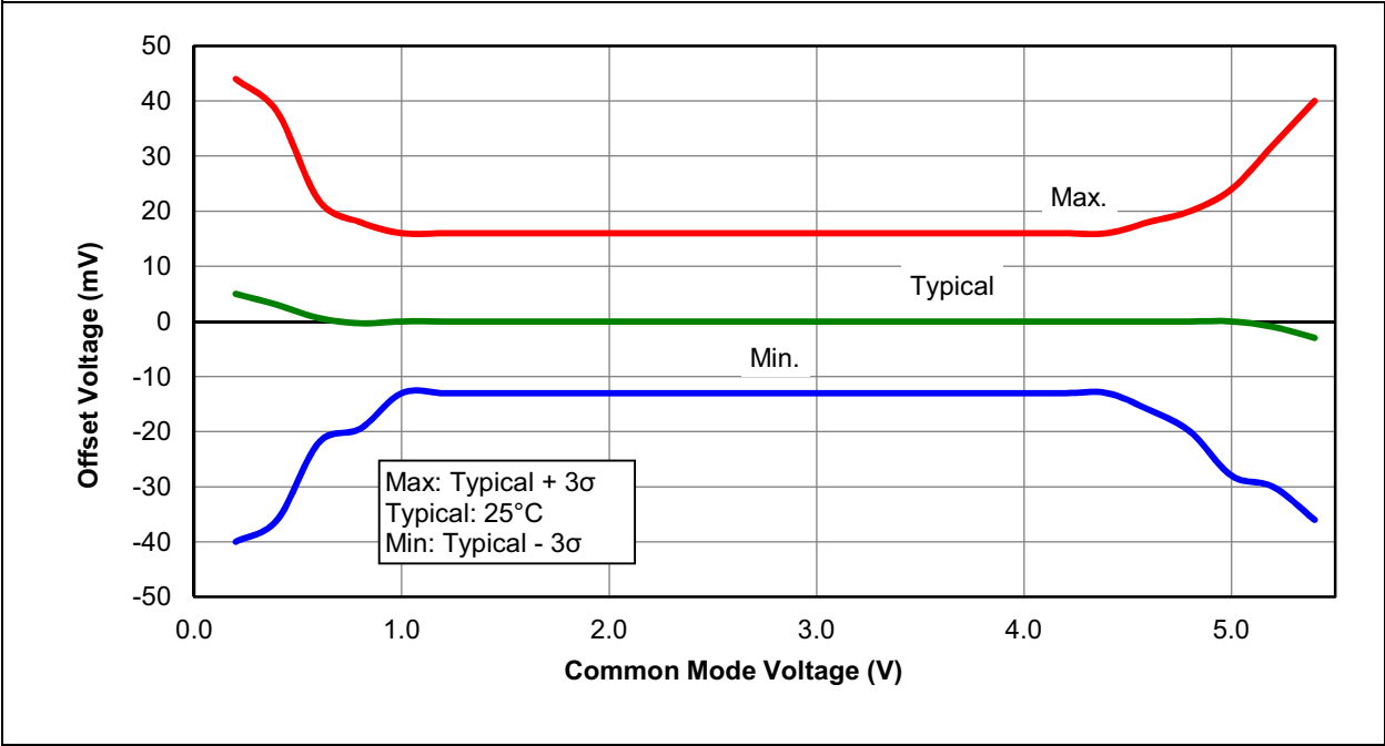
FIGURE 36-24: COMPARATOR INPUT OFFSET AT 25°C, NORMAL-POWER MODE (CxSP = 1), PIC16F1615/9 ONLY
