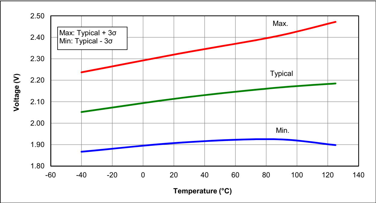
FIGURE 36-15: LOW-POWER BROWN-OUT RESET VOLTAGE, LPBOR = 0
