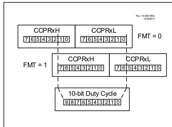
FIGURE 26-4: CCPx DUTY-CYCLE ALIGNMENT
