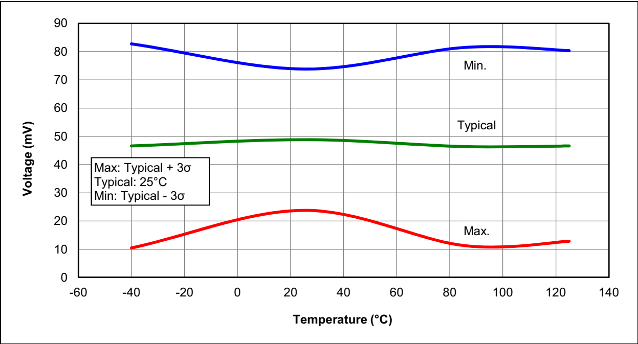
FIGURE 36-14: BROWN-OUT RESET HYSTERESIS, BORV = 0
