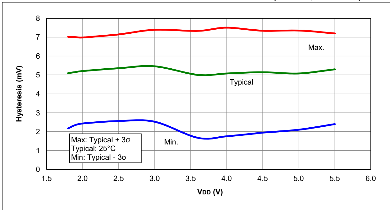
FIGURE 36-21: COMPARATOR HYSTERESIS, LOW-POWER MODE (CxSP = 0, CxHYS = 1)
