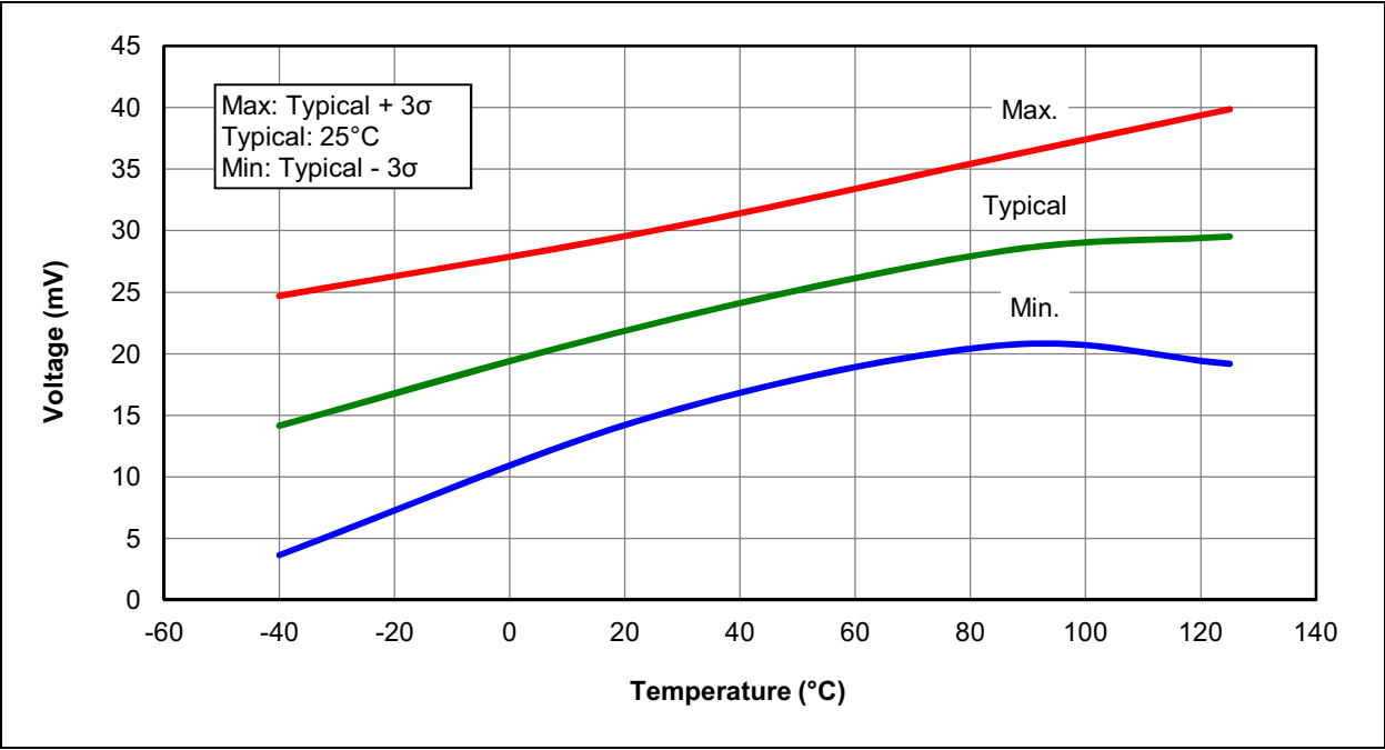
FIGURE 36-16: LOW-POWER BROWN-OUT RESET HYSTERESIS, LPBOR = 0
