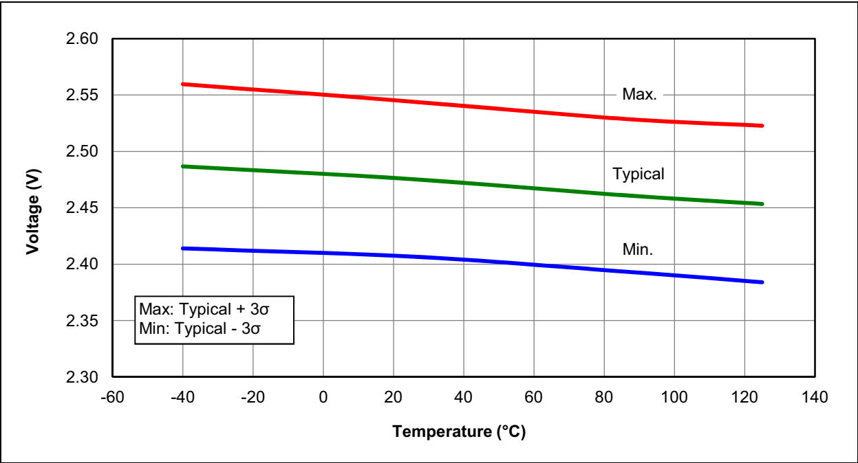
FIGURE 36-11: BROWN-OUT RESET VOLTAGE, BORV = 1, PIC16F1615/9 ONLY
