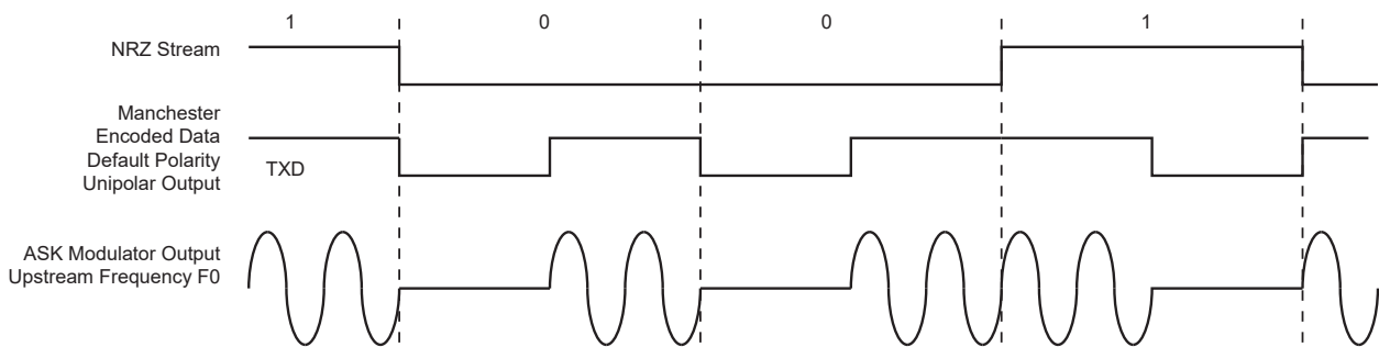
Figure 46-17. ASK Modulator Output
