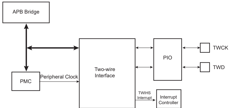
Figure 43-1. Block Diagram
