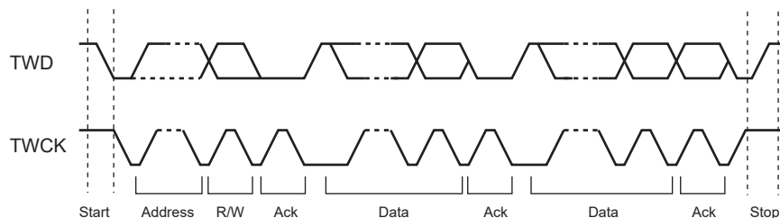
Figure 43-3. Transfer Format
