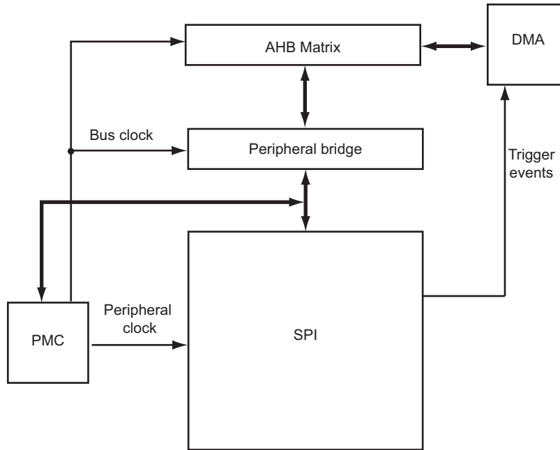
Figure 41-1. Block Diagram
