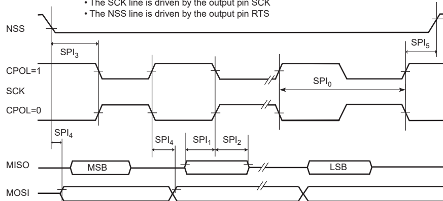
Figure 58-26. USART SPI Host Mode
