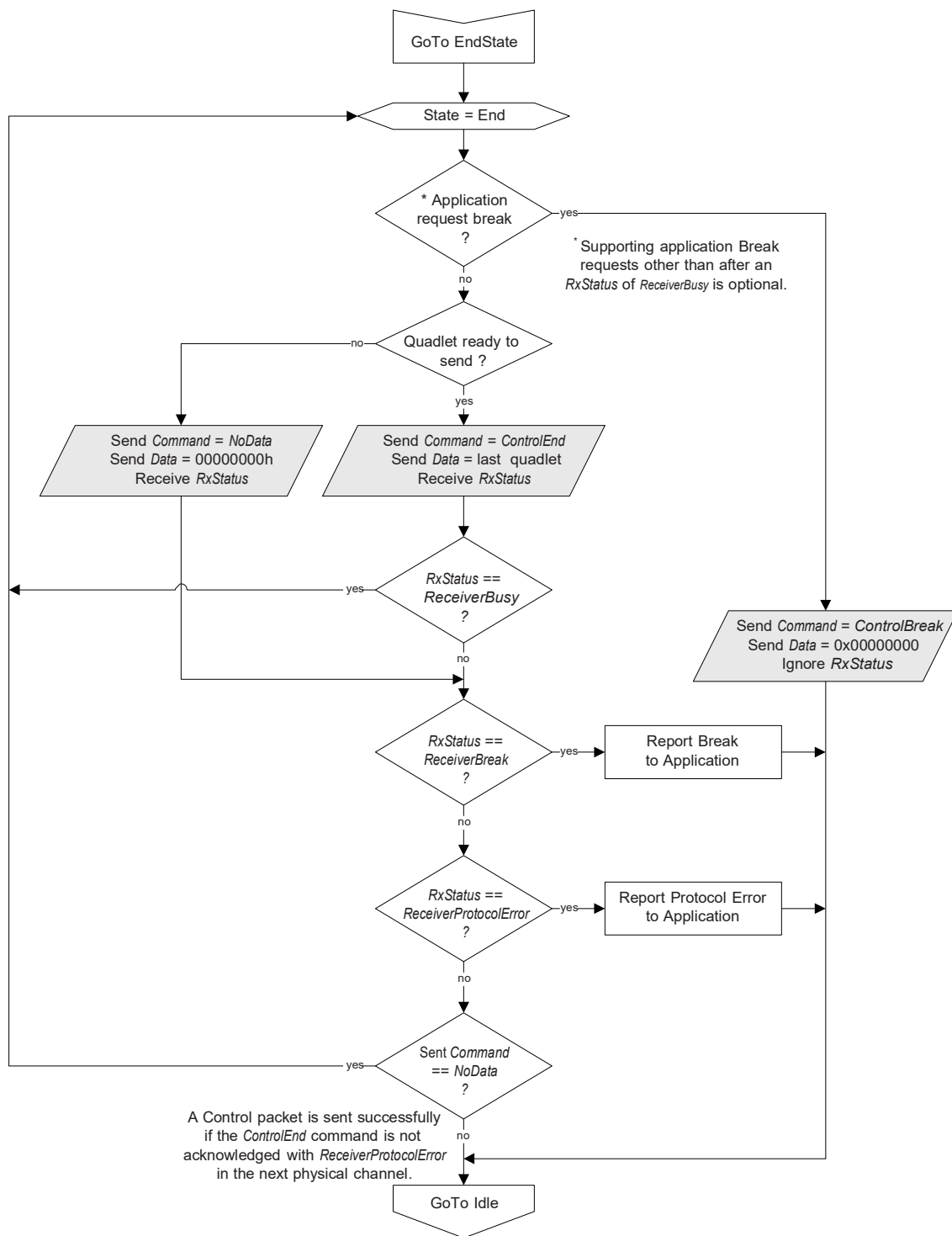
Figure 48-8. Control Packet Tx Device Protocol: End
