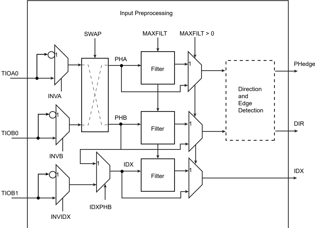
Figure 50-18. Input Stage
