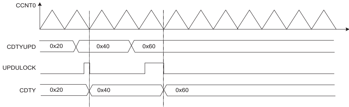
Figure 51-19. Method 1 (UPDM = 0)
