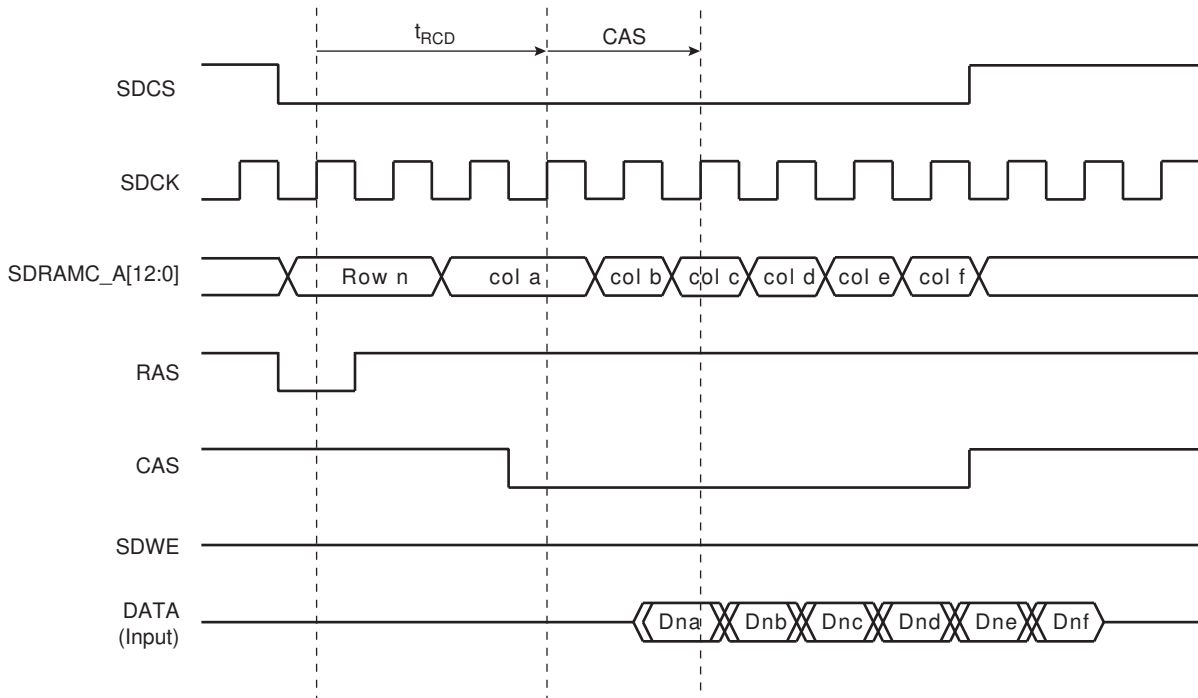
Figure 34-3. Read Burst SDRAM Access
