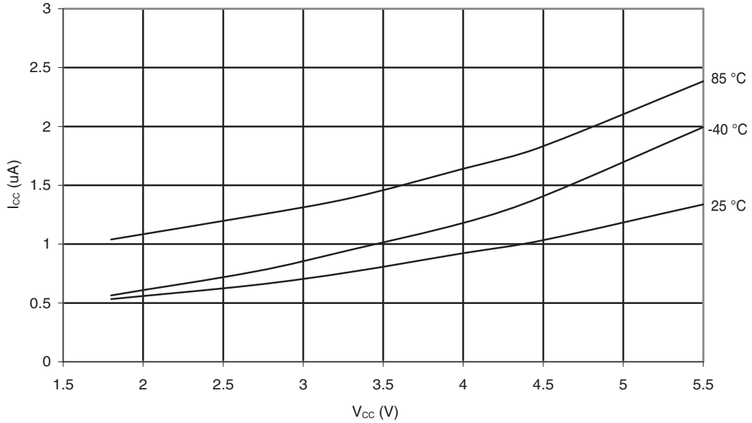
Figure 31-107. ATmega88A: Power-Save Supply Current vs. V_{CC} (Watchdog Timer Disabled and 32kHz Crystal Oscillator Running)
