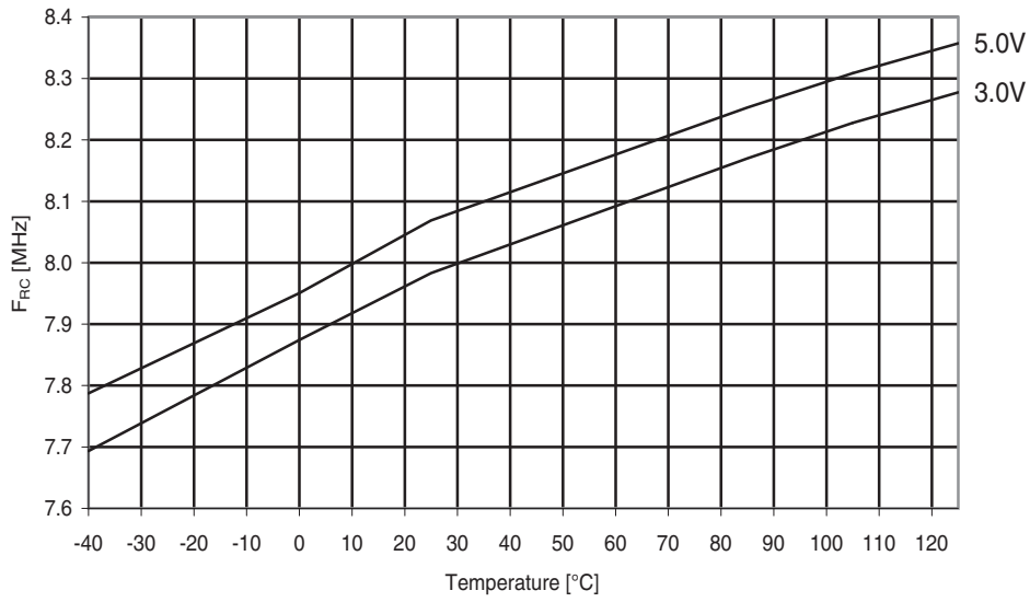
Figure 30-284. ATmega644PA: Calibrated 8MHz RC oscillator vs. temperature
