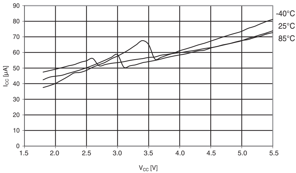
Figure 30-189. ATmega324PA: Analog comparator current vs. V_{CC}
