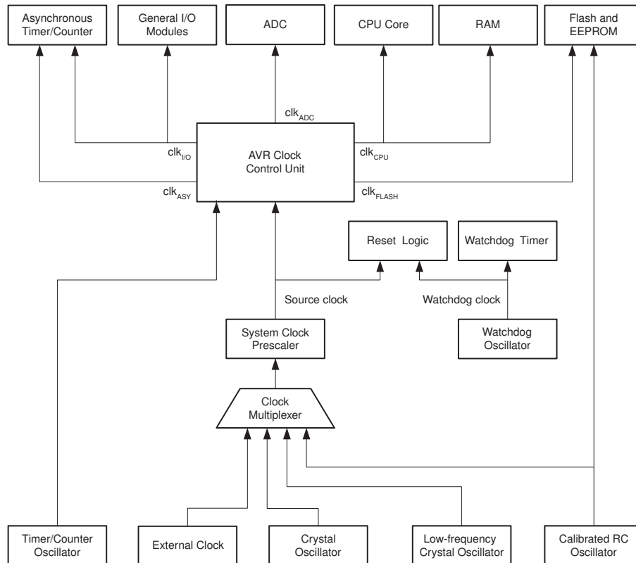
Figure 9-1. Clock distribution.
