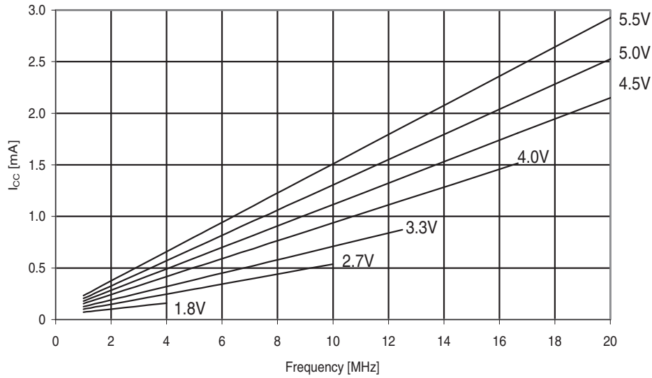
Figure 30-203. ATmega644A: Idle supply current vs. V_{CC} (1 - 20MHz)
