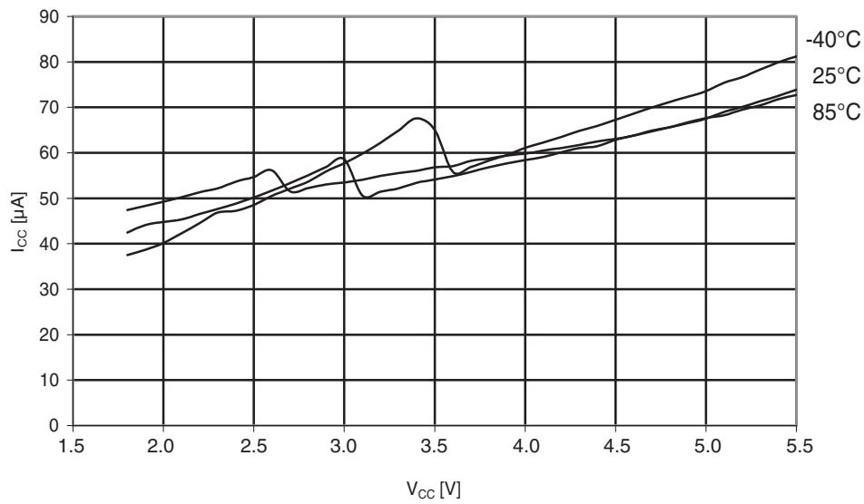
Figure 30-140. ATmega324A: Analog comparator current vs. V_{CC}
