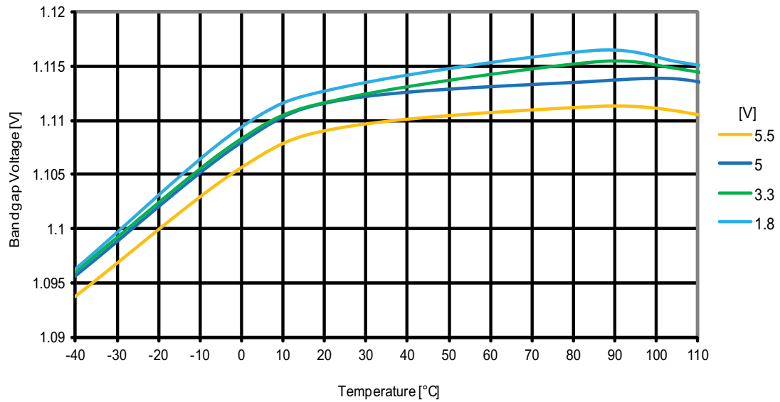
Figure 31-150. ATmega1284P: Bandgap voltage vs. temperature
