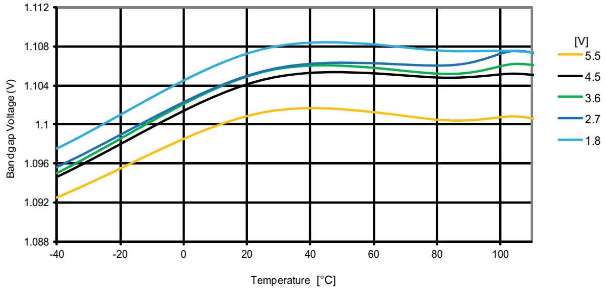
Figure 31-29. ATmega164PA: Bandgap voltage vs. temperature
