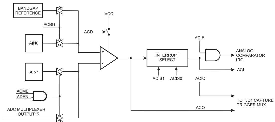
Figure 22-1. Analog Comparator block diagram (2)
