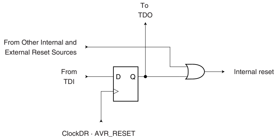
Figure 25-2. Reset register
