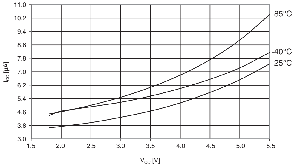
Figure 30-356. ATmega1284P: Power-down supply current vs. V_{CC} (watchdog timer enabled)
