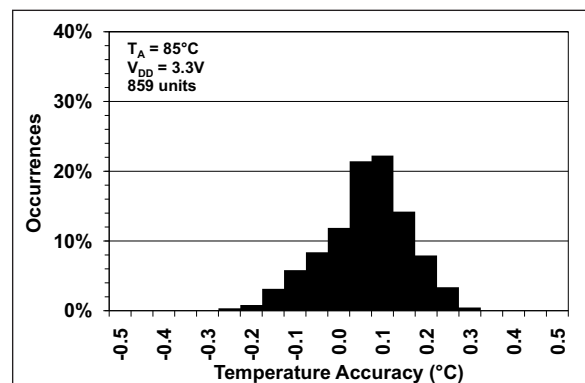
FIGURE 2-5: Temperature Accuracy Histogram, T_A = +85^{\circ}C .
